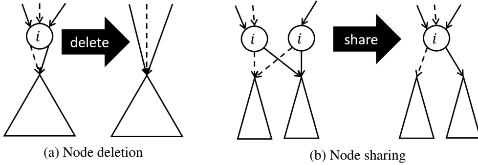
Figure 2.4. Reduction rules of the BDD
