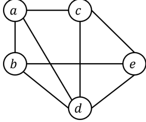
(a) An undirected graph
