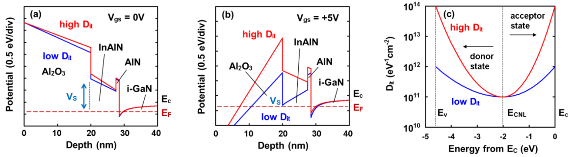
Fig. 6-4. Potential profile of Al 2 O 3 /InAlN/GaN structures at (a) V_{gs} = 0 V and (b) V_{gs} = +5 V. (c) Interface state density distributions used in calculation (Reproduced from ref. 22, copyright 2017 by the Japan Society of Applied Physics).
