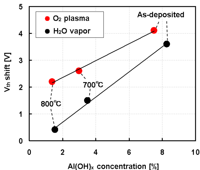
Fig. 4-6. \text{Al(OH)}_x concentration dependence on V_{th} shift for \text{H}_2\text{O} vapor and \text{O}_2 plasma- \text{Al}_2\text{O}_3 . PDA temperature was varied (Reproduced from ref. 18, with the permission of CS-MANTECH).
