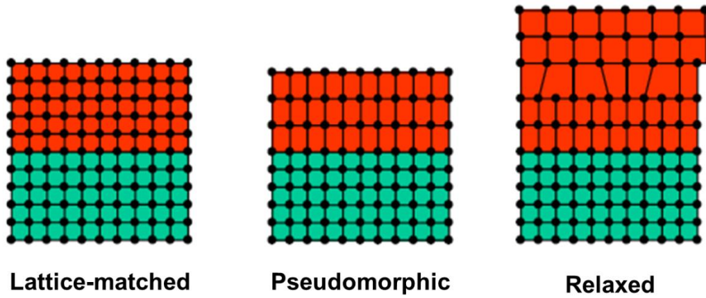
Fig. 2-4. Schematic illustrations for types of heteroepitaxial growth.
