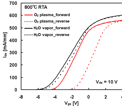
Fig. 4-10. I_{ds}-V_{gs} curves for AlGaIn/GaN MOS-HEMTs using H 2 O vapor and O 2 plasma-Al 2 O 3 for gate insulator films. 800°C PDA was applied in this figure case (Reproduced from ref. 18, with the permission of CS-MANTECH).
