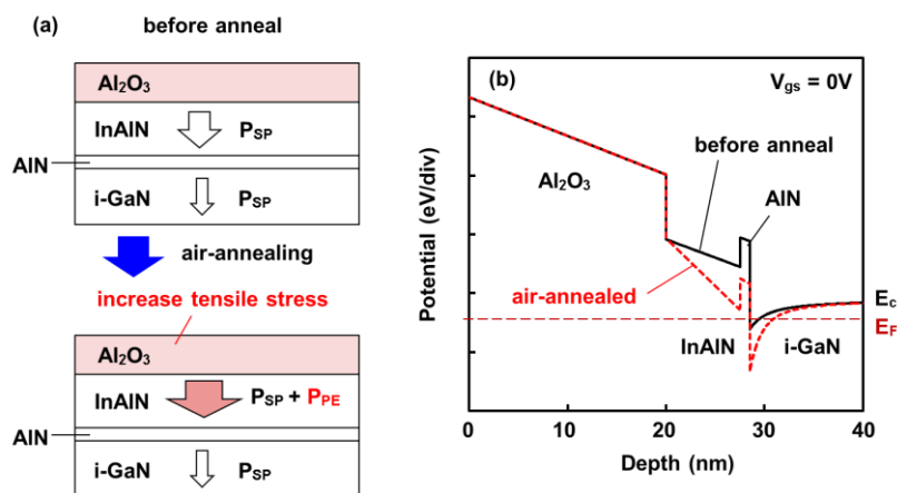
Fig. 6-6. (a) Polarization vectors and (b) schematic energy band diagrams of \text{Al}_2\text{O}_3/\text{InAlN}/\text{GaN} structures obtained before and after air-annealing (Reproduced from ref. 22, copyright 2017 by the Japan Society of Applied Physics).
