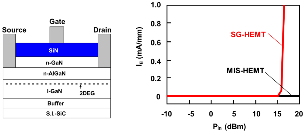
Fig. 1-11. Reduction in gate leakage current of AlGaIn/GaN HEMTs using SiN-based insulated-gate structures. 16)
