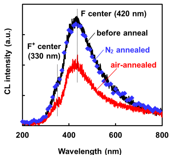
Fig. 6-5. Cathodeluminescence of ALD- \text{Al}_2\text{O}_3 before and after annealing (Reproduced from ref. 22, copyright 2017 by the Japan Society of Applied Physics).
