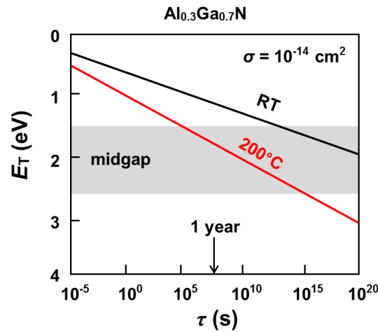
Fig. 3-7. Emission time constant \tau at \text{Al}_{0.3}\text{Ga}_{0.7}\text{N} bandgap as function of trap energy E_T , which is based on the Shockley-Read-Hall static model. 20)
