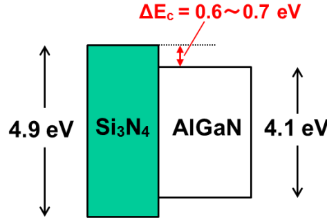
Fig. 1-12. Band offsets between Si 3 N 4 and AlGaN.
