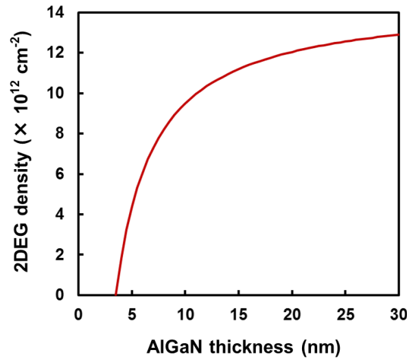
Fig. 2-9. Relationship between the 2DEG density and the thickness of AlGaIn with the Al composition ratio of 34%. 5)
