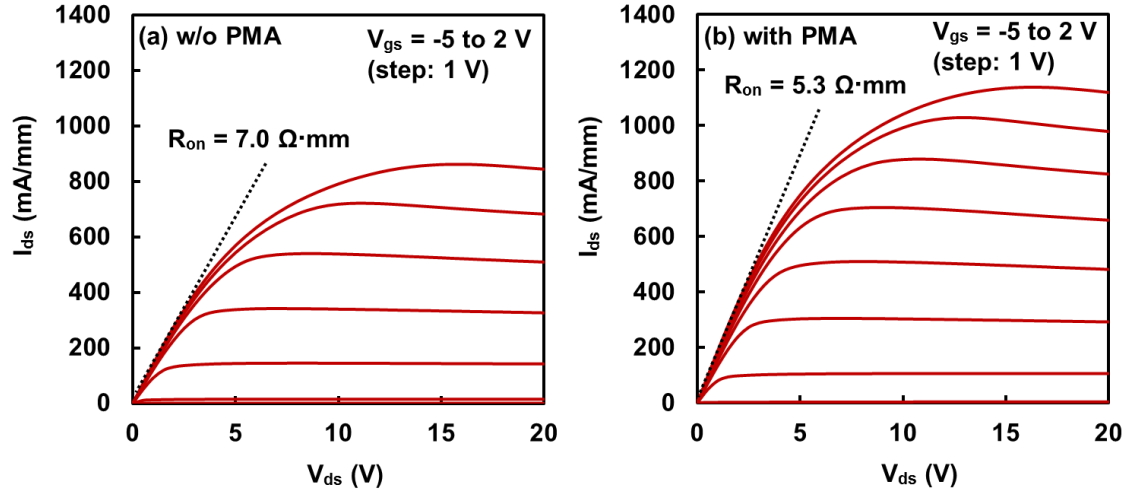
Fig. 6-2. I_{ds} - V_{ds} characteristics of InAlN/GaN MOS-HEMTs (a) without and (b) with PMA (Reproduced from ref. 22, copyright 2017 by the Japan Society of Applied Physics).
