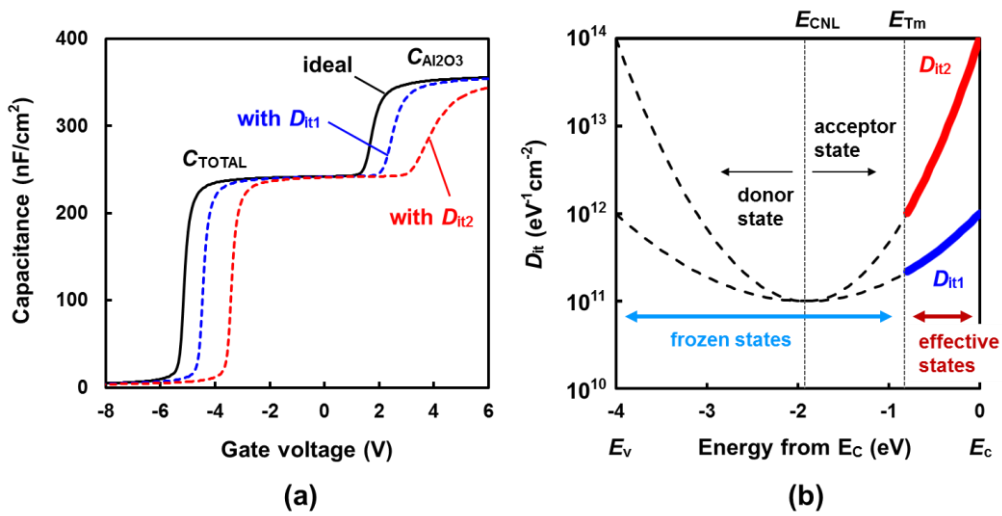
Fig. 3-6. (a) Calculated C – V characteristics of \text{Al}_2\text{O}_3/\text{AlGaIn}/\text{GaN} structures. (b) \text{Al}_2\text{O}_3/\text{AlGaIn} interface density distributions assumed in calculation.
