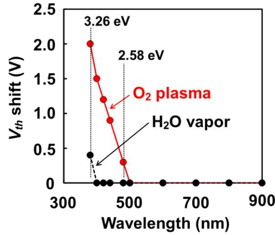
Fig. 4-12. Relationship between wavelength and V_{th} shift of AlGaIn/GaN MOS-HEMT measured by photo-assisted C - V measurement (Reproduced from ref. 10, copyright 2013 by the Japan Society of Applied Physics).
