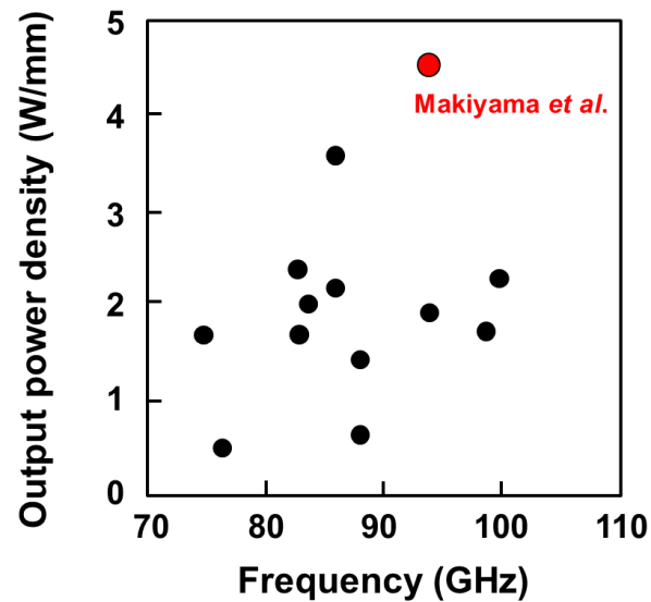
Fig. 1-10. Comparison in performance of GaN HEMT power amplifiers.
