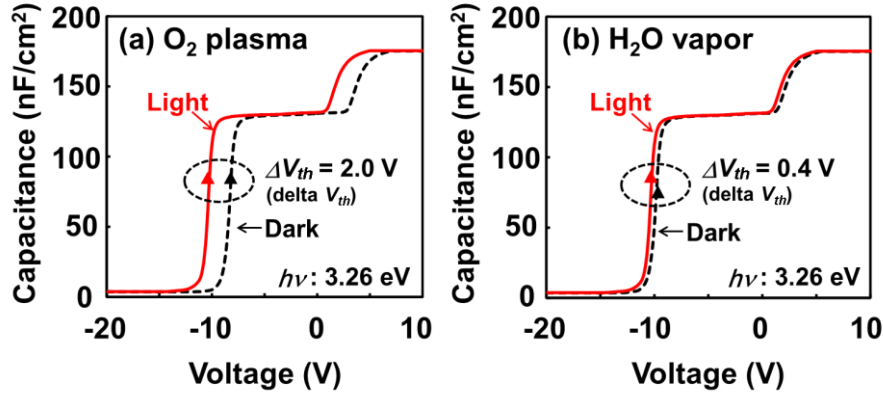
Fig. 4-11. C–V curves of AlGaN/GaN MOS-HEMTs obtained before and after light irradiation when using (a) O 2 plasma-Al 2 O 3 and (b) H 2 O vapor-Al 2 O 3 . Photon energy was applied at 3.26 eV (Reproduced from ref. 10, copyright 2013 by the Japan Society of Applied Physics).
