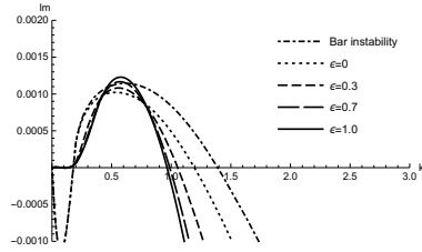
Figure 4.12: Plot for C_f=0.005 , \beta=10
