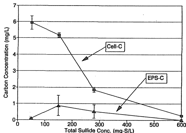
Figure 10. Change in cellular and EPS carbon concentrations with changing total sulfide concentration. Error bars represent the standard errors of measurement ( n = 2 ).
