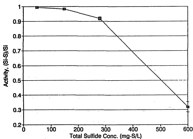
Figure 9. Response of lactate oxidation [S_i - S]/S_i to change in the total sulfide concentration: D = 0.2 \text{ h}^{-1} , temperature 35^\circ\text{C} , pH 7.0. \text{Na}_2\text{S} \cdot 9\text{H}_2\text{O} was added to obtain desired total sulfide concentration. Error bars represent the standard error of measurement ( n = 2 ). The error bar is not presented except for 600 mg TS/L because the other standard errors are so small (Table V).
