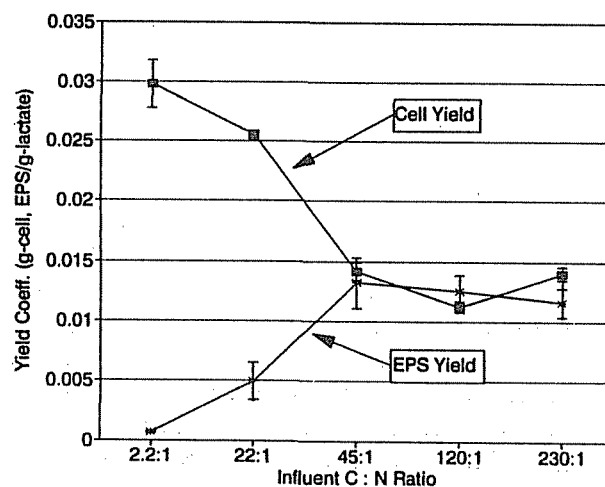
Figure 8. Change in cell and EPS yield coefficients with changing C:N ratio. Error bars represent the standard errors of measurement ( n = 2 ).
