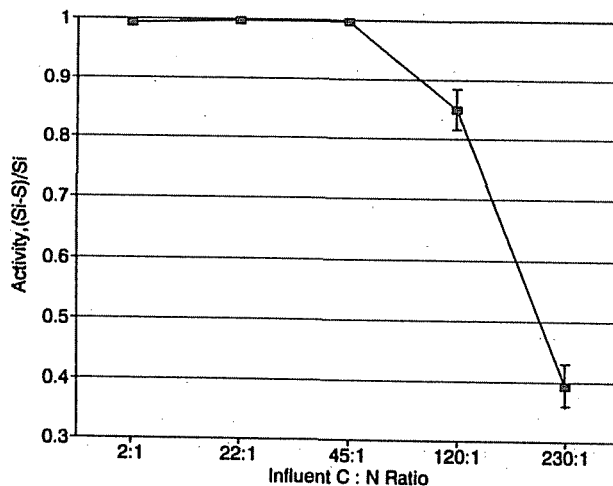
Figure 7. Response of lactate oxidation ((S_i - S)/S_i) to change in the carbon (C):nitrogen (N) ratio: D = 0.2 \text{ h}^{-1} , temperature = 35^\circ\text{C} . The limiting C:N ratio (w/w) is in the range 45:1-120:1. Error bars represent the standard error of measurement ( n = 2 ). The error bar is not presented except for two points at 120:1 and 230:1 because the other standard errors are so small (Table IV).
