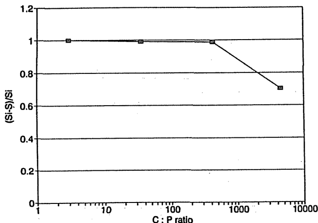
Figure 5. Response of lactate oxidation ((S_i - S)/S_i) by D. desulfuricans to change in the phosphorous concentration: D = 0.2 \text{ h}^{-1} , temperature 35^\circ\text{C} . The limiting C:P ratio is in the range 400:1 to 800:1.
