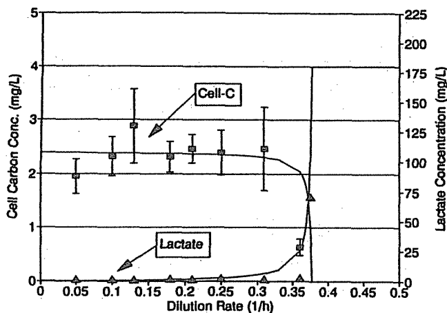
Figure 1. Experimental dependence of the steady state cellular carbon and lactate concentration on the dilution rate at 25°C. The solid lines are drawn using chemostat mass balance equations. The influent lactate concentration was 180 \text{mg/L} . Error bars represent the standard deviation of triplicate measurements.
