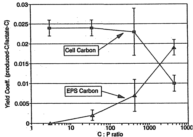
Figure 6. Change in cell and EPS carbon yield coefficients with changing C:P ratio. Error bars represent the standard deviation triplicate measurements.
