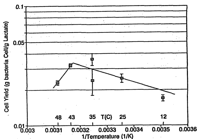
Figure 4. Temperature dependence of the cell yield coefficient ( Y_{c/Lac} ). The highest cellular yield was observed around optimum temperature for growth. Error bars represent the standard error of the estimated Y_{c/Lac} .
