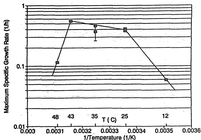
Figure 2. Temperature dependence of the maximum specific growth rate ( \mu_{\max} ). The highest \mu_{\max} of 0.55 h -1 was obtained at 43°C. The activation energies for \mu_{\max} were 14 KJ/mol in the range 25–43°C and 104 KJ/mol below 25°C. Error bars represent the standard error of the estimated \mu_{\max} . The error bar was not given except one point at 35°C because their standard errors are so small (Table V).
