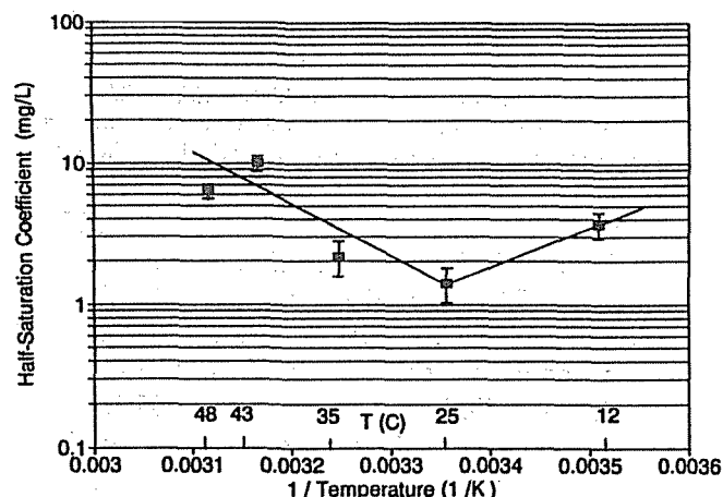
Figure 3. Temperature dependence of the half-saturation coefficient ( K_{Lac} ). The activation energies were 47 KJ/mol above 25°C and -52 KJ/mol below 25°C. Error bars represent the standard error of the estimated K_L .
