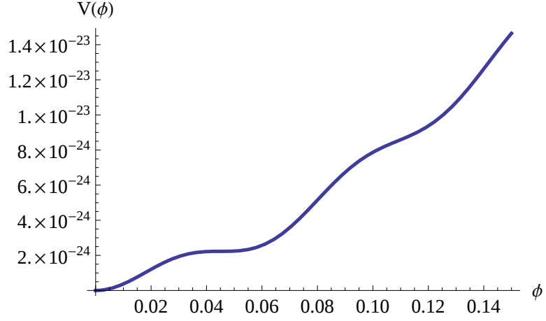
Figure 3.14: - The inflaton potential is drawn by setting the parameters as A_1/A_2 = 22.474579785926 and A_2 = 6.47 \times 10^{-25} .
