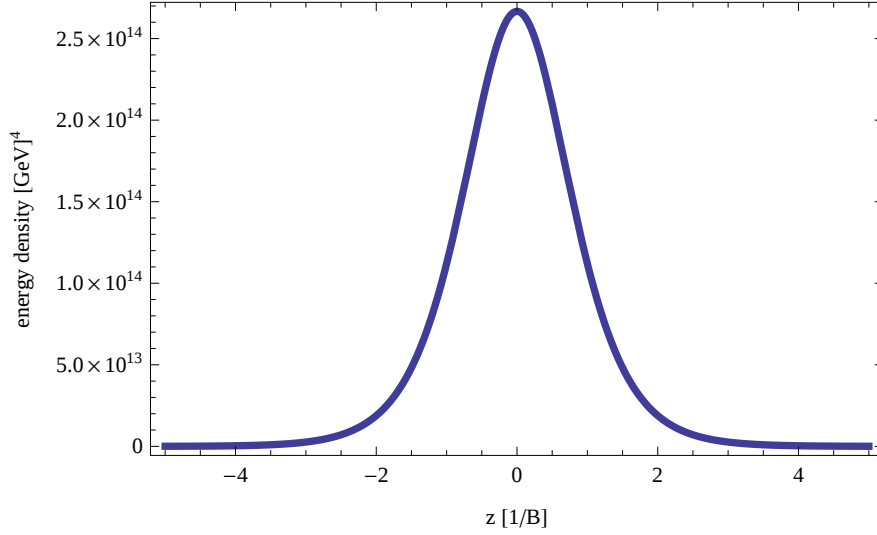
Figure 5.2: - Spatial configuration of a domain wall energy density for \lambda = \kappa = 0.01 , A_\lambda = A_\kappa = 10 \text{ TeV} , \mu = 1 \text{ TeV} , \tan \beta = 10 . The z -axis is normalized by 1/B .
