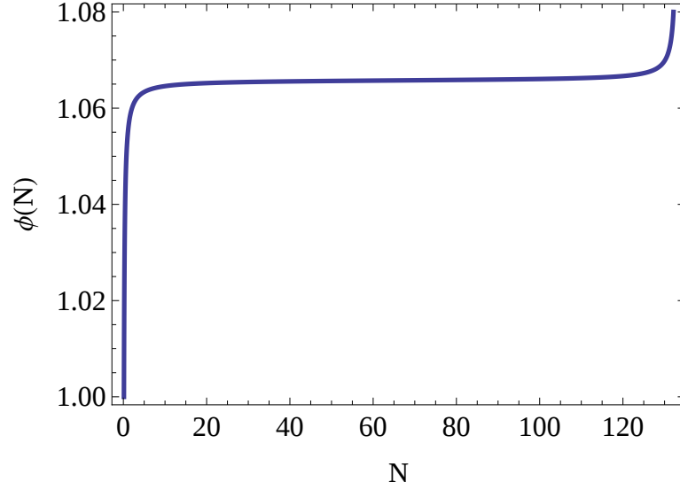
Figure 3.5: - The inflaton amplitude as a function of the number of e-folds \phi(N) for f = 0.1 , \Lambda_1/\Lambda_3 = 4.9 and \Lambda_2/\Lambda_3 = 0.25 (corresponding to V_{\text{inf}}^{1/4}(N = 55) = 6.1 \times 10^{-5} ).
