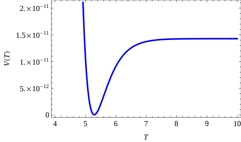
Figure 3.23: - A canonically normalized potential which is given by eqs.(3.67), (3.72) and (3.71), while the original one is already shown in Figure. 3.22. We put the parameters as ( a_1 = 1 , a_2 = 1 , a_3 = 1 , c_1 = 1.01 , c_2 = 250 ).
