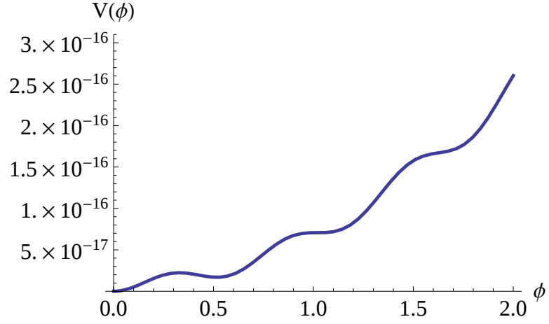
Figure 3.1: - The axion inflation potential with a sub-Planck axion decay constant f = 0.1 for the small field axion inflation (the field excursion \Delta\phi < 1 during the inflation).
