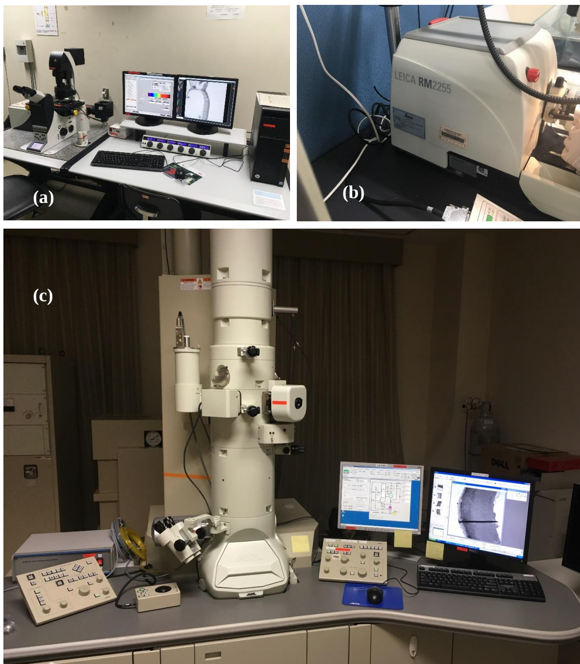
Fig. 29. Transmission Electron Microscope sample preparation. a. Laser microscope, b. fully automated Leica RM2255 rotary microtome, c. Transmission Electron microscope.
