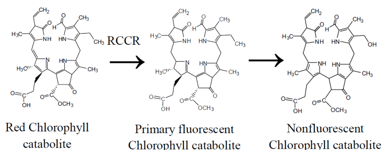
Fig. 3. The last stage of Chl degradation pathway in higher plants. The pathway of the late stage includes the cleavage reaction and steps after the reaction. And the products in late stage are colorless.
