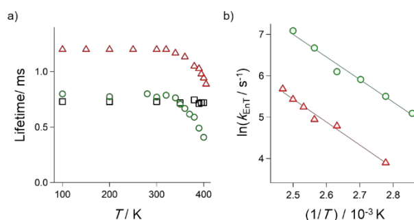
Figure 5. (a) Temperature-dependent emission lifetimes of Tb-TPPO (black square), Tb-PEB (red triangle) and Tb-BPEB (green circle) excited at 355 nm (Nd:YAG 3 \omega ), and the (b) Arrhenius plot for energy-transfer rate of Tb-PEB (red triangle) and Tb-BPEB (green circle). Arrhenius equation: \ln(1/\tau_{\text{obs}} - 1/\tau_{100\text{K}}) = \ln(k_{\text{EnT}}) = \ln(A) - (E_a/k_B T) .
