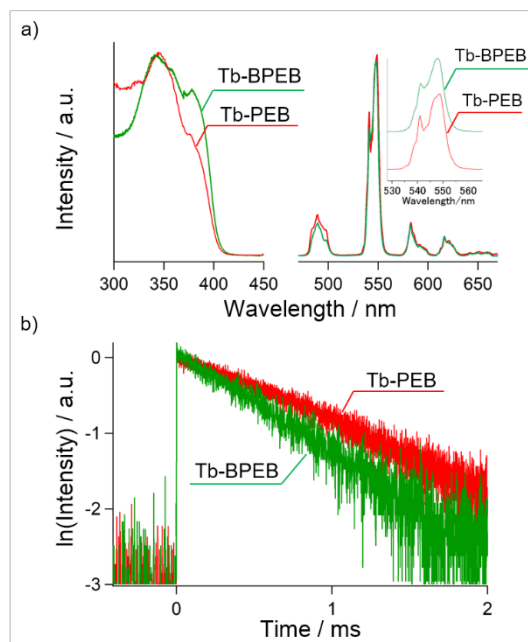
Figure 3. (a) Excitation and emission spectra of Tb-PEB (red line) and Tb-BPEB (green line) in solids at room temperature. Excitation spectra were recorded in respect to emission at 544 nm ( ^5D_4 \rightarrow ^7F_6 ) and were normalized at 350 nm. Emission spectra were excited at 350 nm. (b) Emission decay profiles of Tb-PEB (red line) and Tb-BPEB (green line) in solids at room temperature excited at 355 nm (Nd:YAG 3 \omega ).
