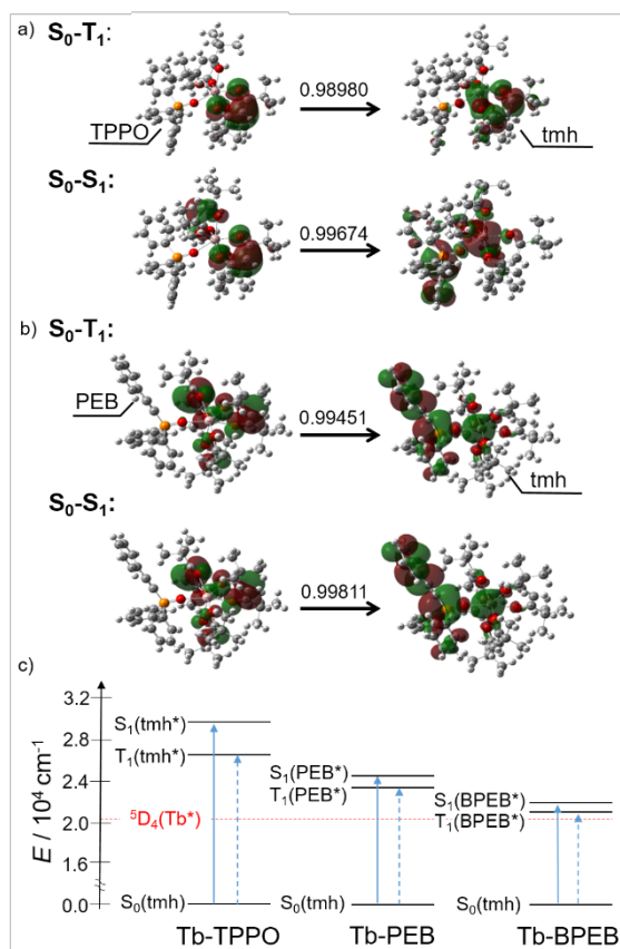
Figure 4. Molecular orbital representations of the lowest triplet and singlet excited states of (a) Tb-TPPO and (b) Tb-PEB simplified by NTO showing the highest transition probability. (c) Energy diagram for the lowest triplet and singlet excited states for Tb-TPPO, Tb-PEB and Tb-BPEB. DFT calculations were performed using \text{Al}^{\text{III}} ions instead of \text{Tb}^{\text{III}} ions for all complexes.
