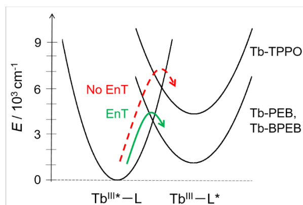
Figure 6. Potential curves showing the energy transfer from \text{Tb}^{\text{III}} excited state ( ^5D_4 ) to the ligands' excited states.
