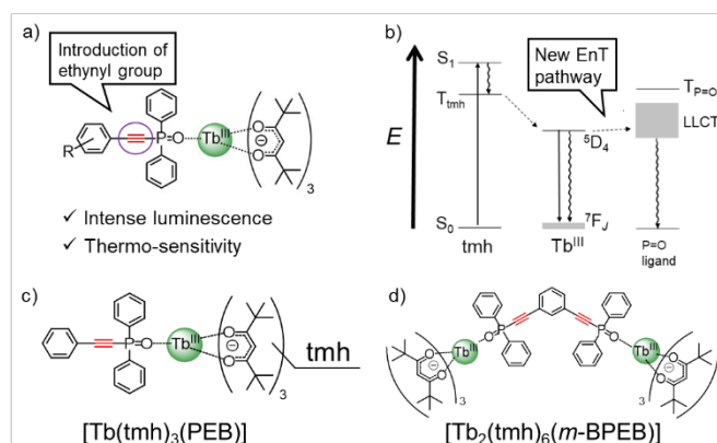
Figure 1. (a) Conceptual molecular design, (b) Energy diagram of Tb III complexes with ethynyl group, (c) Mono-nuclear [Tb(tmh) 3 (PEB)], and (d) Di-nuclear [Tb 2 (tmh) 6 ( m -BPEB)].
