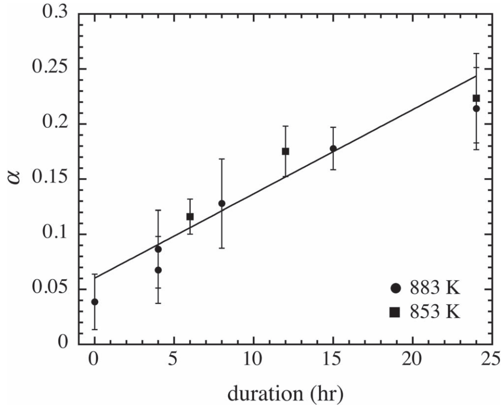
Figure 10. Time evolution of the degree of oxygen isotopic exchange ( \alpha ) obtained from \Delta\kappa/\kappa_0 of samples heated at 883 K (circle) and 853 K (square) and 0.01 Pa of \text{H}_2^{18}\text{O} vapor. The solid line represents the best-fit line by Equation (3). Error bars are the 1\sigma standard deviations of the means.
