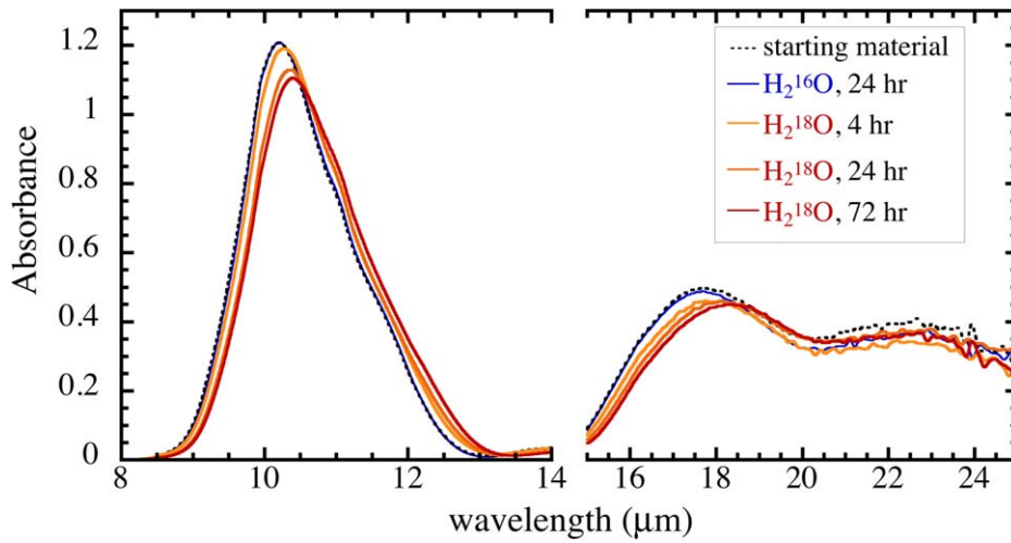
Figure 2. Infrared adsorption spectra of amorphous forsterite used as the starting material (dotted curve) and samples heated at 853 K and 0.3 Pa of \text{H}_2^{16}\text{O} vapor (blue solid curve) or \text{H}_2^{18}\text{O} vapor (orange to red solid curves) for different durations.
