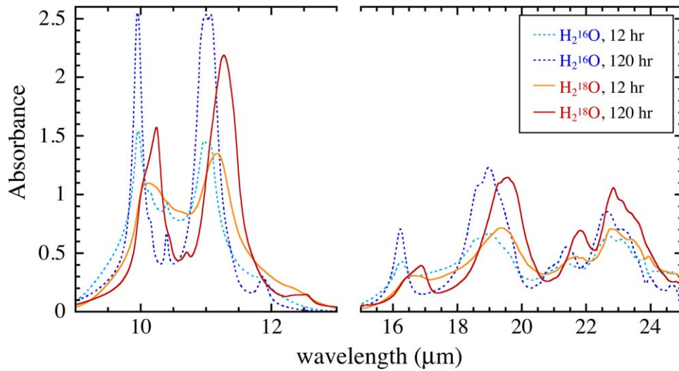
Figure 5. Infrared adsorption spectra of samples heated at 0.3 Pa of \text{H}_2^{16}\text{O} or \text{H}_2^{18}\text{O} vapor for 12 and 120 hr at 953 K.
