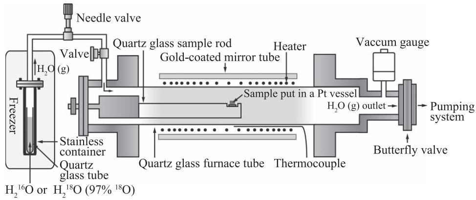
Figure 1. Schematic illustration of the vacuum furnace configuration.
