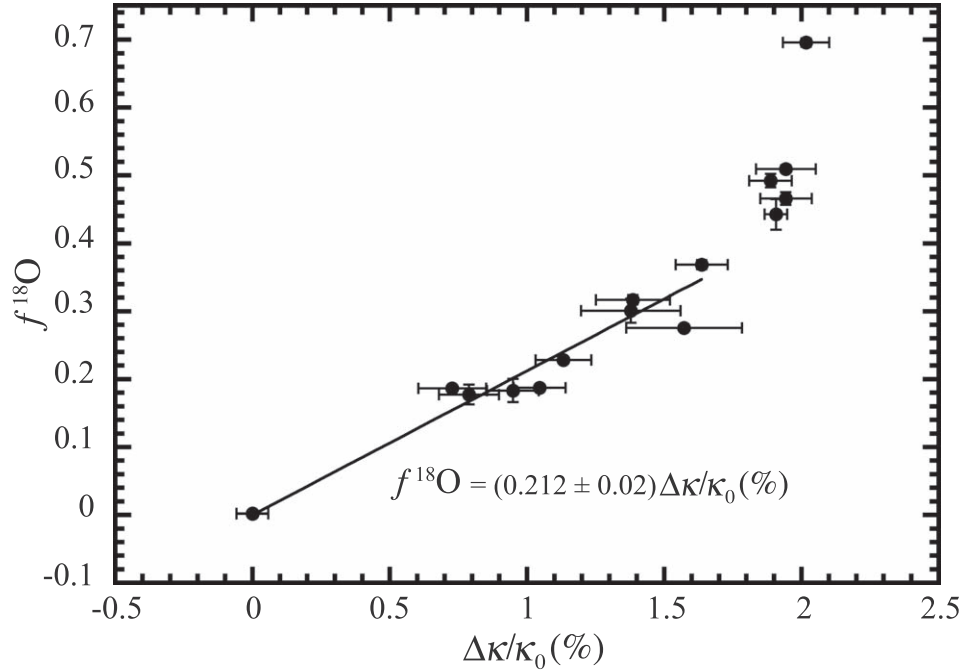
Figure 4. Comparison of the oxygen isotopic composition f^{18}\text{O} = {}^{18}\text{O}/({}^{18}\text{O} + {}^{16}\text{O}) and \Delta\kappa/\kappa_0 . A linear correlation is found between f^{18}\text{O} and \Delta\kappa/\kappa_0 of <\sim 1.64\% . Error bars are the 1\sigma standard deviations of the means.
