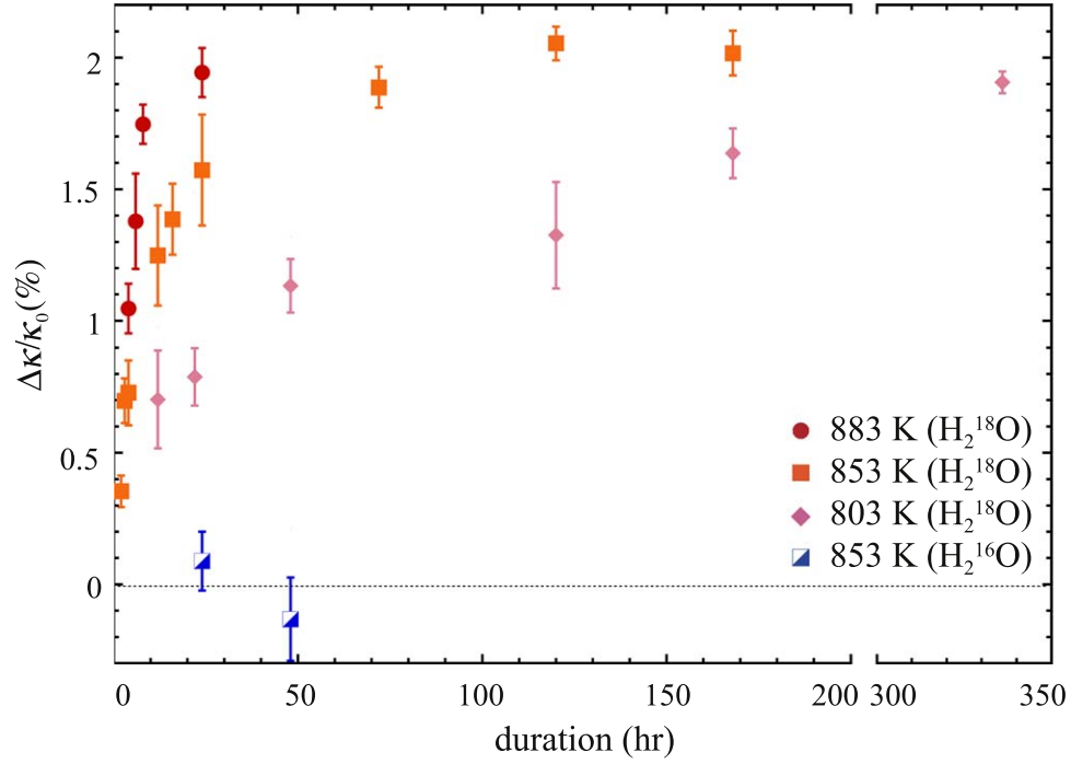
Figure 3. Relative peak shifts ( \Delta\kappa/\kappa_0 ; see text in detail) of the 10\ \mu\text{m} infrared absorption feature of amorphous forsterite heated at 0.3 Pa of \text{H}_2^{18}\text{O} vapor at 883, 853, and 803 K for different durations. The \Delta\kappa/\kappa_0 of the amorphous forsterite heated at 0.3 Pa of \text{H}_2^{16}\text{O} vapor and 853 K are also shown for comparison. Error bars represent the 1\sigma standard deviations of the means of several measurements of the same sample.
