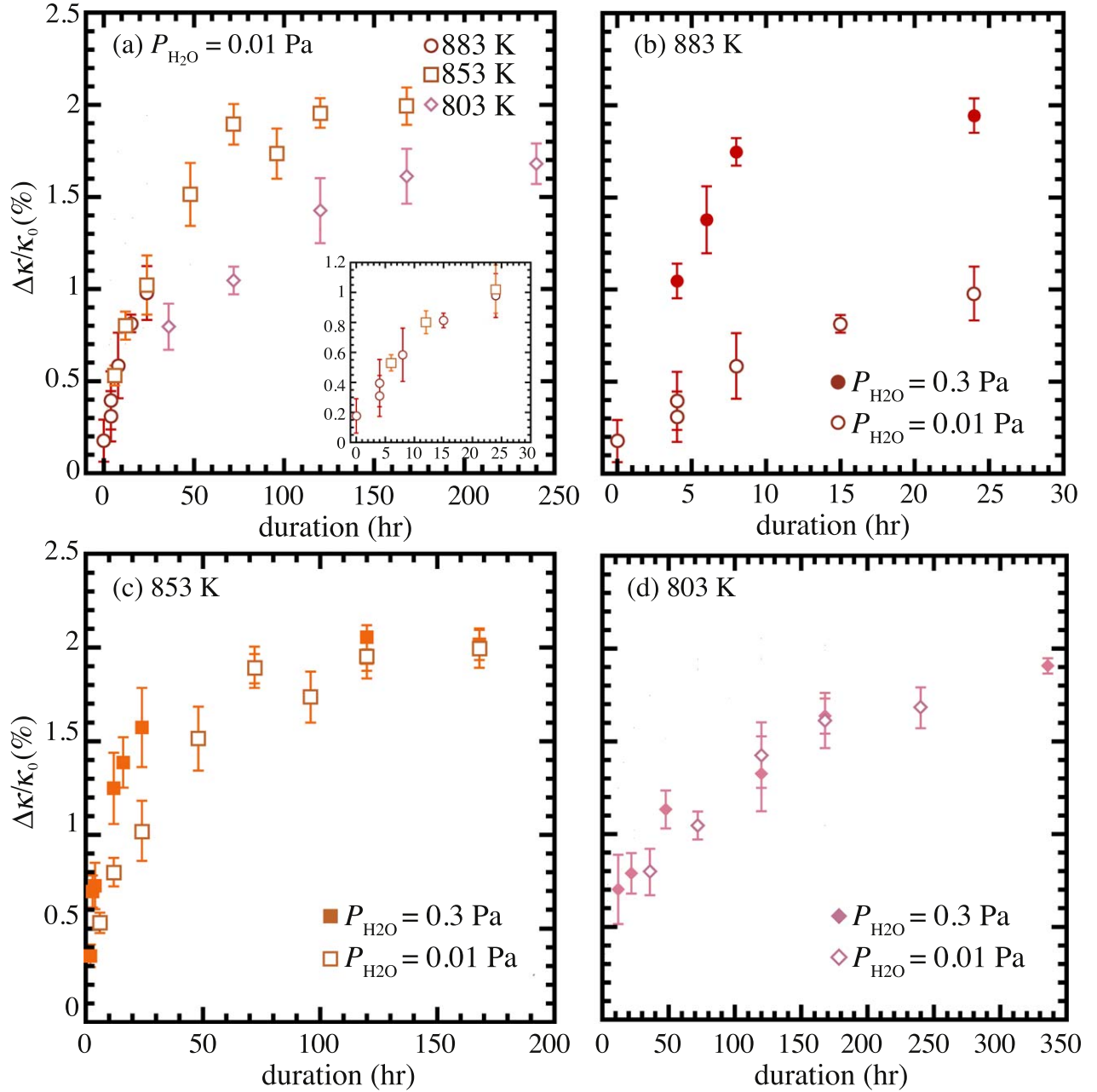
Figure 7. (a) Temporal changes of relative peak shifts ( \Delta\kappa/\kappa_0 ) of the 10\ \mu\text{m} infrared absorption feature of amorphous forsterite heated at 803, 853, and 883 K and 0.01 Pa of \text{H}_2^{18}\text{O} . An inset shows the temporal change of \Delta\kappa/\kappa_0 for shorter heating durations. Error bars represent the 1\sigma standard deviations of the means of several measurements of the same sample. (b) Temporal changes of \Delta\kappa/\kappa_0 at 0.01 and 0.3 Pa of \text{H}_2^{18}\text{O} vapor at 883 K. These are also shown at 853 K (panel (c)) and 803 K (panel (d)).
