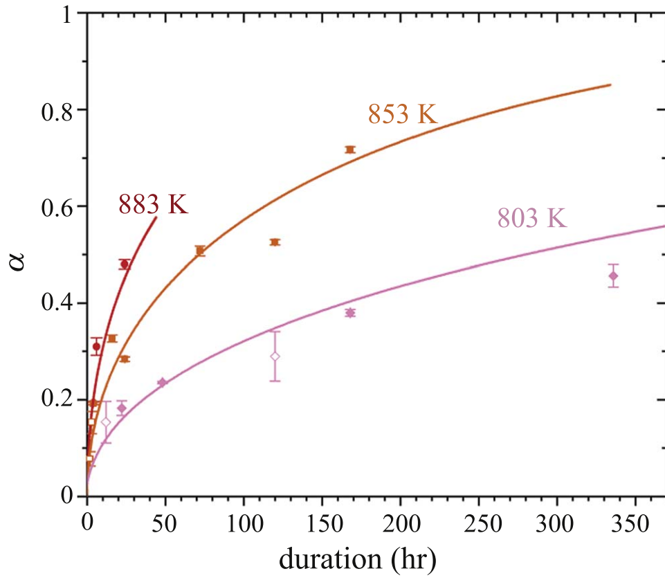
Figure 8. Time evolution of the degree of oxygen isotopic exchange ( \alpha ) at 0.3 Pa of \text{H}_2^{18}\text{O} vapor and 803, 853, and 883 K. The solid curves represent the fitting results by Equation (1). Filled symbols are the data measured by SIMS, and open symbols are those estimated from \Delta\kappa/\kappa_0 (%) of samples. Error bars are the 1\sigma standard deviations of the means.
