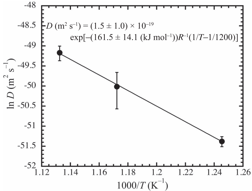
Figure 9. Arrhenius plot of the diffusive isotopic exchange rate constant ( D ) at P_{\text{H}_2\text{O}} of 0.3 Pa. Errors represent the 1\sigma standard deviations of the means.
