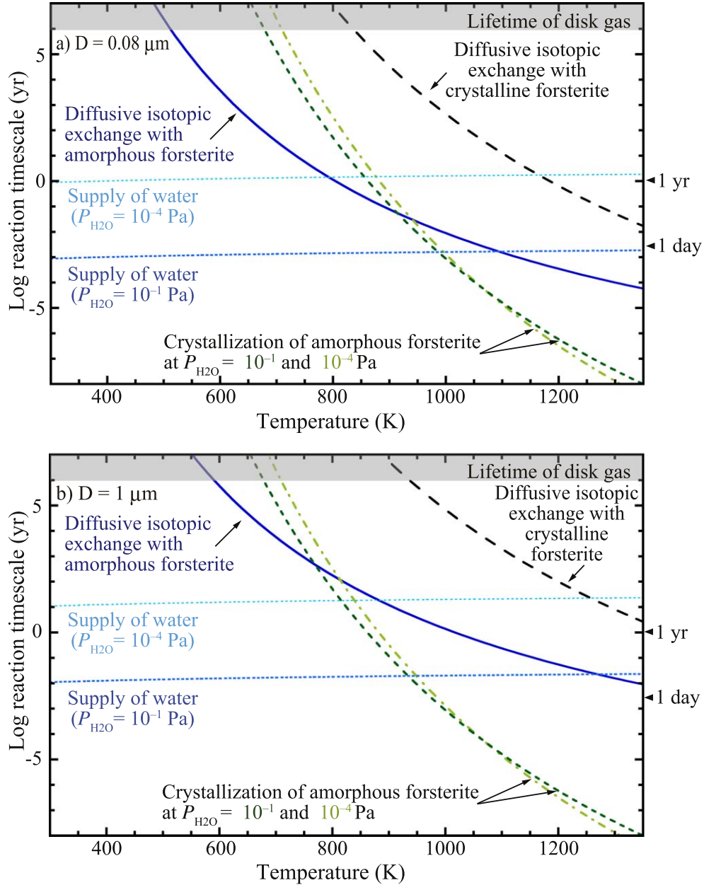
Figure 11. Timescales of oxygen isotopic exchange between amorphous forsterite dust and water vapor in protoplanetary disks controlled by the diffusive isotopic exchange reaction (solid curves) and the supply of water molecules at P_{\text{H}_2\text{O}} of 10^{-1} and 10^{-4} \text{ Pa} (dotted curves). Timescales of oxygen self-diffusion in crystalline forsterite (long-dashed curves; Jaoul et al. 1980) and crystallization of amorphous forsterite at P_{\text{H}_2\text{O}} of 10^{-1} and 10^{-4} \text{ Pa} (short-dashed and dotted-dashed curves, respectively; Yamamoto & Tachibana 2018) are shown for comparison. The estimated lifetime of protoplanetary disk gas (1–10 Myr) is also shown for comparison. (a) 0.08 \mu\text{m} . (b) 1 \mu\text{m} .
