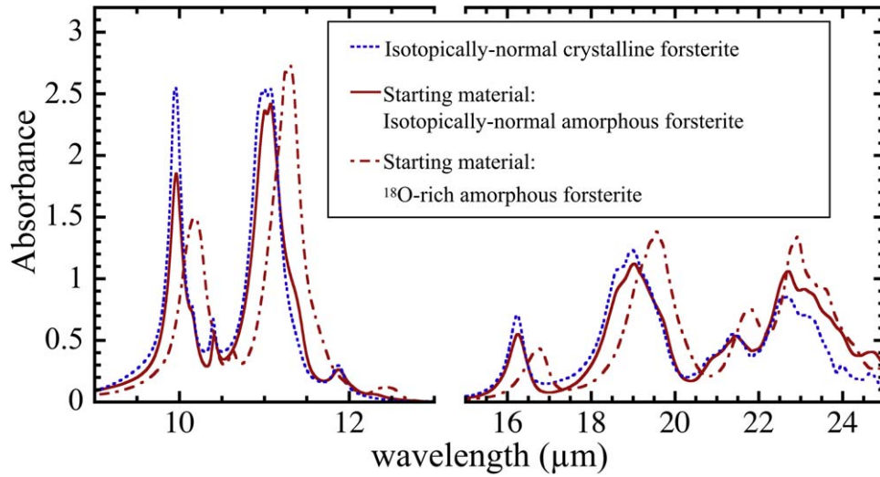
Figure 6. Infrared spectrum of forsterite crystallized at 1073 K and 0.3 Pa of \text{H}_2^{18}\text{O} vapor for 2 hr from the starting material (red solid curve). The spectrum of forsterite crystallized at the same condition from amorphous forsterite that was preheated at 853 K and 0.3 Pa of \text{H}_2^{18}\text{O} vapor for 120 hr is shown as a red dotted-dashed curve. An infrared spectrum of the isotopically normal crystalline forsterite is also shown for comparison (blue dotted curve).
