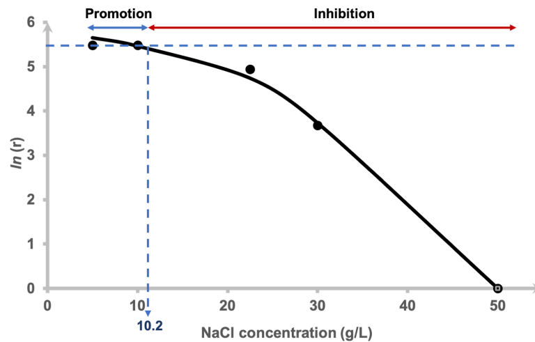
Figure 2 Effects of NaCl on the hydrogen production rate of Vibrio tritonius . Logarithm of hydrogen production rate, [\ln(r)] and relative activity using a non-competitive inhibition model. The fitted curve was drawn in full lines.
