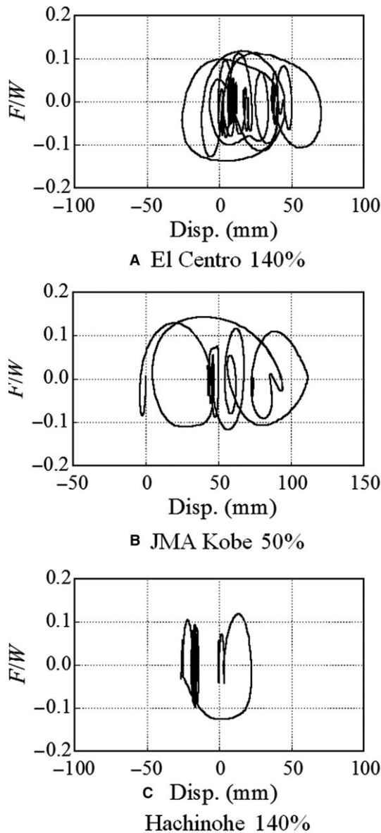
Figure 12. F/W–Horizontal displacement relationships
