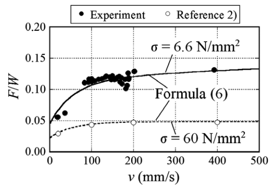
Figure 26. F/W -velocity relationships
