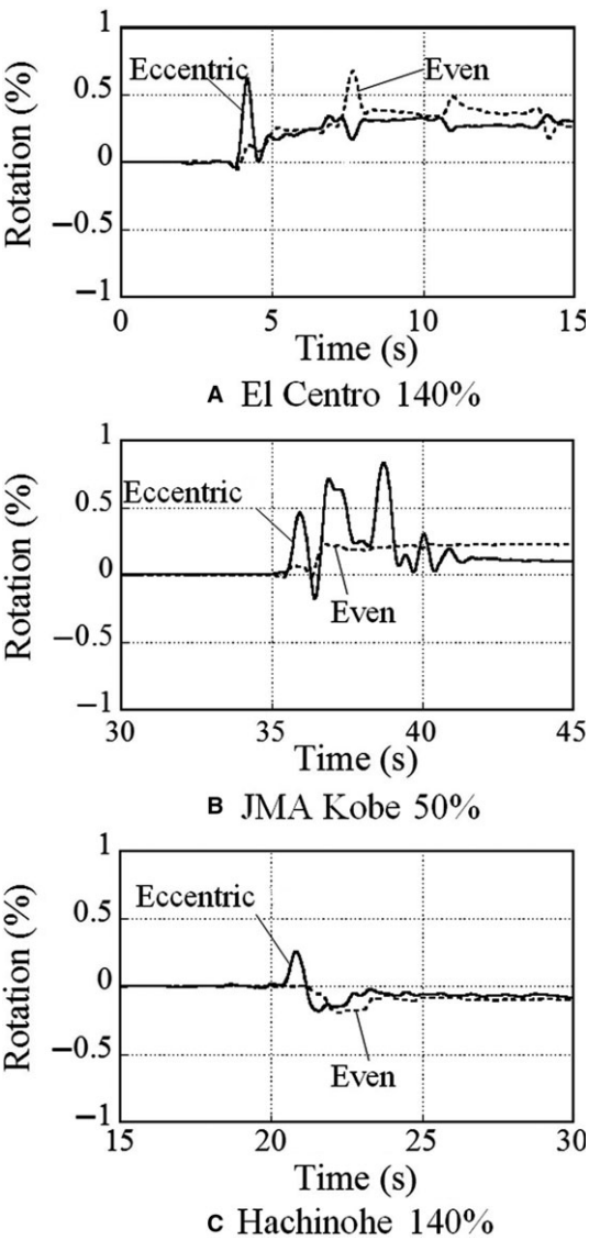
Figure 17. Twisting angle time histories
