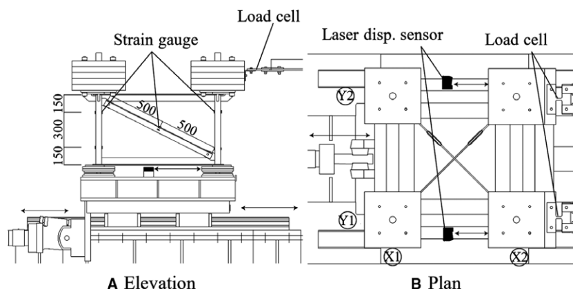
Figure 5. Measurement instrumentation
