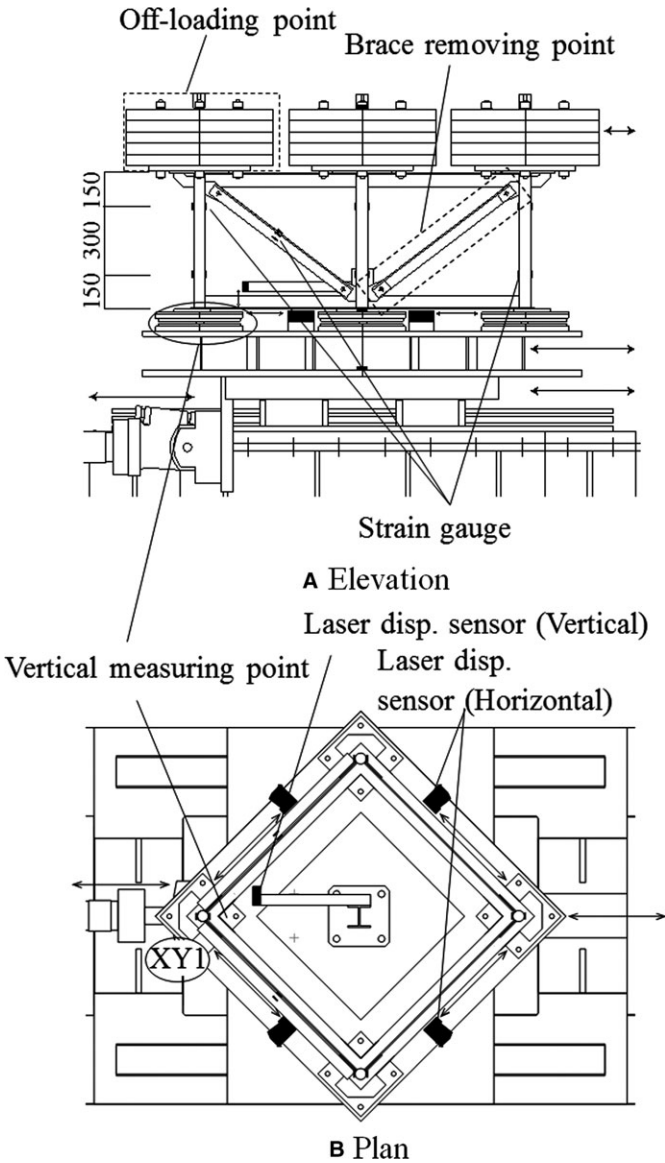
Figure 20. Measurement instrumentation
