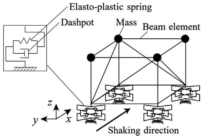
Figure 30. Analysis model
