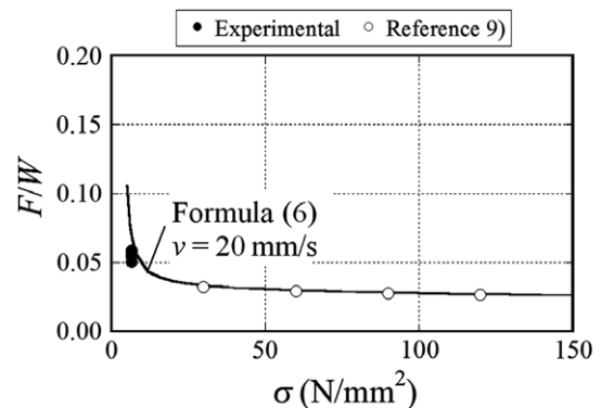
Figure 27. F/W -pressure relationships
