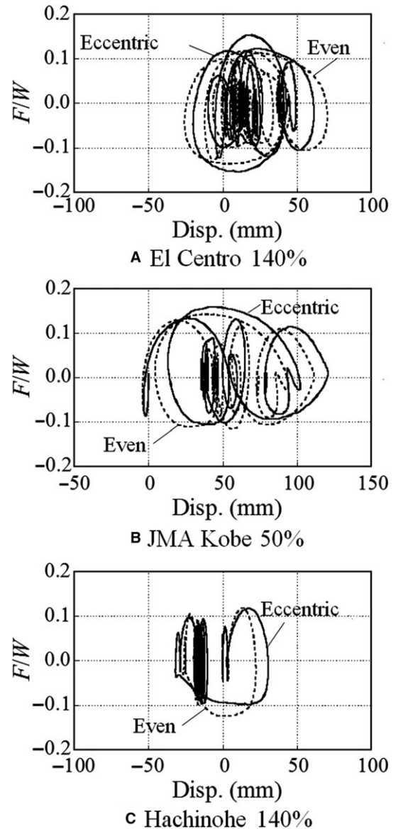
Figure 16. F/W–Horizontal displacement relationships
