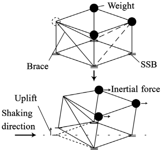
Figure 19. Uplift mode
