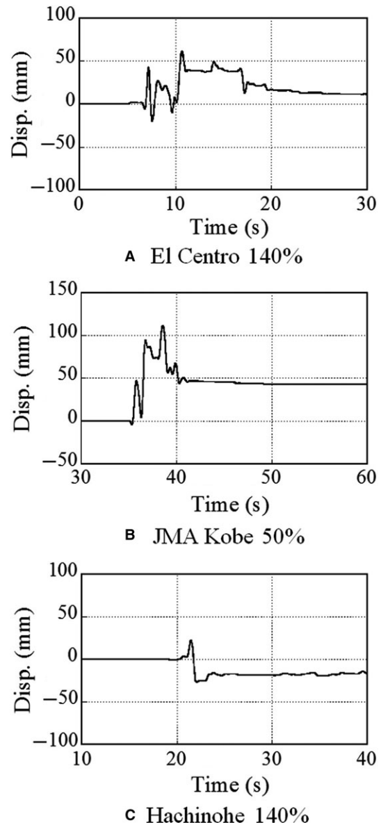
Figure 13. Horizontal displacement time histories
