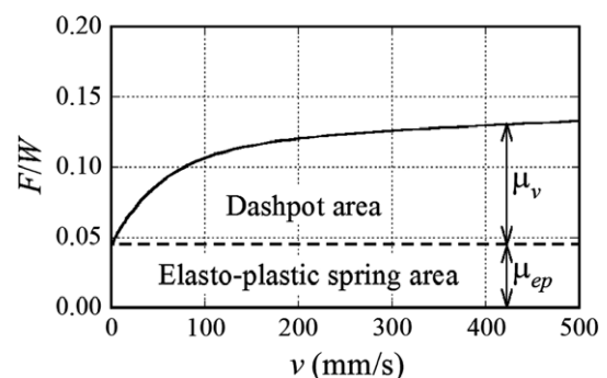
Figure 28. F/W - v relationship of SSB model (pressure 6.6 \text{ N/mm}^2 )
