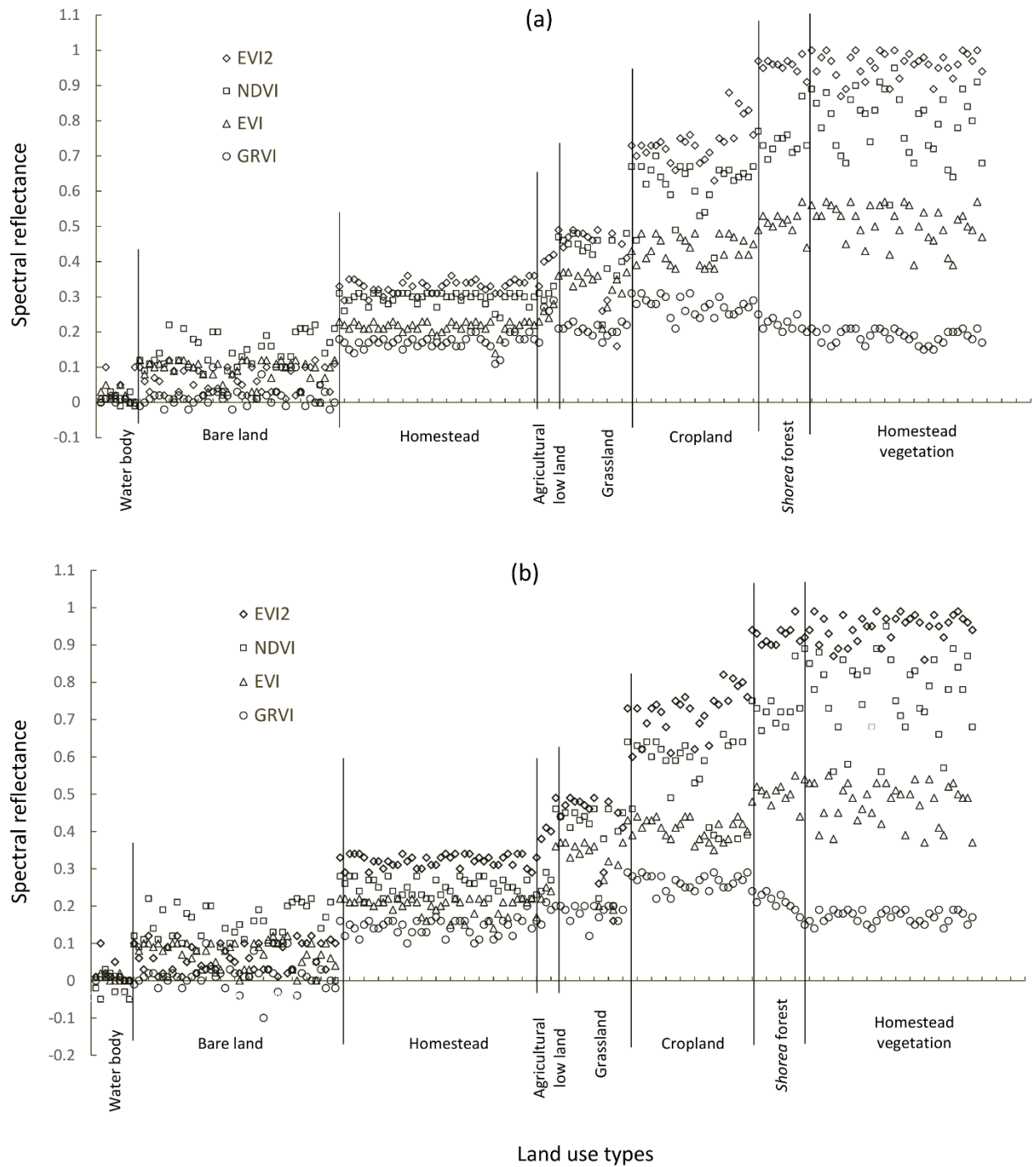
Fig. 3 Spectral reflectances in the VIs extracted from 182 ground truth points for eight land use classes. The y-axis indicates the spectral reflectances among the four VIs, while the x-axis represents the eight land use types
