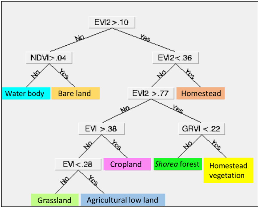
Fig. 4 A DT constructed using the hierarchical classification of land use types. Numerals with inequality signs indicate the VI values that represent the thresholds of the classifiers
