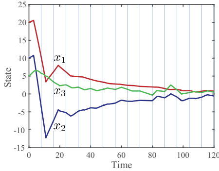
Fig. 2. Time response of the state. Red line: the first element of the state ( x_1 ). Blue line: the second element of the state ( x_2 ). Green line: the third element of the state ( x_3 ).
