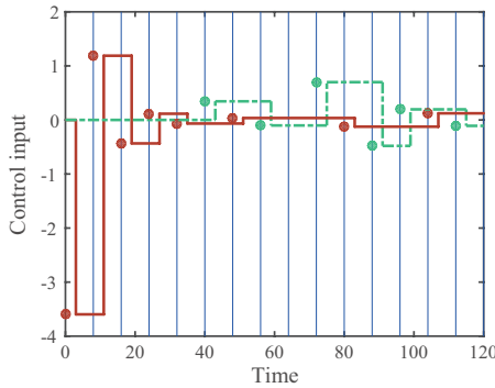
Fig. 3. Time response of the control input. Solid line: the control input u_1 . Dash line: the control input u_2 . Circles imply the control inputs computed at 2Ll , l = 0, 1, 2, \dots . After the message about the control input reaches the plant, computed control inputs are applied to the plant.
