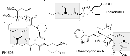
Figure 1. Biologically active compounds
