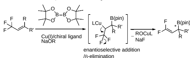
Scheme 1. Catalytic Enantioselective Synthesis of Allyl Boronates
