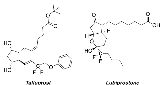
Figure 1. Representative Bioactive gem -Difluoromethylene-containing Molecules.
