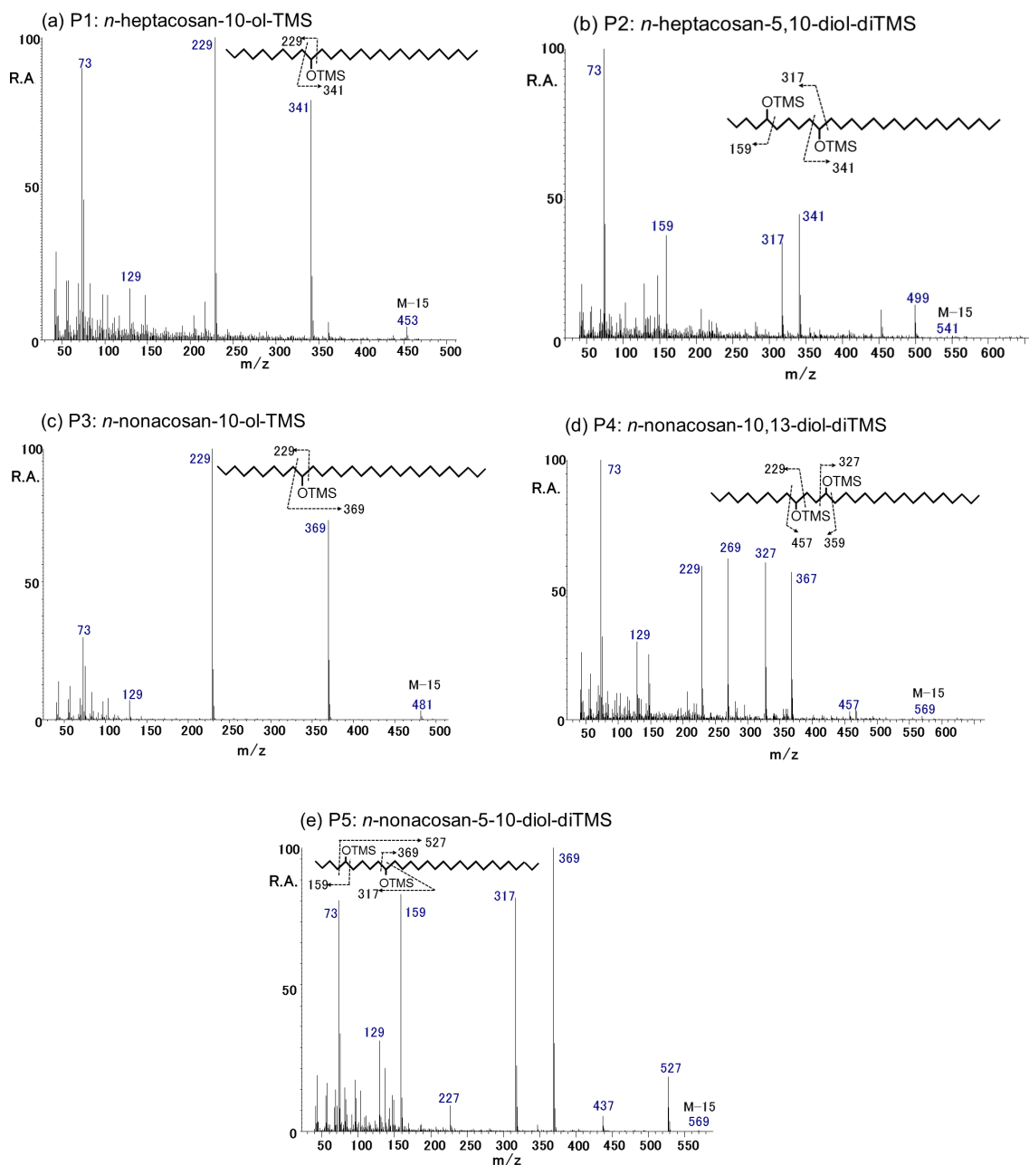
Figure 3. EI mass spectra obtained for the TMS derivatives of the identified secondary fatty alcohols. (a) P1: n -heptacosan-10-ol-TMS, (b) P2: n -heptacosan-5,10-diol-diTMS, (c) P3: n -nonacosan-10-ol-TMS, (d) P4: n -nonacosan-10,13-diol-diTMS, and (e) P5: n -nonacosan-5-10-diol-diTMS.
