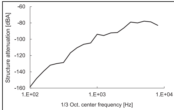
Figure 3. Structural attenuation of the test engine.
