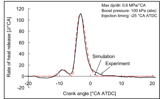
Figure 5. Heat release data in the engine experiment and simulation.
