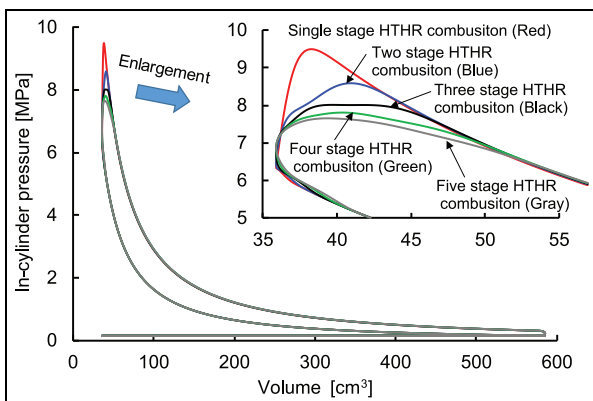
Figure 23. Pressure-volume histories (PV line) for multiple fuel injections.
