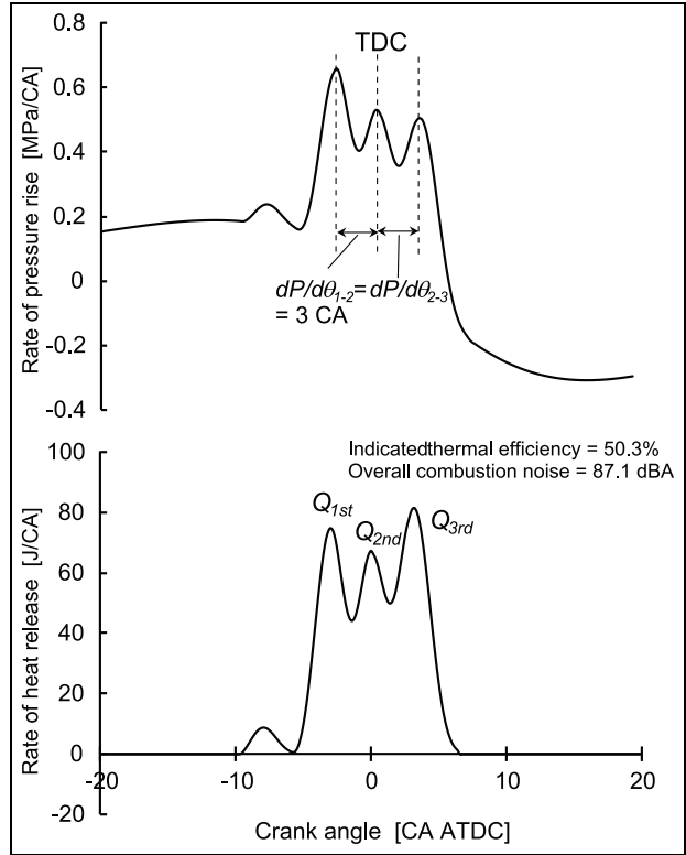
Figure 12. Optimum shapes of heat release and rate of pressure rise for the higher indicated thermal efficiency and lower combustion noise in the three-stage HTHR combustion.
