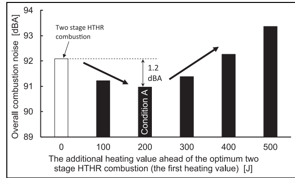
Figure 9. Overall combustion noise versus the additional heating value added ahead of the two-stage HTHR combustion.
