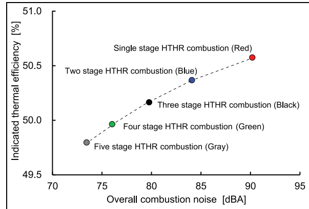
Figure 24. Overall combustion noise versus indicated thermal efficiency for multiple fuel injections.
