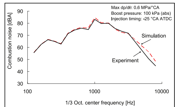
Figure 6. Plots of the combustion noise in the engine experiment and simulation.
