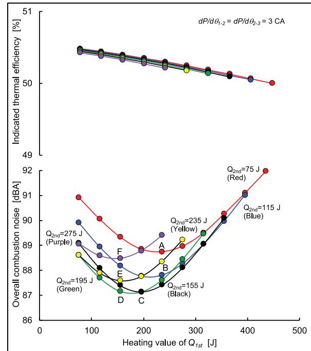
Figure 13. Effect of Q_{1st} on the indicated thermal efficiency and overall combustion noise.
