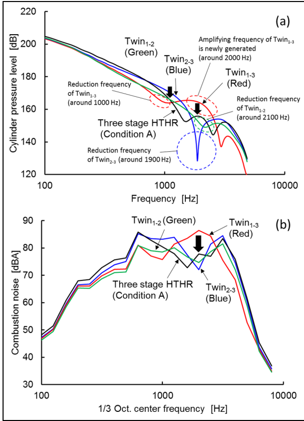
Figure 11. (a) Cylinder pressure levels and (b) frequency characteristics of the three-stage HTHR combustion and the three sets of two-stage HTHR heat releases: Twin_{1-2} , Twin_{1-3} , and Twin_{2-3} .
