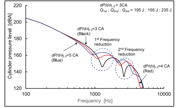
Figure 15. Effects of dP/d\theta_{2-3} on cylinder pressure level.
