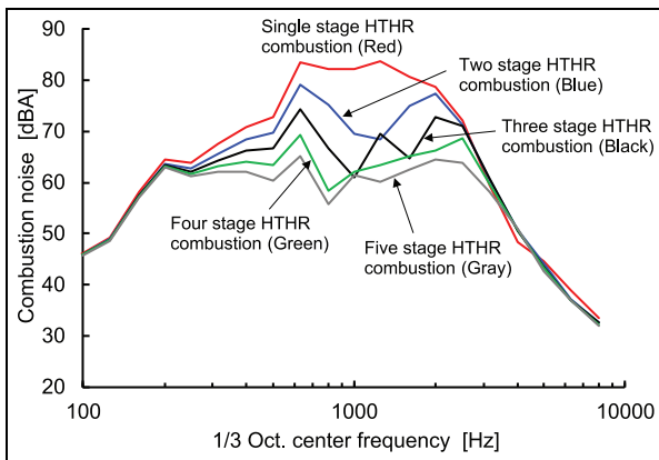
Figure 22. Frequency characteristics of combustion noise with 1–5 fuel injections.
