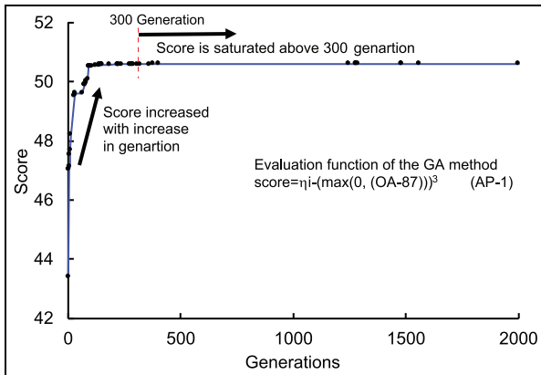
Figure 26. Score history of generation-based algorithm method against generations (equation (10)).
