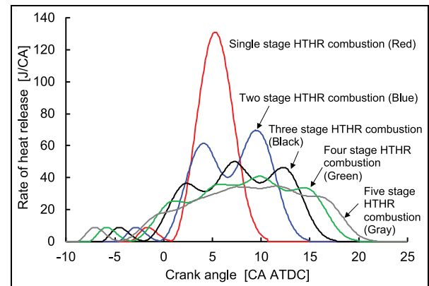
Figure 20. Optimum heat releases for one to five injections calculated by the GA method.
