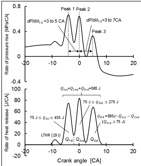
Figure 8. Variable parameters in the calculations for Tests 2 and 3.
