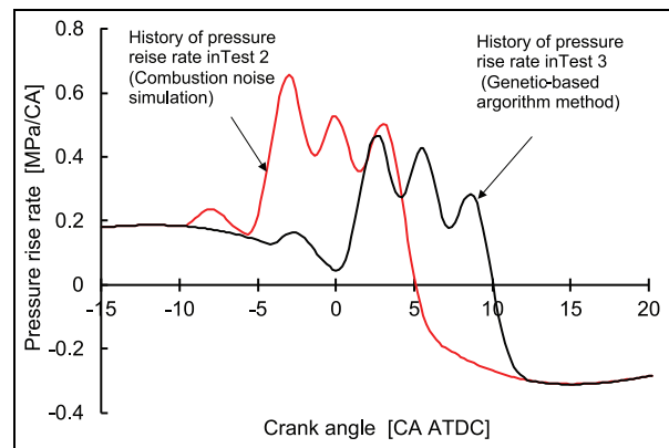
Figure 18. Plot of the pressure rise rates calculated in Test 2 (Combustion noise simulation) and Test 3 (the GA method).
