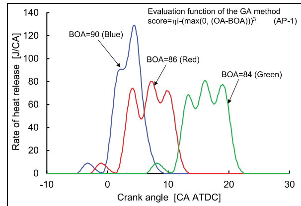
Figure 28. Optimized heat release histories for the basic overall values of 84, 86, and 90 (equation (10)).
