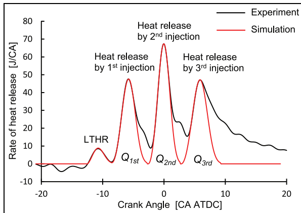
Figure 4. Approximation by the Wiebe function for the three-stage HTHR combustion.
