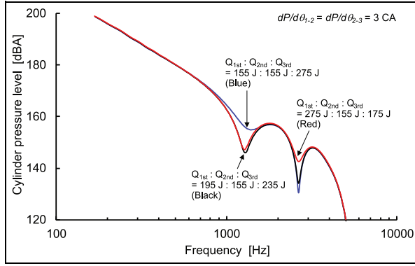
Figure 14. Effects of Q_{1st} and Q_{3rd} on cylinder pressure level (CPL).
