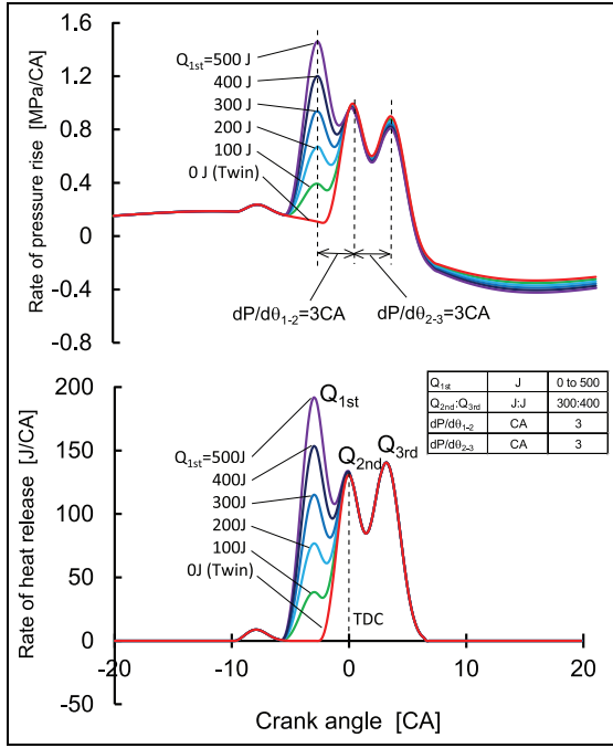
Figure 7. Combustion noise reduction method in three-stage HTHR combustion (Test 1).
