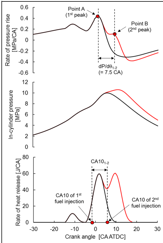
Figure 25. Definitions of CA10_{1-2} and dP/d\theta_{1-2} in two-stage combustion.
