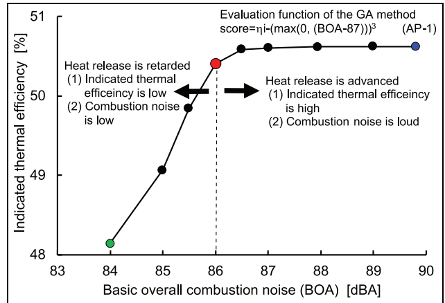
Figure 27. Plots of basic overall combustion noise versus indicated thermal efficiency (equation (10)).
