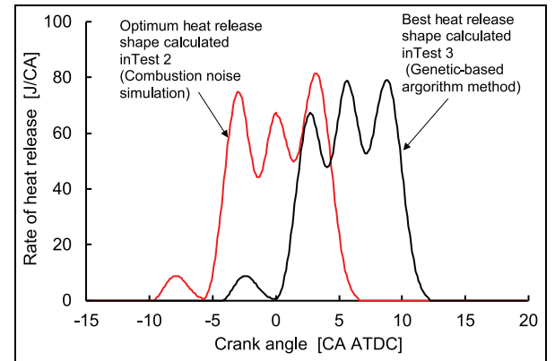
Figure 16. Comparison of heat releases calculated in Test 2 (Combustion noise simulation, red) and Test 3 (the GA method, black).
