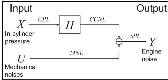
Figure 2. Engine noise generation and analysis model.
