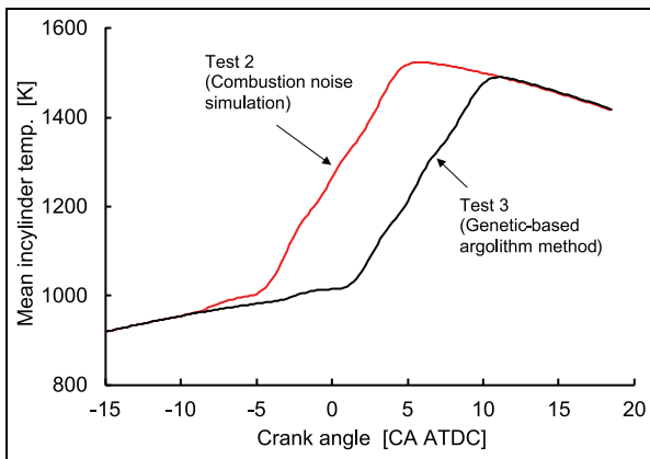
Figure 17. Plots of crank angle versus mean in-cylinder temperature for Test 2 (Combustion noise simulation) and Test 3 (the GA method).
