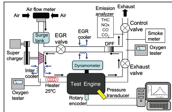
Figure 1. Outline of the engine test set-up.
