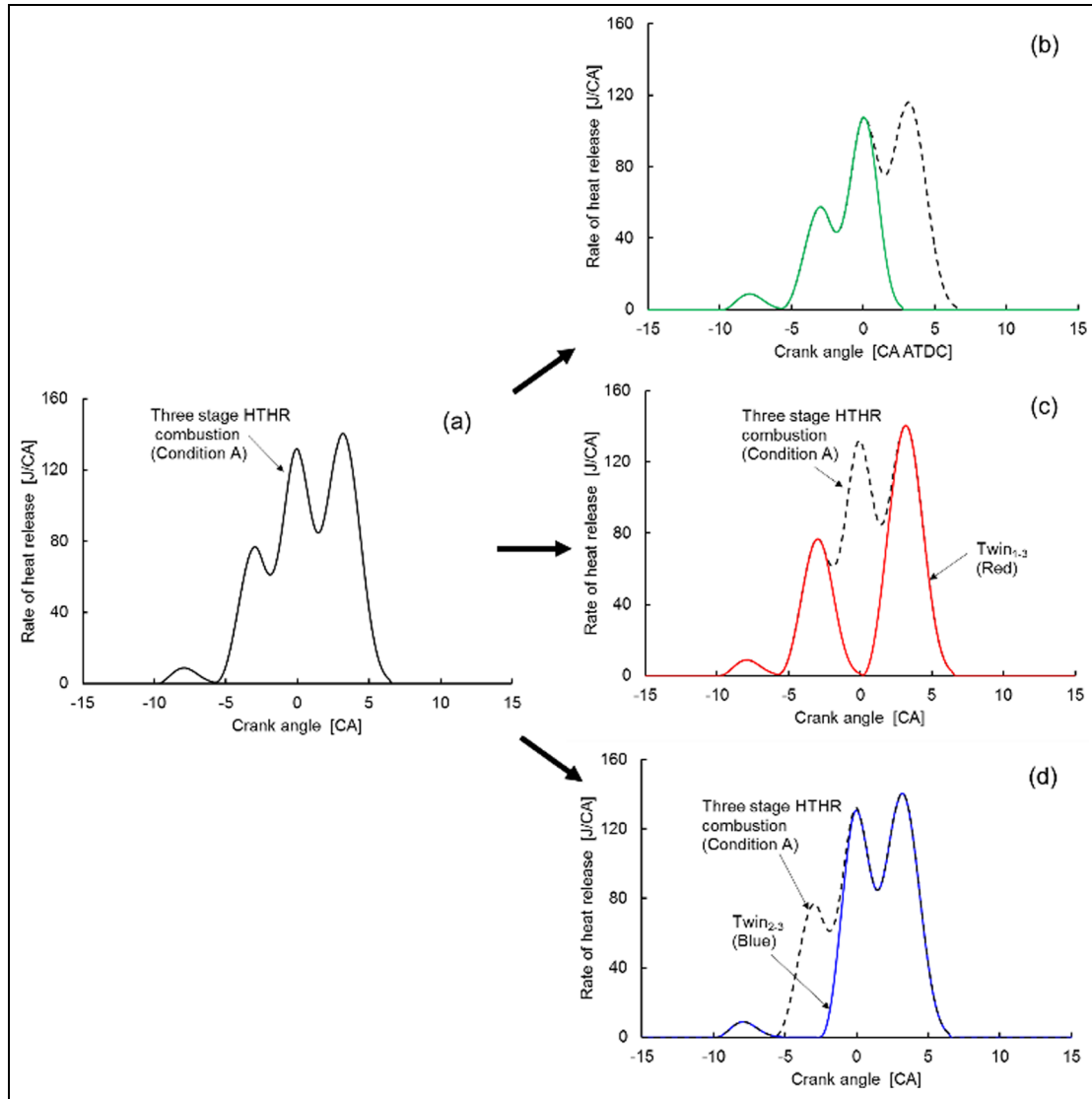
Figure 10. The optimum heat release shape for the three-stage HTHR combustion in Test 2: (a) three-stage HTHR release, (b) Twin_{1-2} , (c) Twin_{1-3} , and (d) Twin_{2-3} .
