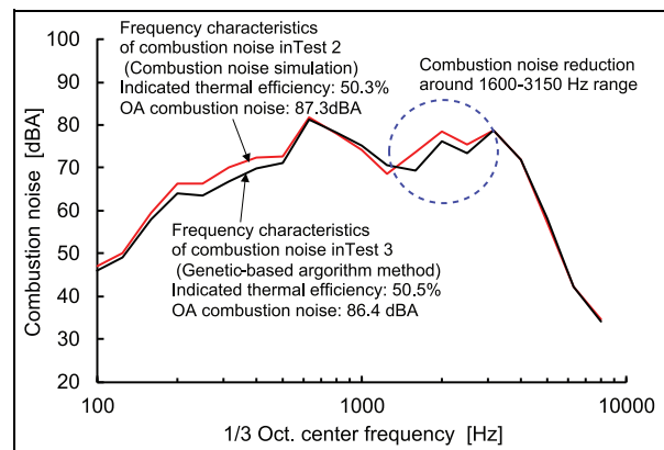
Figure 19. Frequency characteristics of the combustion noise calculated in Test 2 (Combustion noise simulation) and Test 3 (the GA method).
