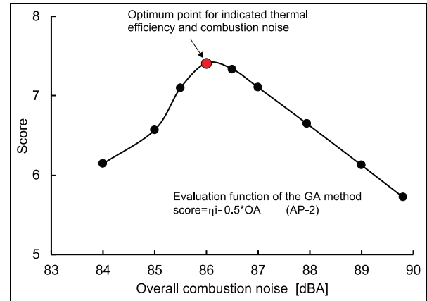
Figure 29. Plots of overall combustion noise versus score (equation (11)).
