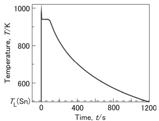
Fig. 10 Cooling curve during cast-in insertion in the case of Fig. 9
