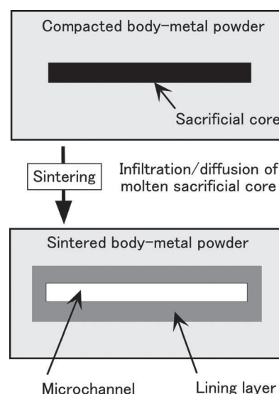
Fig. 1 Powder-metallurgical microchanneling process
