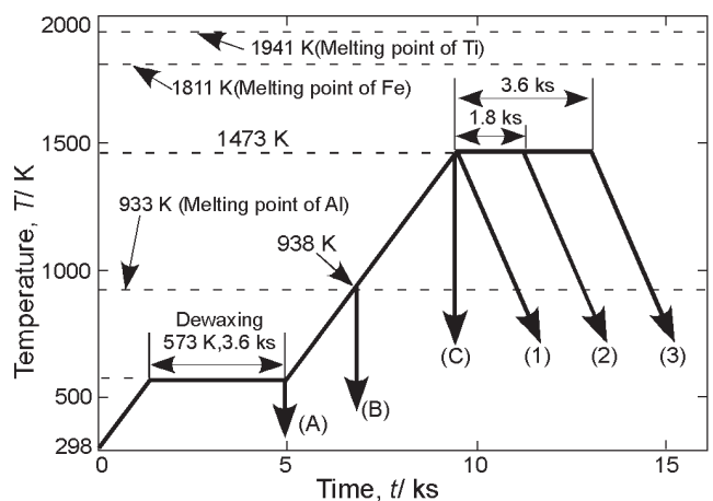
Fig. 3 Heating patterns
