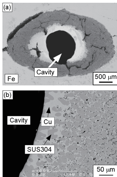
Fig. 10 Back-scattered electron image of a cross section of the Fe/SUS304/Cu specimen (a) and a magnified view of the SUS304-Cu tube body (b)
