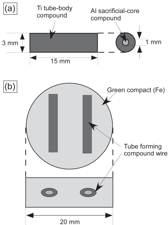
Fig. 2 Schematic illustration of the tube-forming compound (a) and the green compact (b)
