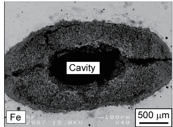
Fig. 11 Back-scattered electron image of a cross-sectional structure of the thin tube in the specimen heat-treated with Pattern (2)
