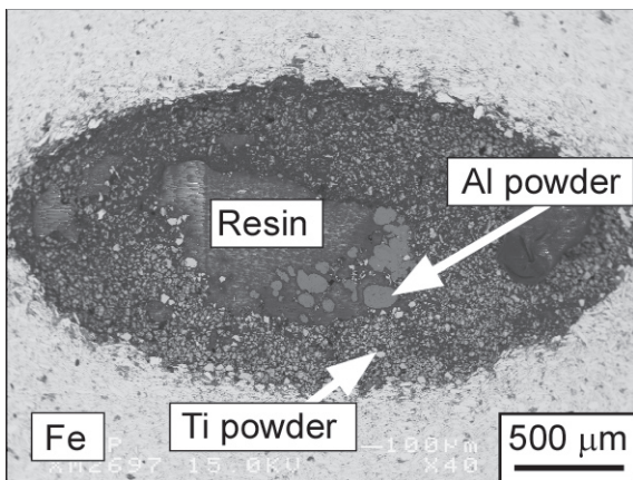
Fig. 7 Back-scattered electron image of a cross-sectional structure of the tube-forming compound wire in the specimen heat-treated with Pattern (A)
