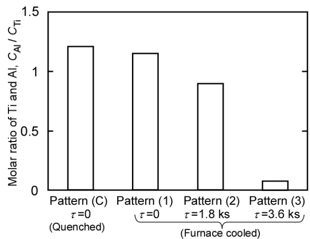
Fig. 13 Relationship between the high-temperature holding time, \tau and the molar ratio of Ti and Al, C_{\text{Al}}/C_{\text{Ti}} near the inner walls of the thin tube
