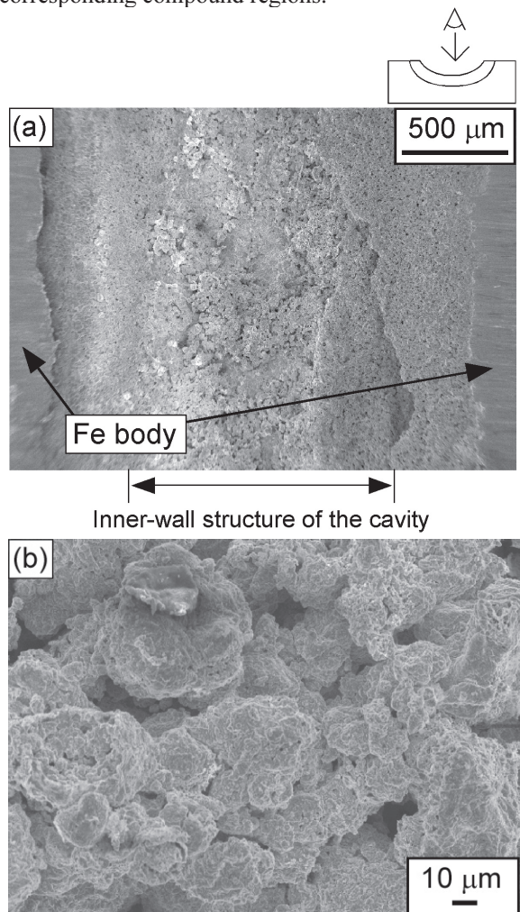
Fig. 5 SEM image of the longitudinal section of the thin tube produced in the specimen heat-treated with Pattern (2) (a) and a magnified view of the inner-wall structure of the cavity (b)
