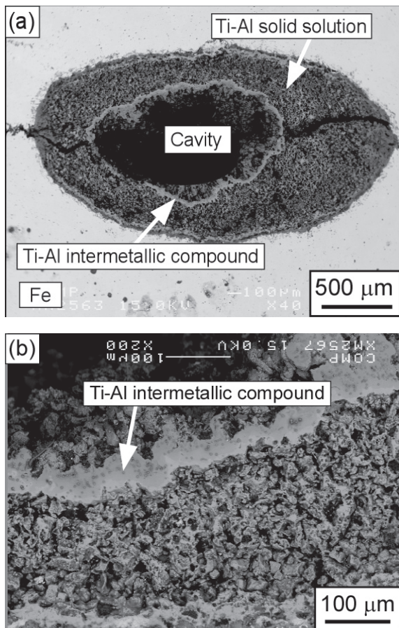
Fig. 4 Back-scattered electron image of a cross-sectional structure of the thin tube in the specimen heat-treated with Pattern (1) (a) and a magnified view of the tube body (b)
