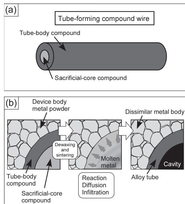
Fig. 1 Constitution of the tube-forming compound wire (a) and schematic representation of the in-situ tube-forming process (b)
