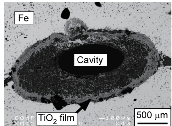
Fig. 12 Back-scattered electron image of a cross-sectional structure of the thin tube in the specimen heat-treated with Pattern (3)
