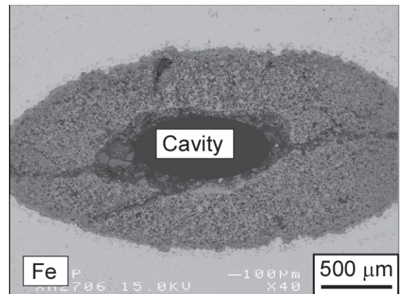
Fig. 9 Back-scattered electron image of a cross-sectional structure of the thin tube in the specimen heat-treated with Pattern (C)
