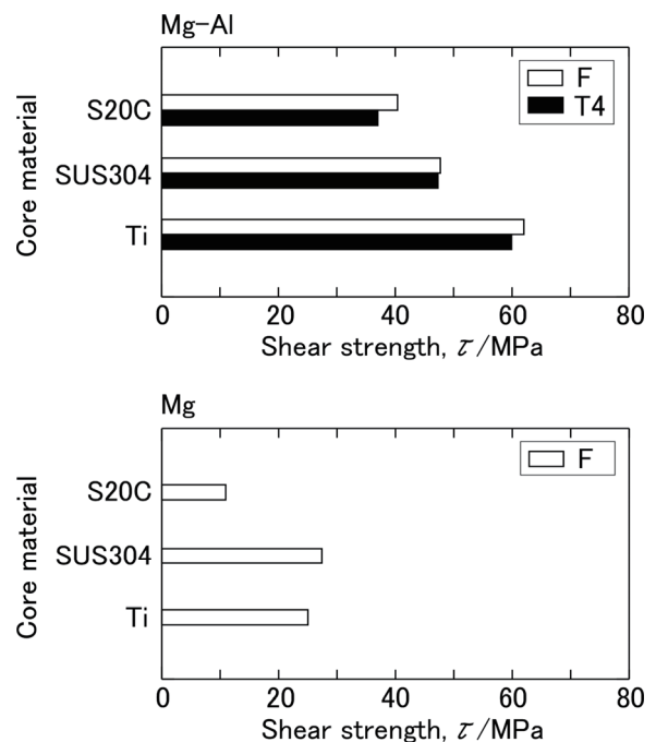
Fig. 4 Results of the Push-out tests
