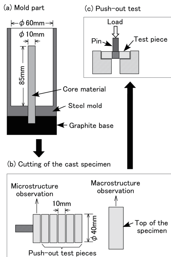
Fig. 1 Experimental procedures. (a) Mold part of the apparatus. (b) Preparation of push-out test pieces and specimens for macro- and microstructure observation. (c) Set up of the jig for the push-out test
