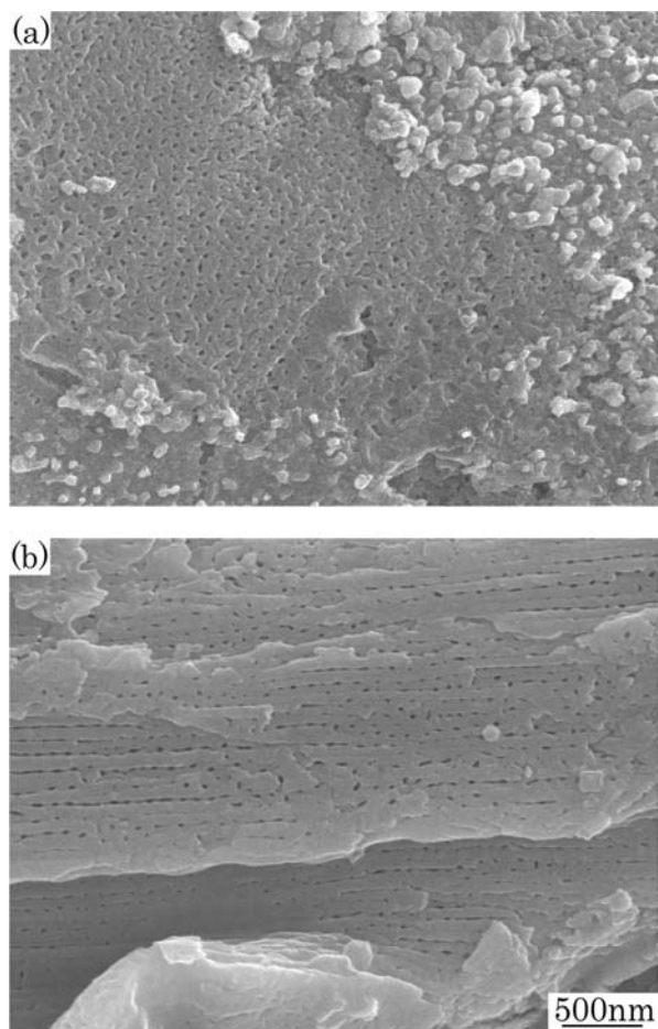
Fig. 5 Surface structures of the specimens after anodic oxidation at 50 V for 7.2 ks. (a) Al-Zn lining layer, (b) comparative specimen
