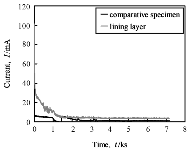
Fig. 4 Change in current with anodizing time at 50V
