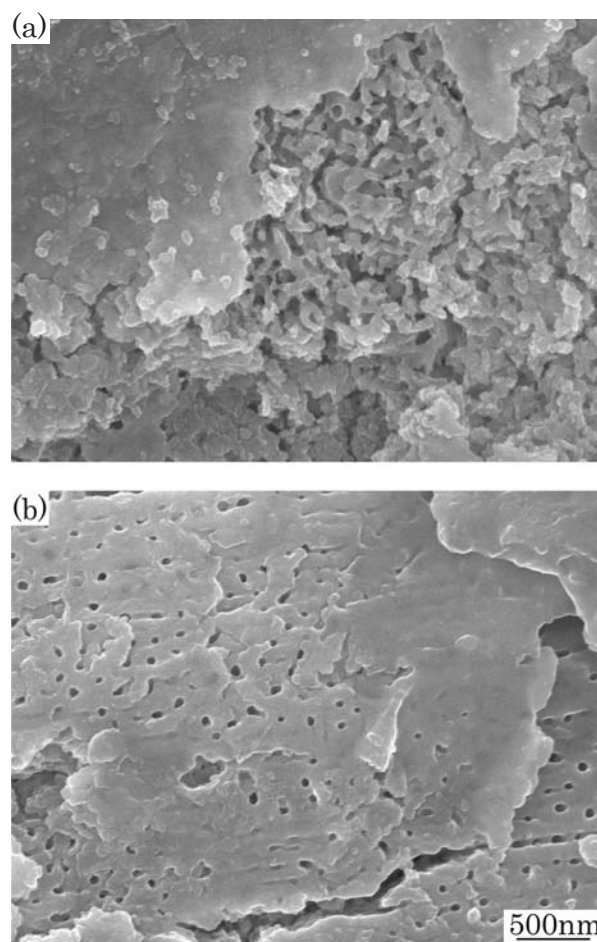
Fig. 6 Surface structures of the specimens after anodic oxidation at 100 V for 7.2 ks. (a) Al-Zn lining layer, (b) comparative specimen
