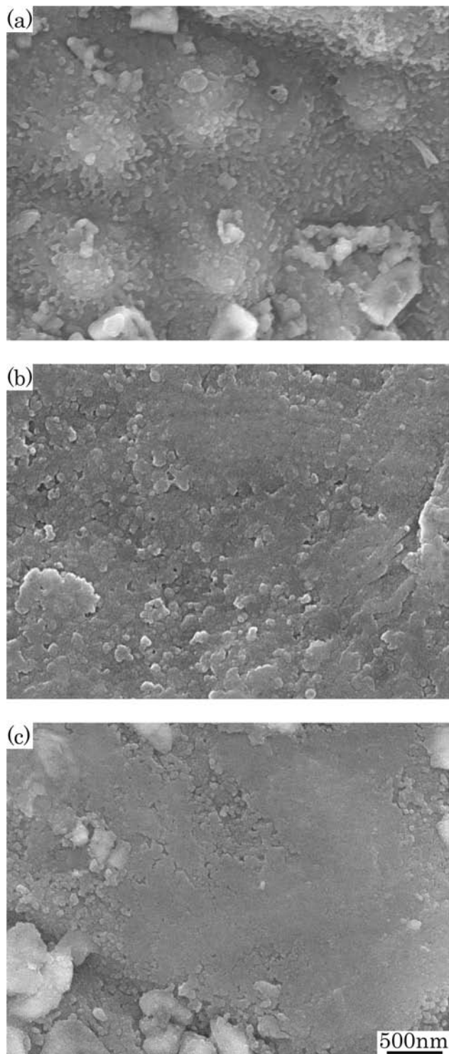
Fig. 2 Surface structures of the Al-Zn lining layers after anodic oxidation at 50 V for 1.8 ks. Compacting pressure: (a) 79.5 MPa, (b) 159 MPa, (c) 318 MPa
