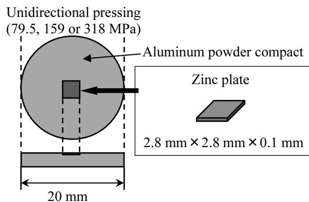
Fig. 1 Preparation of the compact specimen with a plate-like sacrificial core
