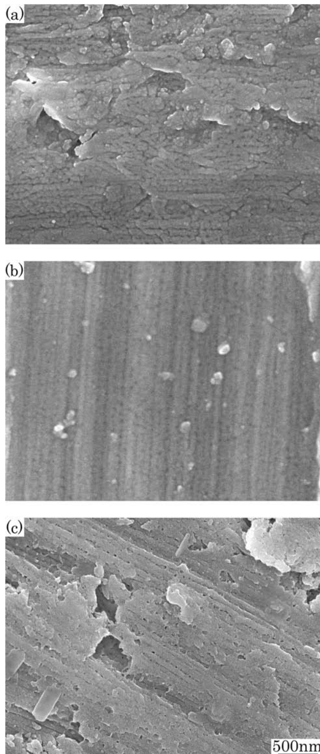
Fig. 3 Surface structures of the comparative specimens after anodic oxidation at 50 V for 1.8 ks. Compacting pressure: (a) 79.5 MPa, (b) 159 MPa, (c) 318 MPa
