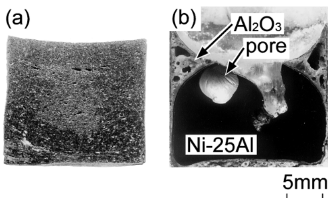
Fig. 3 Longitudinal cross section of Ni-25 mol%Al alloy specimens produced by a thermite-type combustion synthesis in an alumina crucible under 1 G. (a) a=0.23 . (b) a=0.25 .
