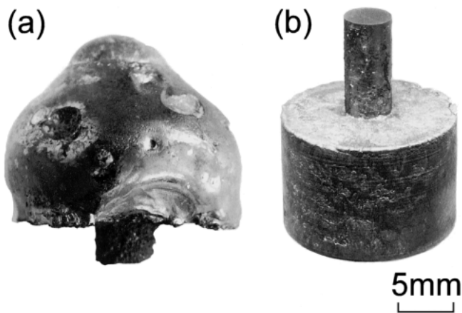
Fig. 4 Ni-25 mol%Al alloy specimens produced by using a graphite mold. (a) Specimen produced under 1 G (Ni-Al alloy that did not flow into the mold cavity). (b) Specimen produced by the centrifugal casting. a=0.25 .
