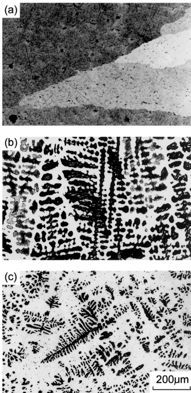
Fig. 7 Microstructures of specimens produced by the centrifugal casting. (a) Ni-50 mol%Al alloy (NiAl). (b) Ni-31 mol%Al alloy (NiAl + Ni 3 Al). (c) Ni-25 mol%Al alloy (NiAl + Ni 3 Al).
