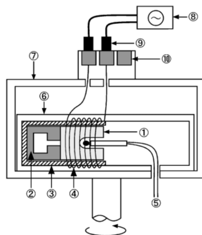
Fig. 1 Schematic illustration of experimental apparatus. ① green compact, ② graphite mold, ③ alumina container, ④ heating coil, ⑤ thermocouple, ⑥ inner steel container, ⑦ outer steel container, ⑧ electric source, ⑨ graphite brush, ⑩ slip ring.
