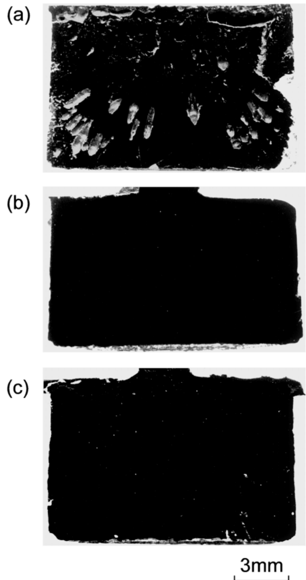
Fig. 6 Longitudinal cross section of centrifugally cast alloys. (a) Ni-50 mol%Al alloy. (b) Ni-31 mol%Al alloy. (c) Ni-25 mol%Al alloy.
