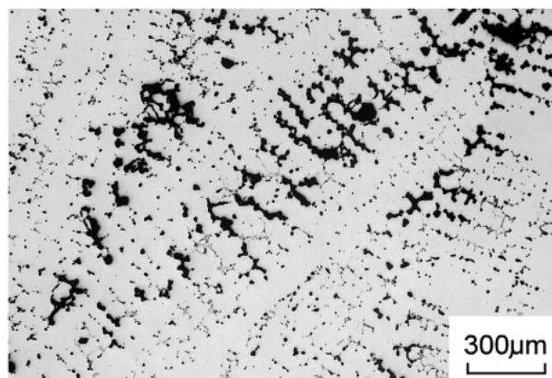
Fig. 8 Micropores formed in the centrifugally cast Ni-37 mol%Al alloy.
