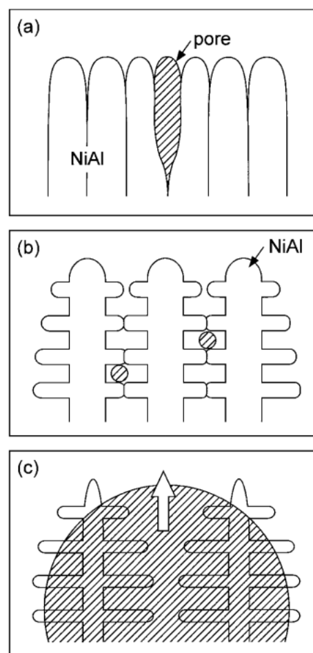
Fig. 9 Formation mechanisms of pores in the centrifugally cast Ni-Al alloys. (a) Ni-50 mol%Al and Ni-43 mol%Al alloys. (b) Ni-37 mol%Al alloy. (c) Ni-31 mol%Al and Ni-25 mol%Al alloys.
