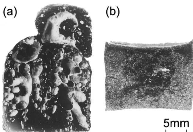
Fig. 2 Longitudinal cross section of Ni-Al alloys produced by a combustion synthesis ( a=0 ) in an alumina crucible under 1 G. (a) Ni-50 mol%Al. (b) Ni-25 mol%Al 12) .
