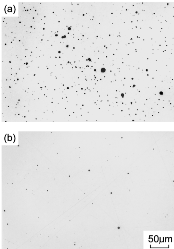
Fig. 5 Distribution of alumina particles in Ni-25 mol%Al alloy specimens. (a) Specimen produced under 1 G. (b) Specimen produced by the centrifugal casting.
