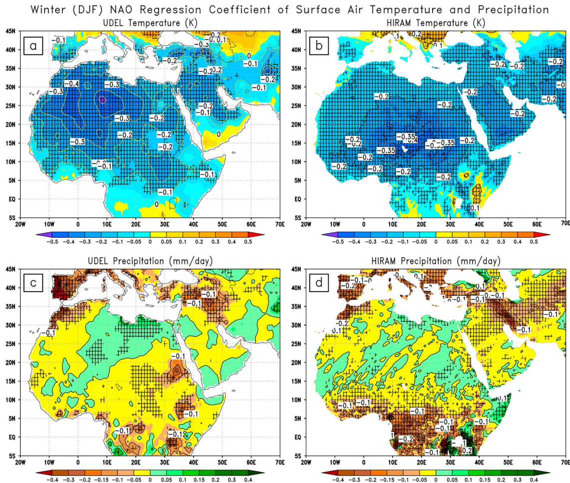
Figure 5. Winter (DJF) NAO regression coefficient with surface air-temperature (K) calculated using (a) UDEL 30-year period and (b) model 30-year period and with precipitation (mm/day) calculated using (c) UDEL 30-year period and (d) model 30-year period. Hatching shows the statistically significant areas with at least 95% confidence level. DJF = December to February; HiRAM = high-resolution atmospheric model; NAO = North Atlantic Oscillation; UDEL = University of Delaware.
