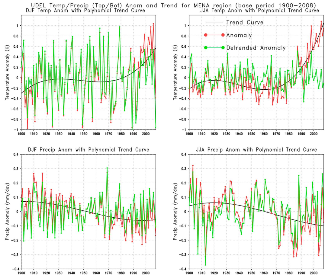
Figure 3. The polynomial trend curve of temperature/precipitation (top/bottom) fields in winter/summer (left/right) computed for MENA region over a longer period of 1900–2008. The anomalies of temperature and precipitation before (red curve) and after removing polynomial trend (green curve) are also shown. DJF = December to February; JJA = June to August; MENA = Middle East and North Africa; UDEL = University of Delaware.
