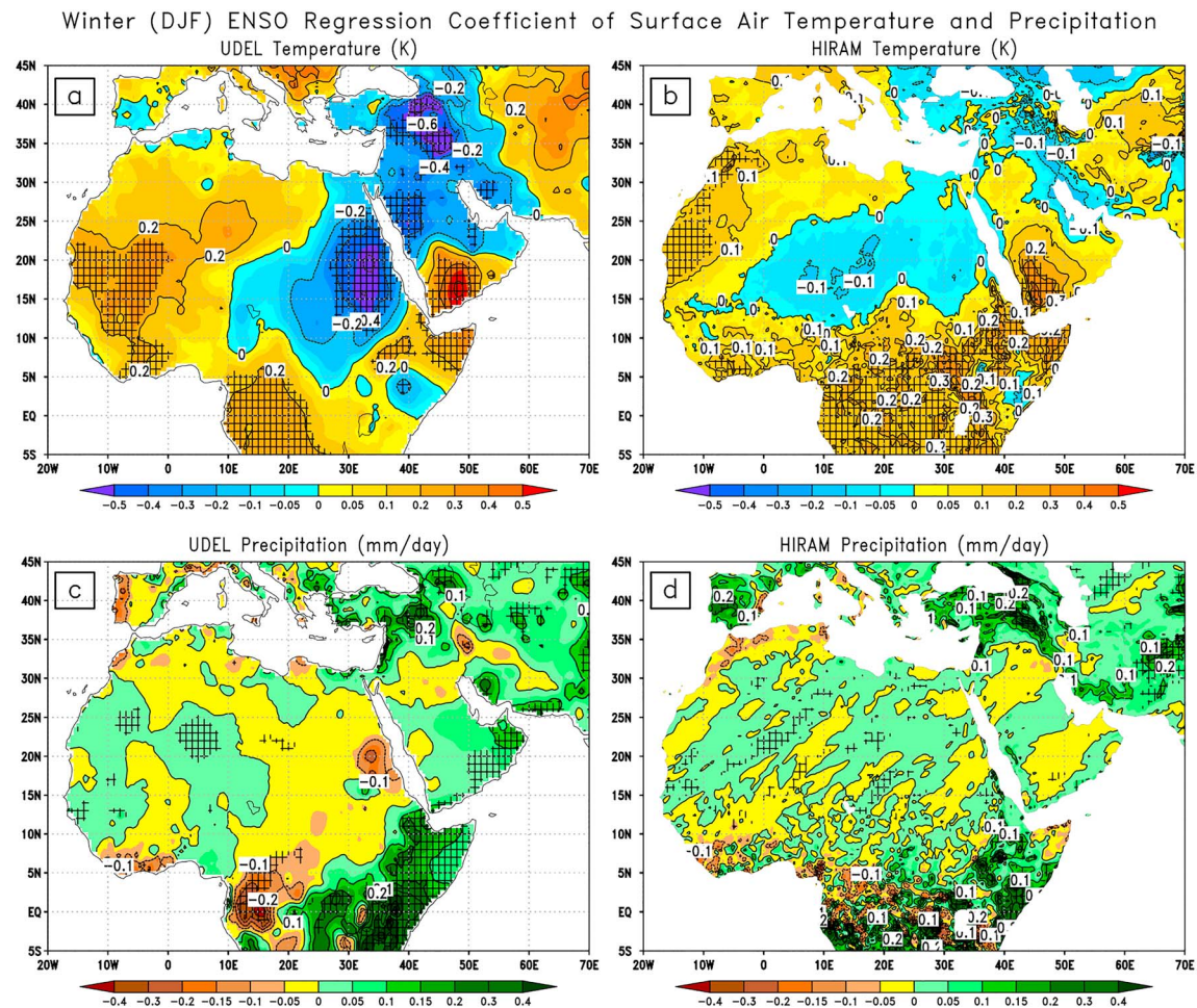
Figure 6. Winter (DJF) ENSO regression coefficient with surface air-temperature (K) calculated using (a) UDEL 30-year period and (b) model 30-year period and with precipitation (mm/day) calculated using (c) UDEL 30-year period and (d) model 30-year period. Hatching shows the statistically significant areas with at least 95% confidence level. DJF = December to February; ENSO = El Niño Southern Oscillation; HIRAM = high-resolution atmospheric model; UDEL = University of Delaware.
