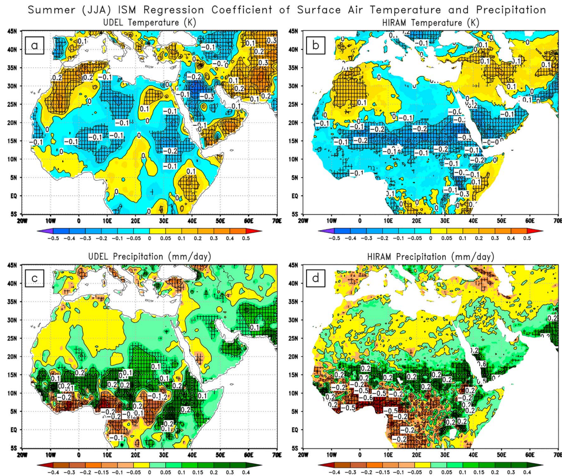
Figure 8. Summer (JJA) ISM regression coefficient of surface air-temperature (K) calculated using (a) UDEL 30-year period and (b) model 30-year period and with precipitation (mm/day) calculated using (c) UDEL 30-year period and (d) model 30-year period. Hatching shows the statistically significant areas with at least 95% confidence level. HIRAM = high-resolution atmospheric model; ISM = Indian summer monsoon; JJA = June to August; UDEL = University of Delaware.
