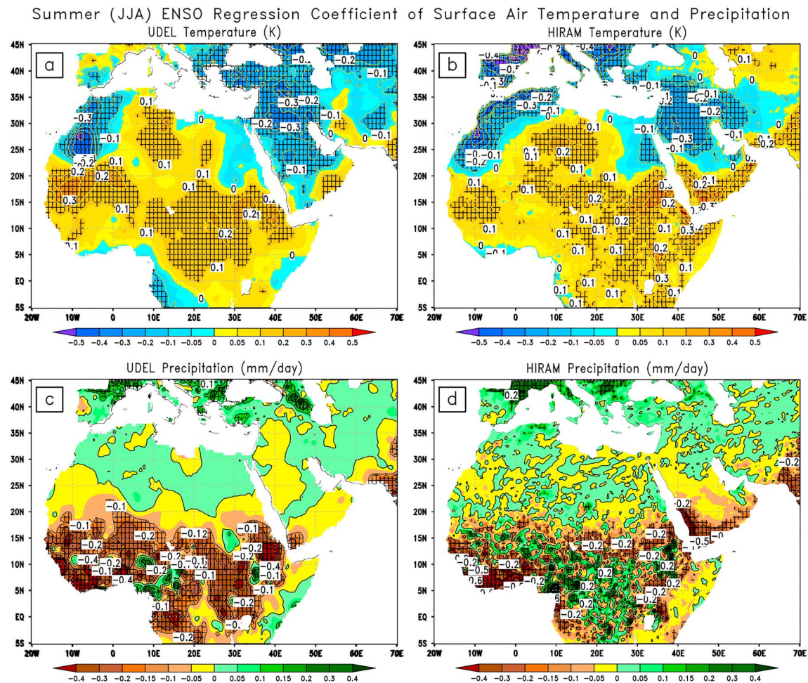
Figure 7. Summer (JJA) ENSO regression coefficient with surface air-temperature (K) calculated using (a) UDEL 30-year period and (b) model 30-year period and with precipitation (mm/day) calculated using (c) UDEL 30-year period and (d) model 30-year period. Hatching shows the statistically significant areas with at least 95% confidence level. ENSO = El Niño Southern Oscillation; HIRAM = high-resolution atmospheric model; JJA = June to August; UDEL = University of Delaware.
