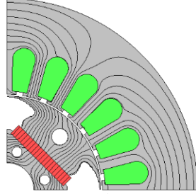
Fig. 11. Shape of motor B in the pareto front shown in Fig.8 T_{ave} = 2.02\text{ Nm} , T_{rip} = 0.074
