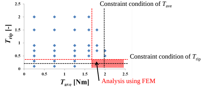
Fig. 7. Domain for execution of FE analysis
