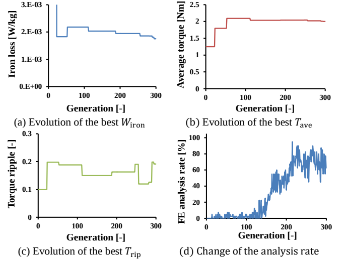
Fig. 14. Evolution of the best values and change of the analysis rate
