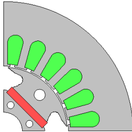
Fig. 2. IPM motor obtained by preliminary optimization
