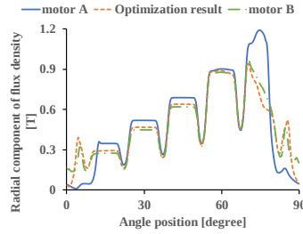
Fig. 13. Radial component of flux density along the midline of the air-gap
