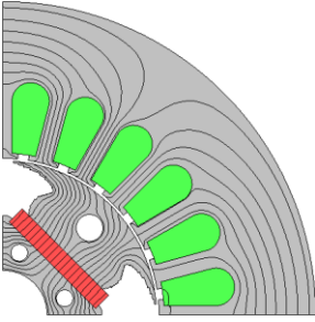
Fig. 12. Optimization result obtained by method (ii). W_{iron} = 1.75 \times 10^{-3} , T_{ave} = 2.00\text{Nm} , T_{rip} = 0.191
