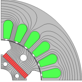
Fig. 10. Shape of motor A in the pareto front shown in Fig.8 T_{ave} = 2.21\text{Nm} , T_{rip} = 0.700
