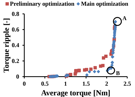
Fig. 8. Comparison of Pareto solutions obtained by method (i)
