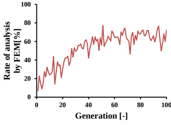
Fig. 9. Rate of FEM evaluations
