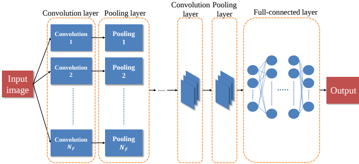
Fig. 1 Structure of CNN
