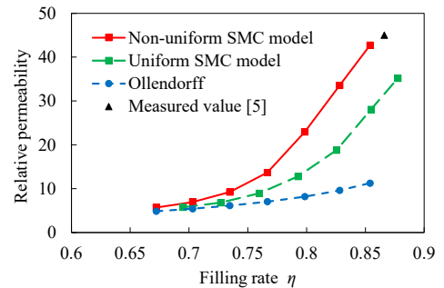
Fig. 7. Dependence of macroscopic permeability of SMC on filling rate
