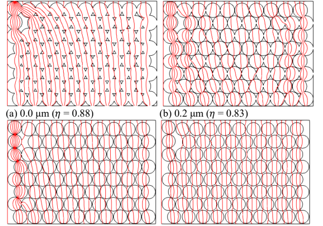
Fig. 6. Flux lines for uniform particles with various insulation thickness
