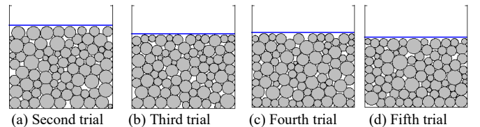
(a) Second trial (b) Third trial (c) Fourth trial (d) Fifth trial Fig. 2. Modeling results starting from different states
