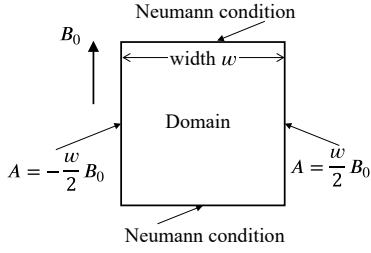
Fig. 3. Boundary condition
