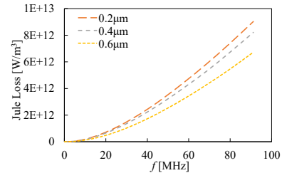
Fig. 10. Joule loss for different insulating thickness
