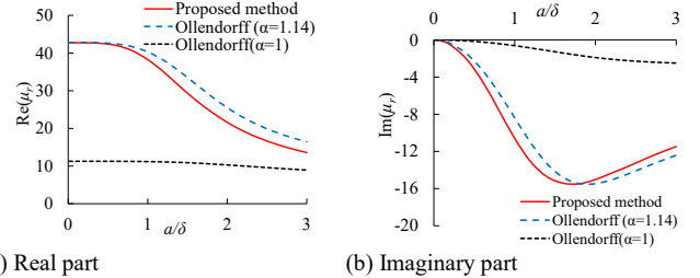
(a) Real part (b) Imaginary part Fig. 11. Accuracy of modified Ollendorff formula considering contact
