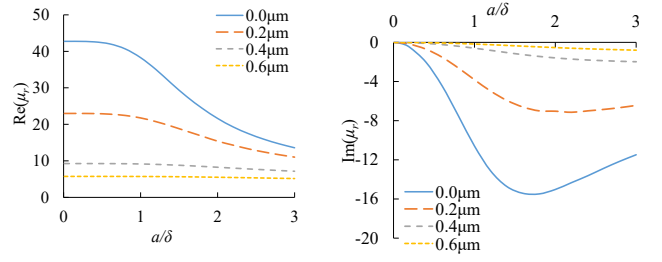
(a) Real part (b) Imaginary part Fig. 8. Frequency characteristic of macroscopic complex permeability for different insulating thickness
