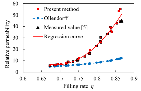
Fig. 5. Dependence of macroscopic permeability of SMC on filling rate
