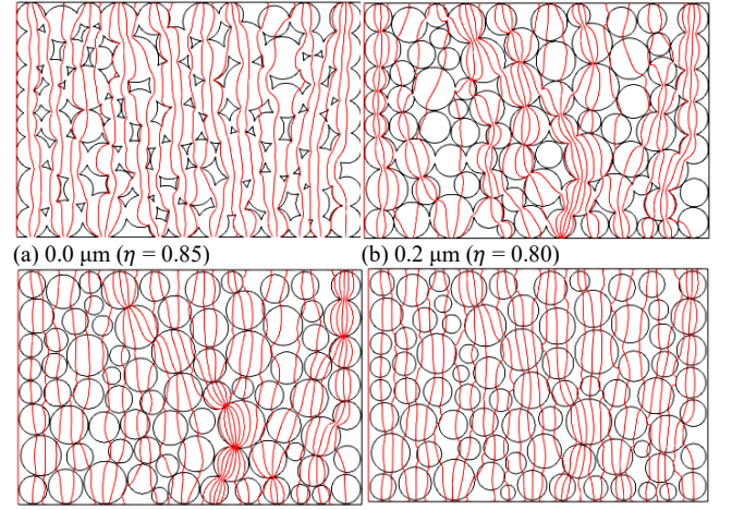
Fig. 4. Flux lines for non-uniform particles with various insulation thickness
