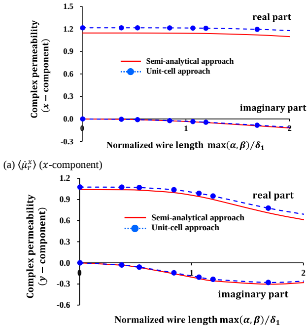
(a) \langle \mu_r^x \rangle (x-component)
