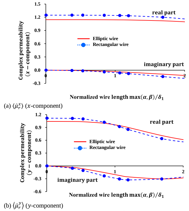
(b) \langle \mu_r^y \rangle (y-component)
