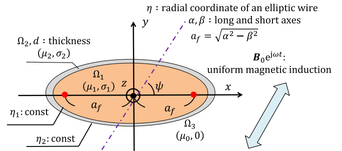
Fig.1 Magnetically shielded wire (MSW) with elliptic cross section immersed in time-harmonic magnetic induction B_0 e^{j\omega t} .
