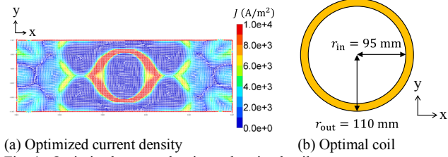
Fig. 4. Optimized current density and optimal coil
