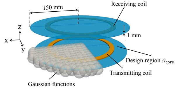
Fig. 6. Optimization model for magnetic core design
