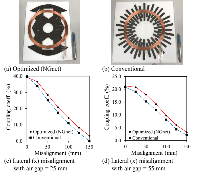
Fig. 10. Manufactured WPTs and measured coupling coefficients
