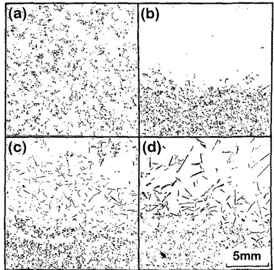
Fig. 5 Formation process of the fine-coarse transition region of the double composite layer. (a) bath-cooled just after the injection, (b) bath-cooled at 953 K, (c) bath-cooled at 934 K, and (d) furnace-cooled until complete solidification. The jet melt is Al-5 mass % Cr alloy.
