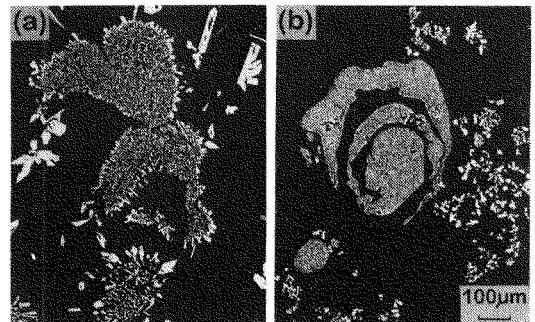
Fig. 6 Clusters of fine intermetallic compound particles observed at 10 mm-height of the samples bath-cooled just after the injection of (a) Al-5 mass % Cr and (b) Al-10 mass % Cr.
