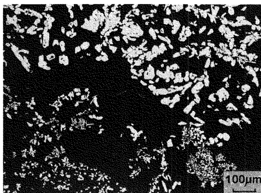
Fig. 3 Microstructure of fine-coarse transition region of the double composite layer in the furnace-cooled sample produced by Injection Quenching with the jet melt of Al-10 mass % Cr alloy.
