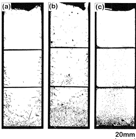
Fig. 2 Macrostructures of vertical cross section of ingots. (a) furnace-cooled Al-1.25 mass % Cr alloy ingot by conventional casting, (b) furnace-cooled ingot produced by Injection Quenching with the jet melt of Al-5 mass % Cr alloy, (c) ingot bath-cooled just after the injection of Al-5 mass % Cr alloy.
