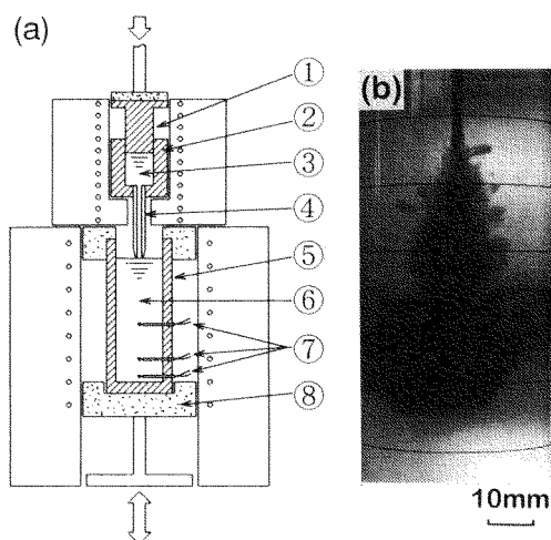
Fig. 1 Experimental apparatus (a), and flow pattern of water jet (b). ① graphite piston ② graphite cylinder ③ jet melt ④ nozzle ⑤ graphite mold ⑥ bulk melt ⑦ thermocouples ⑧ movable stage
