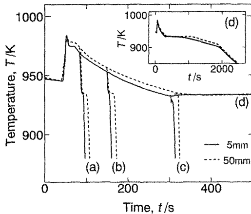
Fig. 4 Time-temperature curves measured during Injection Quenching and furnace-/bath-cooling. The jet melt is Al-5 mass % Cr alloy in each experiment. (a) bath-cooled just after the injection of the jet melt, (b) bath-cooled when the temperature at the position of 5 mm in height was 953 K, (c) bath-cooled when the temperature of the 5 mm-high position was 934 K, and (d) furnace-cooled until complete solidification.
