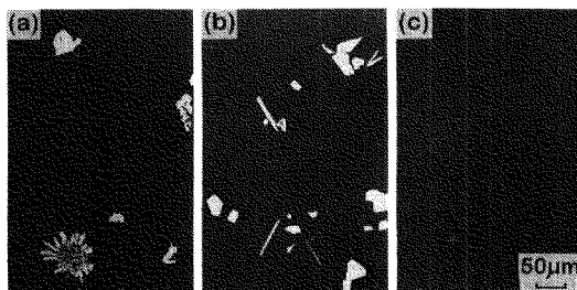
Fig. 7 Sequence of sedimentation of intermetallic compound particles at the 100 mm-high position of the samples produced by Injection Quenching with the jet melt of Al-10 mass % Cr alloy, and (a) bath-cooled just after the injection, (b) bath-cooled at 963 K, and (c) bath-cooled at 933 K.
