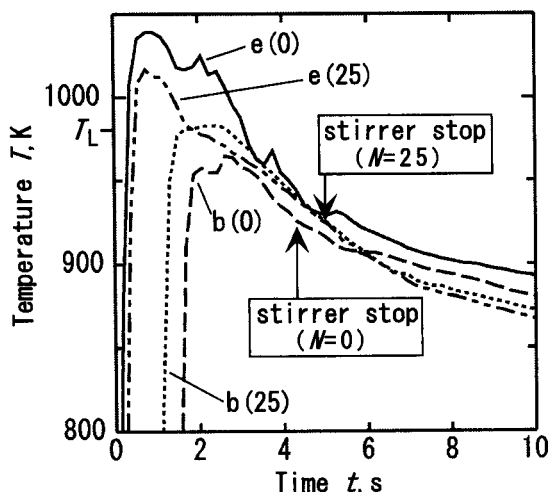
Fig. 6 Cooling curves measured during the single-casting experiments with the stirring conditions of N=0\text{ s}^{-1} and N=25\text{ s}^{-1} . In the figure, “b” and “e” denote the measuring points shown in Fig. 2.
