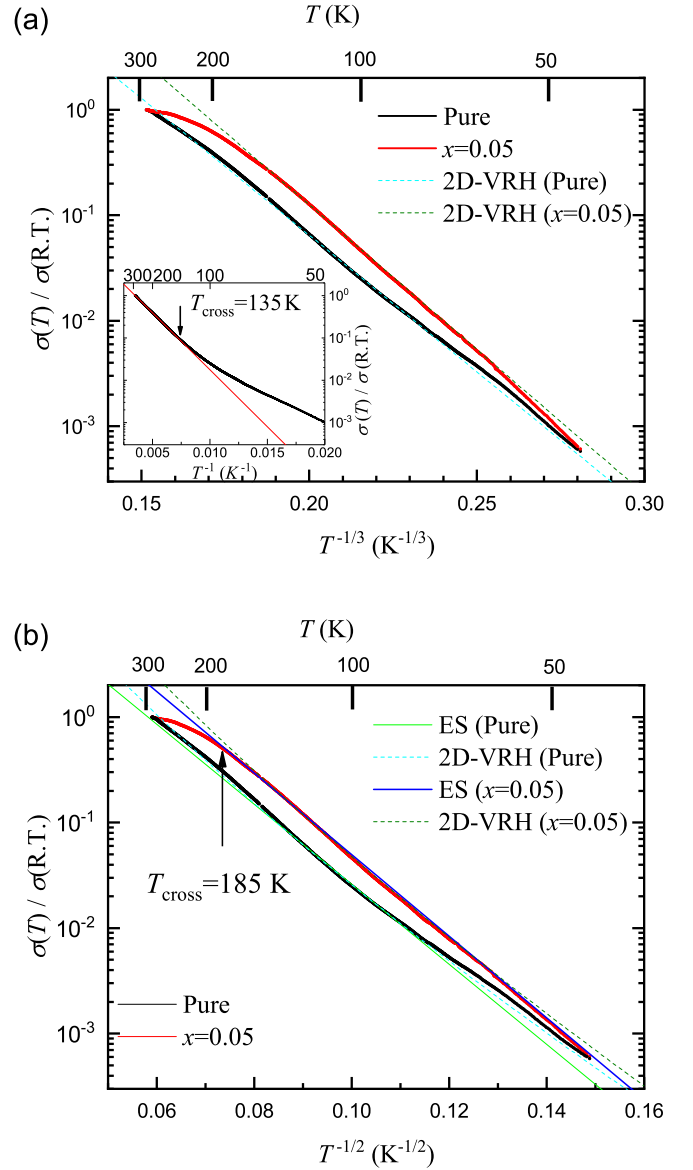
FIG. 3. Normalized conductivity of pure and x = 0.05 samples as a function of (a) T^{-1/3} and (b) T^{-1/2} . The solid (dashed) line shows the fit given by the ES (2D-VRH) model. Inset in (a) shows Arrhenius plot of the pure sample and the solid line shows the fit given by the NNH model.
