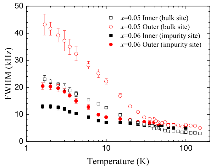
FIG. 12. FWHM of NMR line for impurity and bulk sites as a function of temperature.
