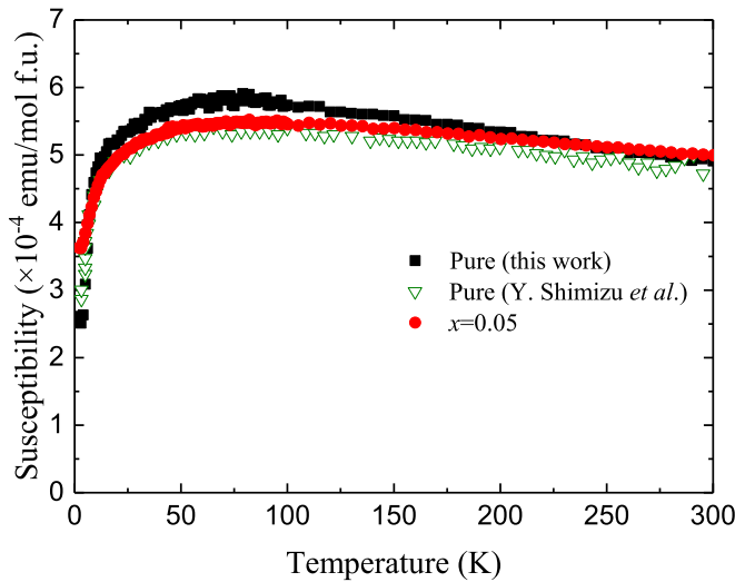
FIG. 4. Magnetic susceptibility as a function of temperature for pure and x = 0.05 samples. The data of one of the pure samples indicated by the inverted triangle are taken from Ref. [3].
