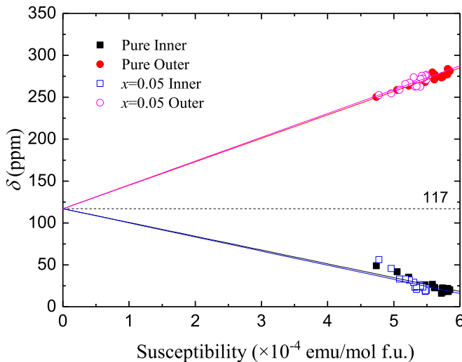
FIG. 7. Temperature dependence of \delta - \chi plot.
