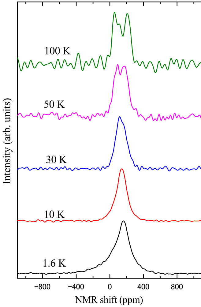
FIG. 10. NMR spectra of impurity sites at several temperatures.
