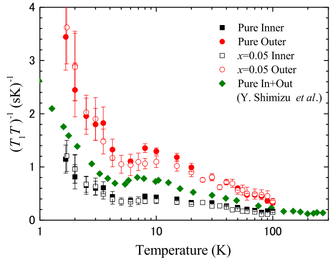
FIG. 9. Temperature dependence of (T_1 T)^{-1} for the pure and x = 0.05 samples. The data of one of the pure samples indicated by the rhombus represents an average of the inner and outer sites and are taken from Ref. [19].
