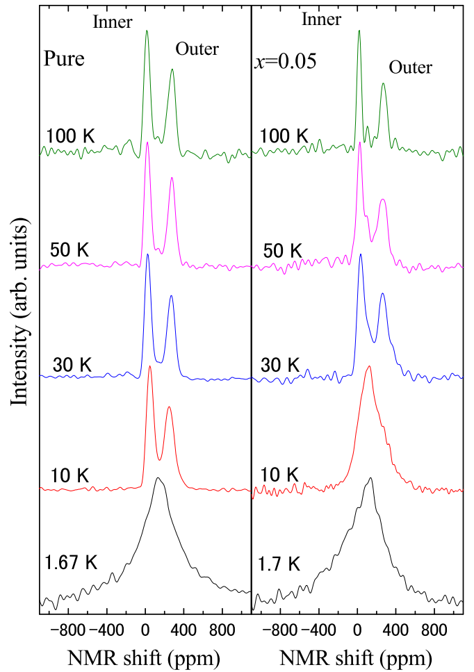
FIG. 5. NMR spectra at several temperatures in a field of H \parallel a^* . Left (right) panel shows the results for the pure ( x = 0.05 ) sample.
