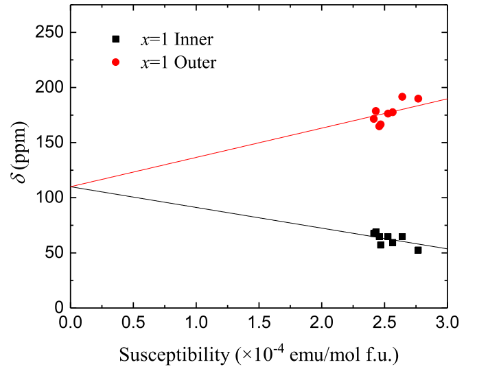
FIG. 11. Temperature dependence of \delta - \chi plot for the x = 1 sample.
