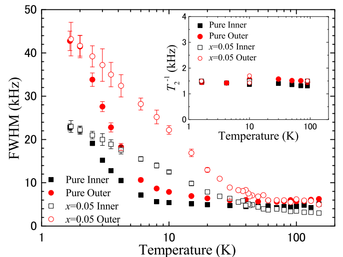
FIG. 8. Temperature dependence of FWHM of NMR lines. Inset shows temperature dependence of T_2^{-1} .
