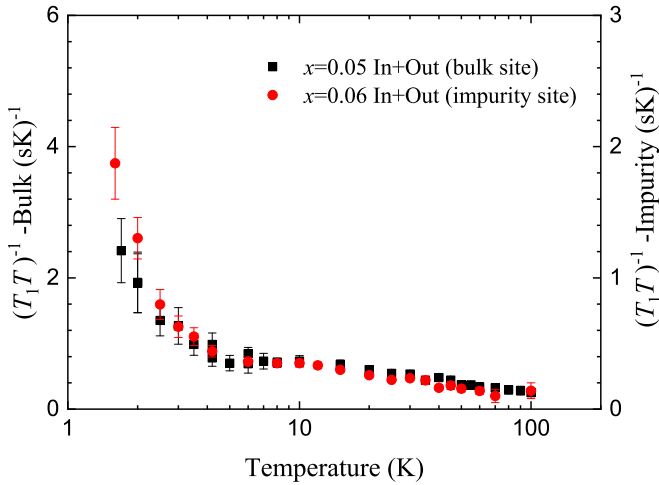
FIG. 13. Temperature dependence of the mean value of (T_1 T)^{-1} of the associated inner and outer sites for bulk and impurity sites. The results of the bulk site are plotted with the left axis, and the results of the impurity site are plotted with the right axis.
