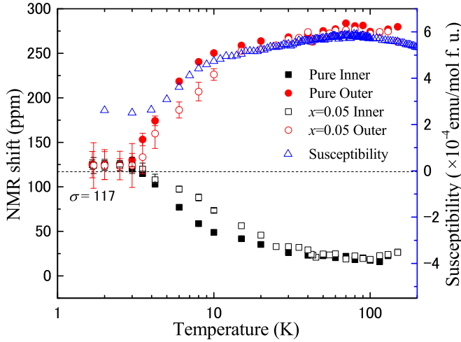
FIG. 6. NMR line shift and magnetic susceptibility as a function of temperature.
