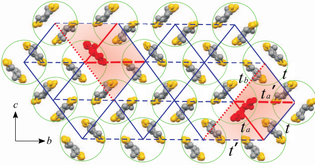
FIG. 2. Schematic view of BEDT-TTF dimers in the bc plane. Red molecules represent BEDT-STF molecules. Original nearly isotropic and modified triangular lattices are shown by blue and red lines, respectively, where t and t' are the original transfer integrals and t_a , t'_a , and t_b are the transfer integrals around the BEDT-STF molecule.
