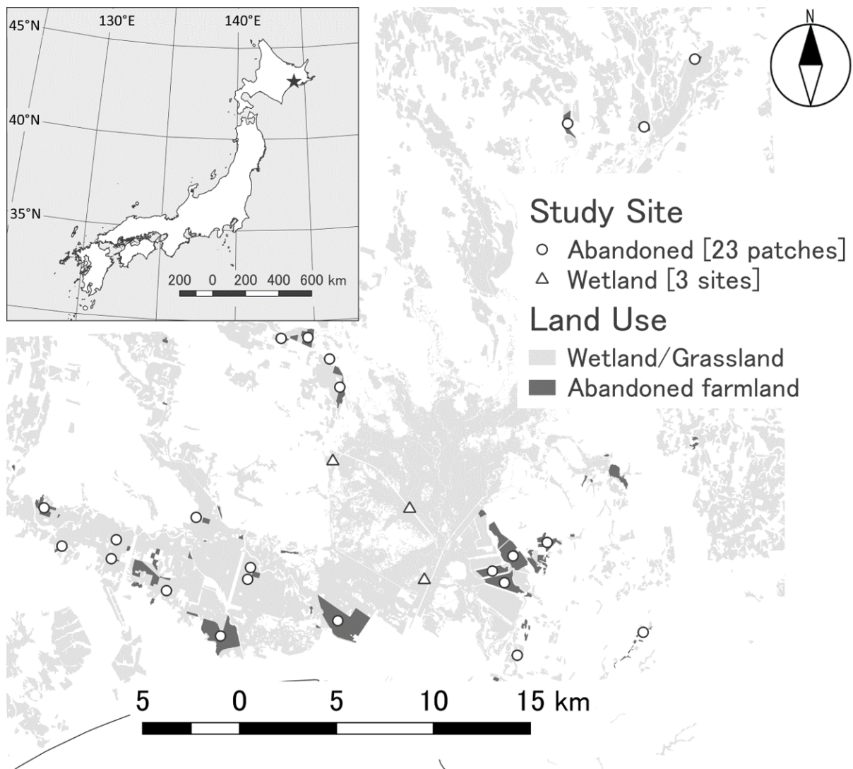
Fig. 1. Study area.
