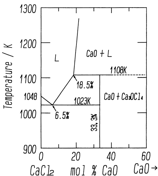
Fig. 4. Phase diagram of the \text{CaCl}_2 -CaO system 16) .
