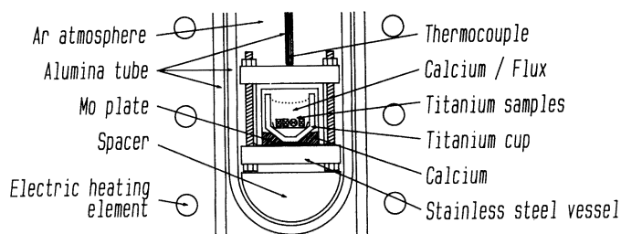
Fig. 5. Schematic illustration of the experimental apparatus.
