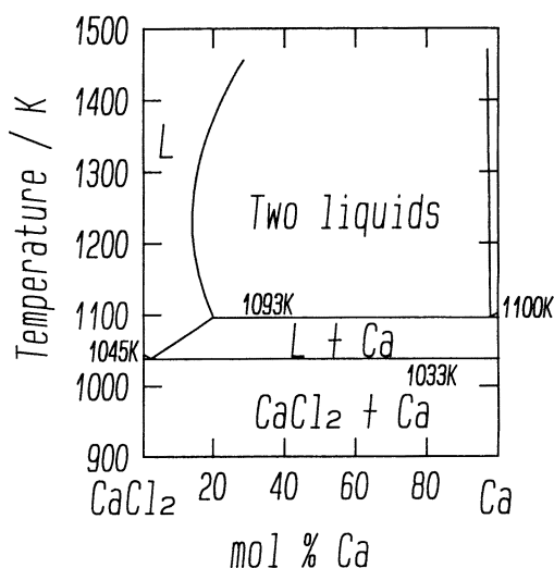
Fig. 3. Phase diagram of the Ca-CaCl 2 system 15) .
