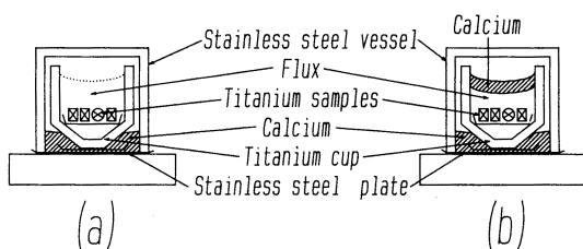
Fig. 6. Reaction vessel arrangement.
