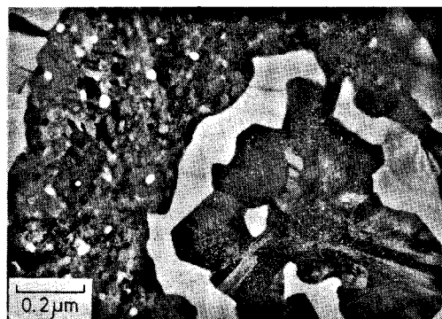
Photo. 5. Phase transformation of metastable phase into stable Al and Ge crystals in \text{Al}_{50}\text{Ge}_{50} alloy.
