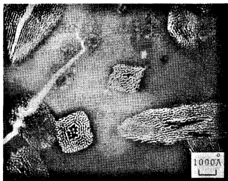
Photo. 3. Cooperative growth of bcc crystal and metastable compound \text{Fe}_3\text{P} in \text{Fe}_{77}\text{P}_{15}\text{C}_8 alloy.
