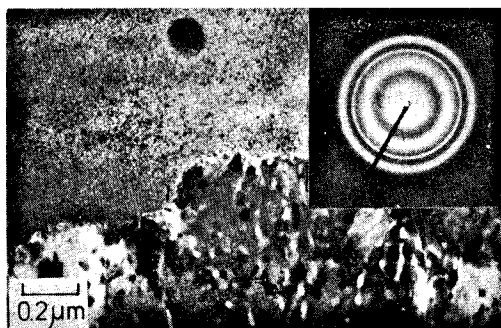
Photo. 4. Growth of metastable phase into the fine grain super-saturated solid solution phase in \text{Al}_{50}\text{Ge}_{50} alloy (aged at room temperature).
