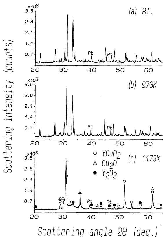
Fig. 2 X-ray diffraction patterns in the sequence of heating \text{Y}_2\text{Cu}_2\text{O}_5 on Pt plate in helium gas. The patterns (a) to (c) were measured at room temperature, 973 K and 1173 K, respectively. (a) and (b) were assigned as the single phase of \text{Y}_2\text{Cu}_2\text{O}_5 .
