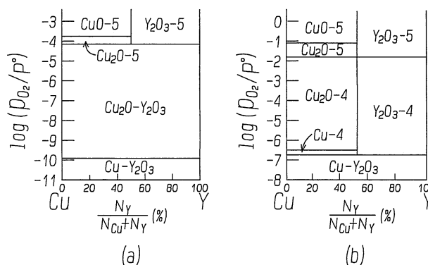
Fig. 6 Oxygen partial pressures as a function of metallic ratio of Y and Cu at 1000 K (a) and at 1250 K (b), where \text{Y}_2\text{Cu}_2\text{O}_5 and \text{YCuO}_2 are referred to as "5" and "4", respectively.
