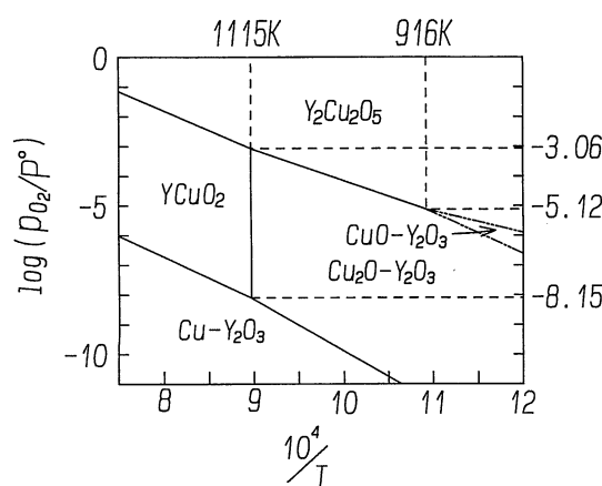
Fig. 7 Oxygen partial pressure of \text{Y}_2\text{Cu}_2\text{O}_5 and \text{YCuO}_2 at the metallic ratio of Y/Cu = 1.
