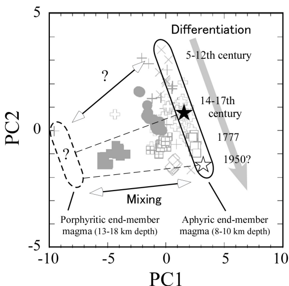
FIGURE 10 | Compositional data of the basaltic samples in a PC2-PC1 diagram, showing the inferred magmatic processes: mixing of phenocryst-rich magmas derived from the 13–18 km-deep magma chamber and phenocryst-free magmas stored in the 8–10 km-deep magma chamber.
