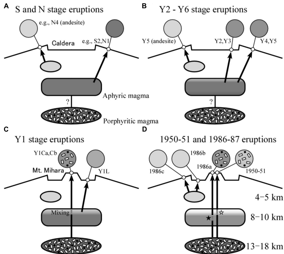
FIGURE 11 | Illustrations of the magma plumbing system of the Izu-Oshima volcano for (A) S and N stage eruptions, (B) Y2–Y6 stage eruptions, (C) Y1 stage eruptions, and (D) 1950–51 and 1986–87 eruptions.
