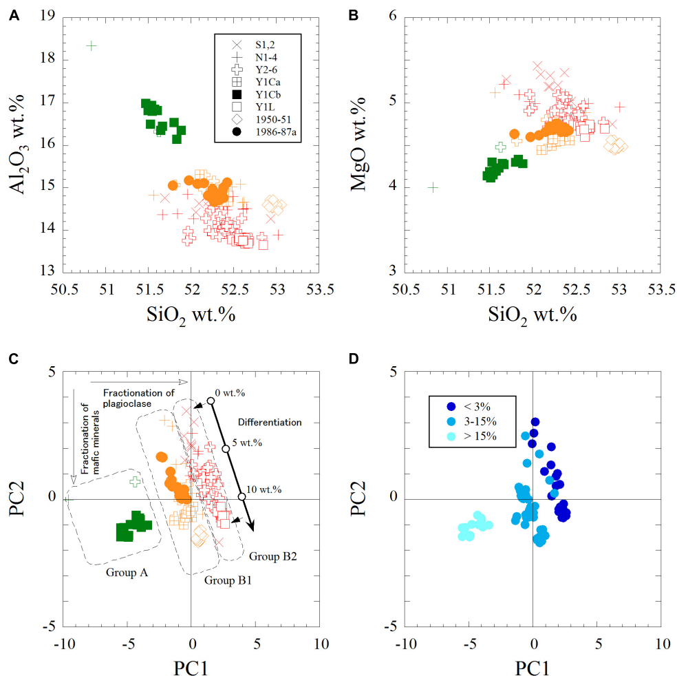
FIGURE 8 | Compositional data of the basaltic samples in (A) \text{Al}_2\text{O}_3 – \text{SiO}_2 , (B) \text{MgO} – \text{SiO}_2 , and (C,D) PC2–PC1 diagrams. The plots in green, orange, and red in (A–C) indicate those belonging to Groups A, B1, and B2, respectively. In panel (C), the result of the crystal fractional modeling for the Group-B2 aphyric samples is shown. In panel (D), the phenocryst contents of the samples investigated in this study are shown in different colors.
