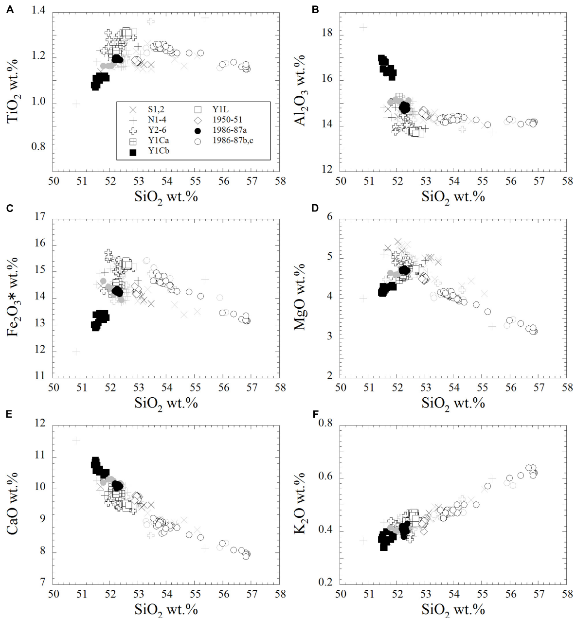
FIGURE 5 | \text{SiO}_2 variation diagrams for (A) \text{TiO}_2 , (B) \text{Al}_2\text{O}_3 , (C) \text{Fe}_2\text{O}_3^* , (D) \text{MgO} , (E) \text{CaO} , and (F) \text{K}_2\text{O} measured in samples from the Younger Oshima Group. Data other than those obtained in this study are taken from Fujii et al. (1988), Kawanabe (1991, 1998), and Ishizuka et al. (2015), and they are shown in gray.
