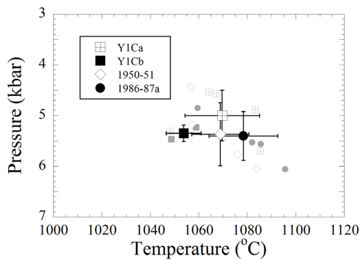
FIGURE 9 | The estimated crystallization pressures and temperatures for pyroxene phenocrysts in products from recent eruptions. The estimates of the individual opx-cpx pairs are represented by the gray plots and the averages with 1\sigma bars of each stage are represented by the black plots.
