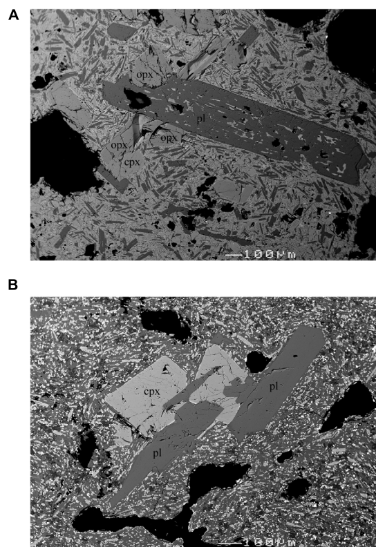
FIGURE 2 | Back-scattered electron images (BEI) of crystal aggregates consisting of plagioclase and pyroxene phenocrysts in (A) 1950–51 and (B) 1986–87a products. “pl,” “opx,” and “cpx” indicate plagioclase, orthopyroxene, and clinopyroxene, respectively.
