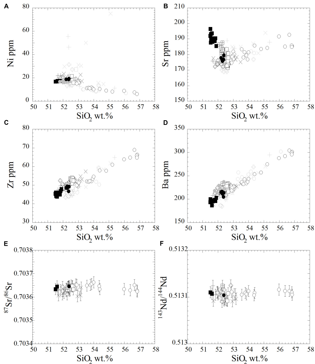
FIGURE 6 | \text{SiO}_2 variation diagrams for (A) Ni, (B) Sr, (C) Zr, (D) Ba, (E) ^{87}\text{Sr}/^{86}\text{Sr} , and (F) ^{143}\text{Nd}/^{144}\text{Nd} measured in samples from the Younger Oshima Group. Data other than those obtained in this study are taken from Ishizuka et al. (2015). The sample symbols are identical to those used in Figure 5.
