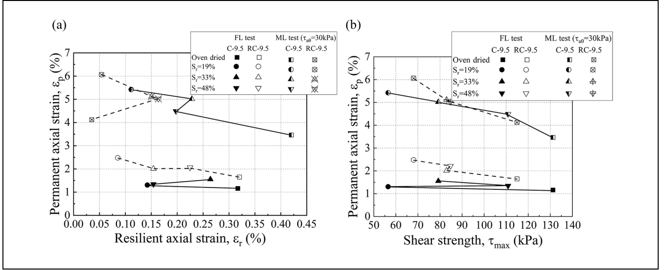
Figure 2. Relations between permanent axial strain and (a) resilient axial strain and (b) shear strength.
