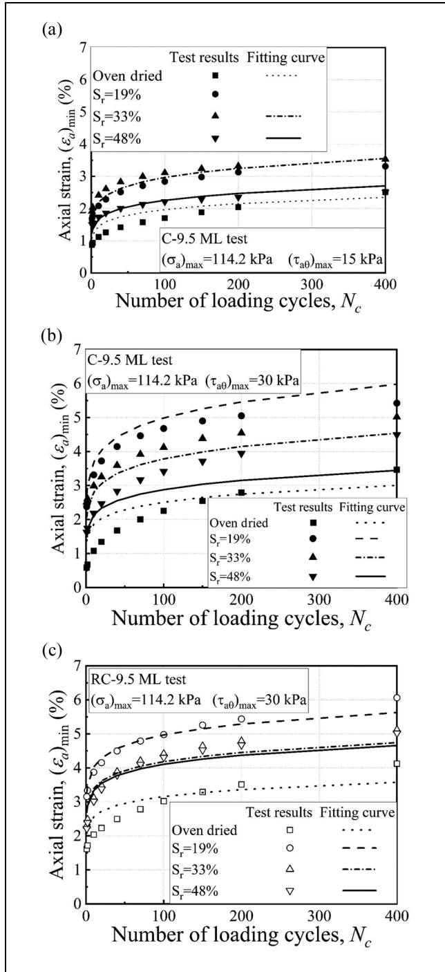
Figure 6. Estimation of the permanent strain of C-9.5 and RC-9.5 with fixed A, B, C, D, showing (a) C-9.5 in ML test ( [\tau_{a\theta}]_{max} = 15 kPa), (b) C-9.5 in ML test ( [\tau_{a\theta}]_{max} = 30 kPa), and (c) RC-9.5 in ML test.
