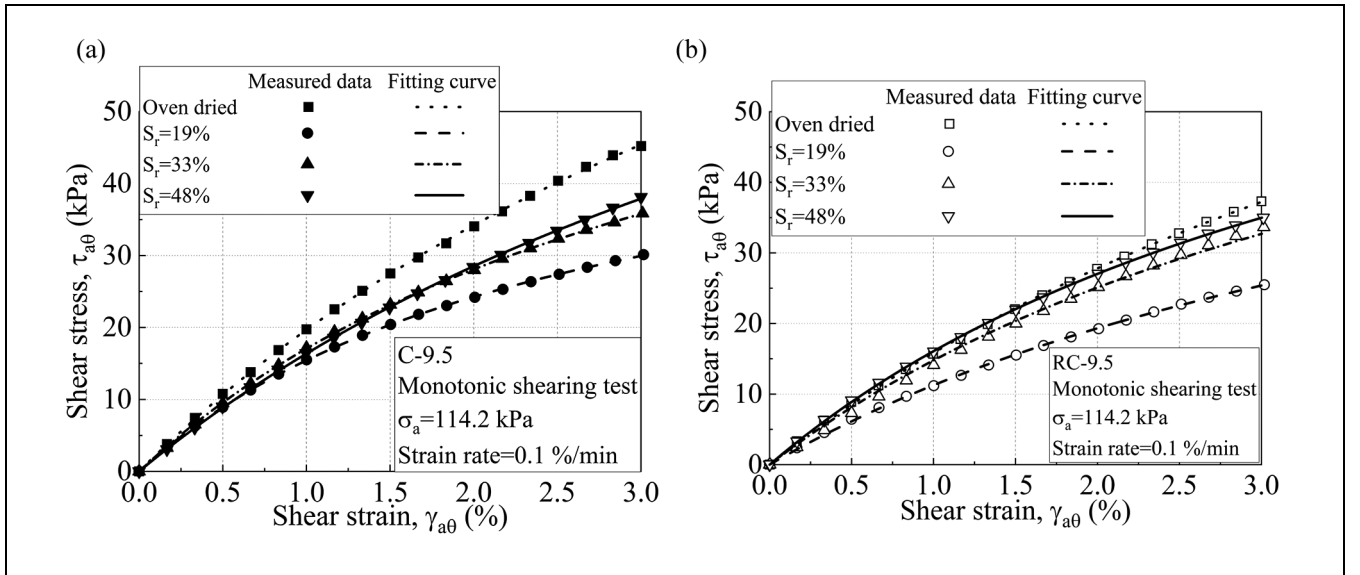
Figure 3. Shear stress-strain curve in monotonic shearing test for (a) C-95 and (b) RC-95.
