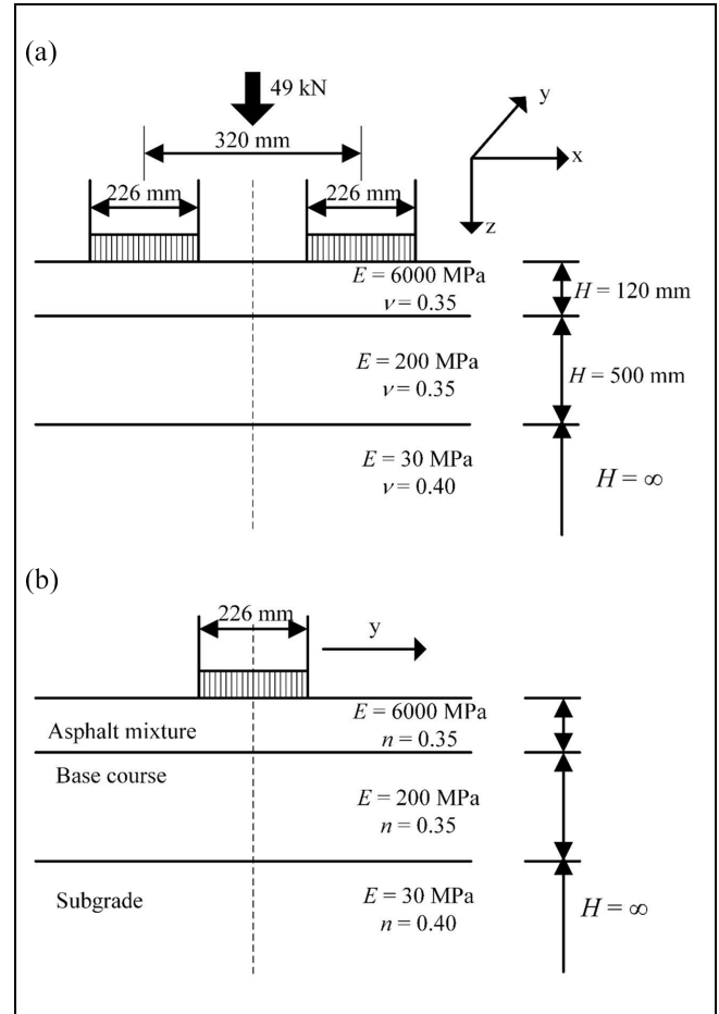
Figure 7. Model for stress analysis, showing (a) cross section and (b) longitudinal section.
