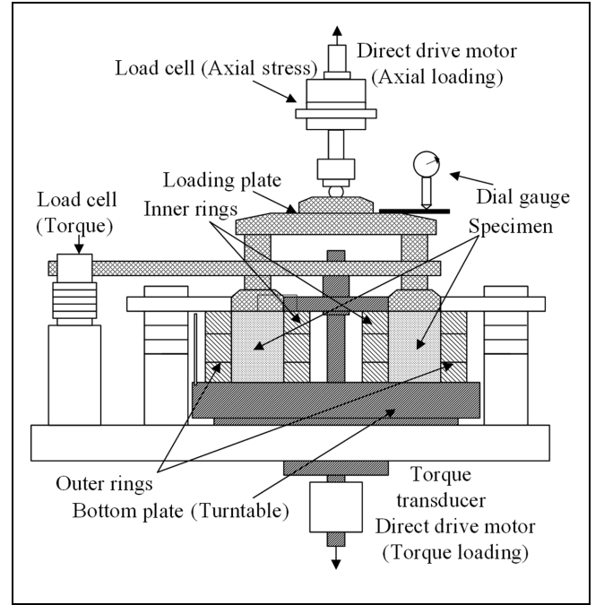
Figure 1. Multi-ring shear apparatus (after Ishikawa et al. 15).
