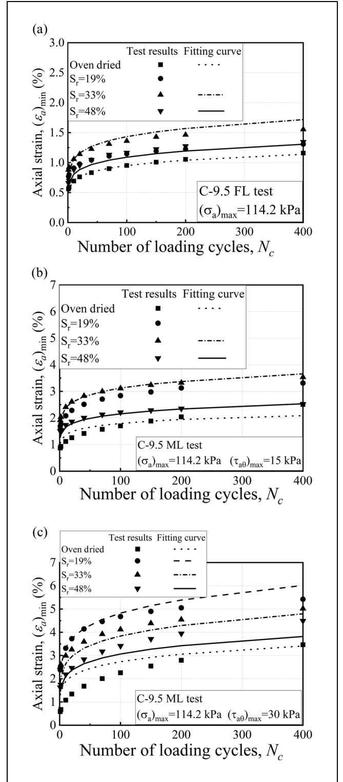
Figure 4. Estimation of permanent axial strain of C-9.5 for (a) FL test, (b) ML test ( [\tau_{a\theta}]_{\max} = 15 kPa), and (c) ML test ( [\tau_{a\theta}]_{\max} = 30 kPa).
