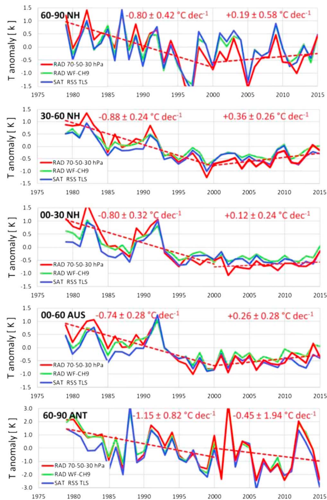
Figure 6. Annual mean temperature anomalies in the lower stratosphere for the period 1979–2015. Time series are radiosonde measurements averaged over the 70, 50, and 30 hPa pressure levels (~18.4- to ~23.8-km altitude; red), radiosonde profiles weighted with the TLS (channel 9) weighting function (green), and satellite observations at the TLS level (blue). Data are shown for 60–90 NH (10 Sta.), 30–60 NH (29 Sta.), 0–30 NH (13 Sta.), 0–60 AUS (4 Sta.), and 60–90 ANT (4 Sta.). Trend lines and trend values with their respective \pm 2\sigma standard errors are given for the radiosonde 70, 50, and 30 hPa levels for the periods 1979–2000 and 2000–2015 (red broken lines). TLS = temperature of the lower stratosphere.
