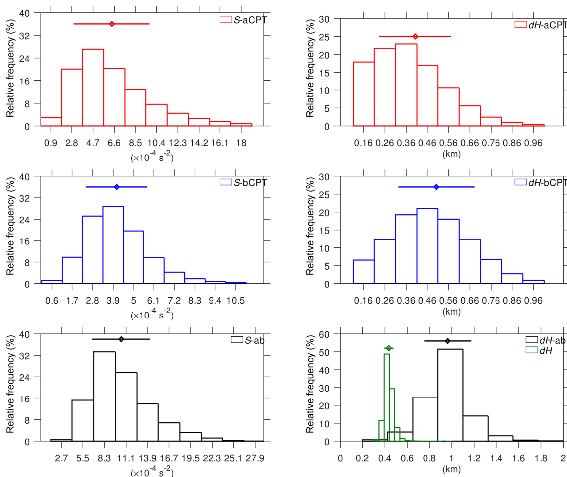
Figure 5. Frequency distribution of TIL parameters with respect to the vertical distance from the CPT. The diamonds and horizontal lines above each histogram represent the mean and standard deviation of each parameter, respectively.
