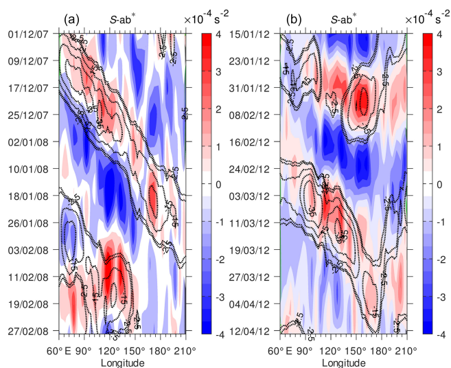
Figure 12. Time–longitude distribution (Hovmöller diagram) of S\text{-}ab^* (color shading) and OLR^* (dotted contours). Color contour interval is 0.25 \times 10^{-4} \text{ s}^{-2} and only negative values of OLR^* are shown for -35 , -25 , -15 , -5 , and -2.5 \text{ W m}^{-2} .
