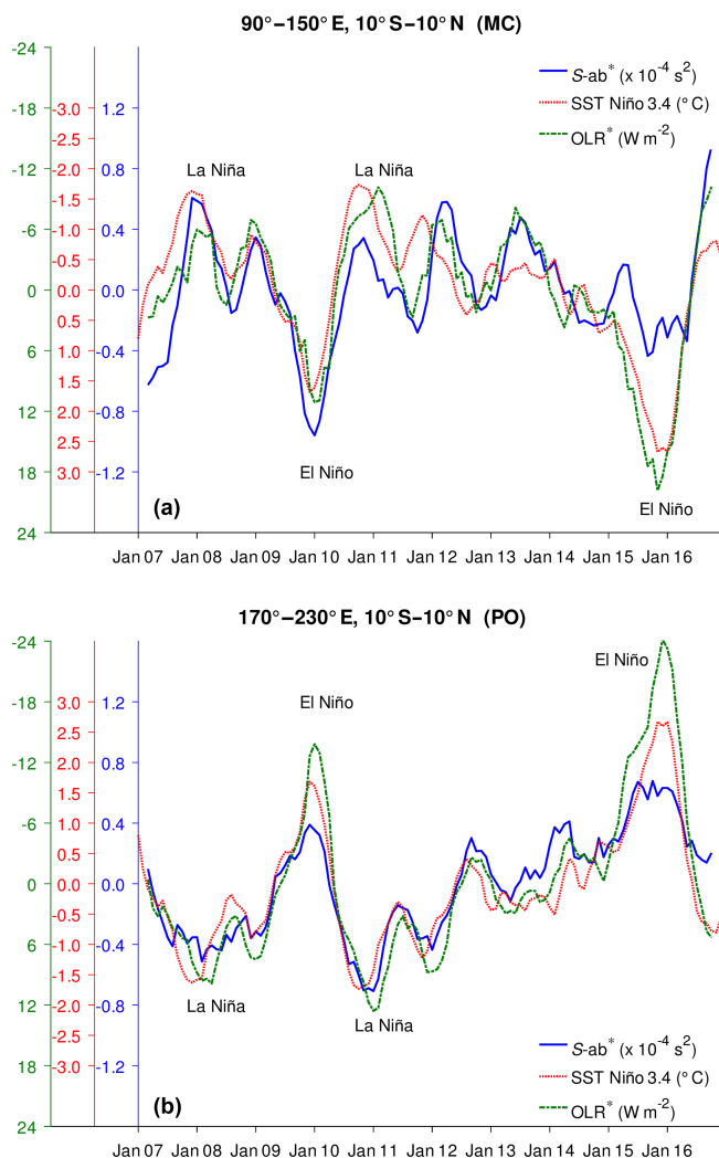
Figure 10. Interannual variations in a S\text{-}ab^* (solid blue line), OLR anomaly (OLR*) (dashed-dotted green line), and SST Niño 3.4 index (dotted red line) for the MC (a) and PO (b). Note that the ordinate axes of both OLR* and SST Niño 3.4 index are reversed in panel (a), but only the ordinate axis of OLR* is reversed in panel (b).
