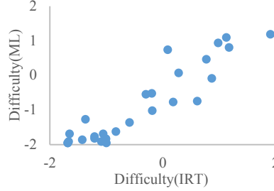
Fig. 2. ML-based difficulty against IRT-based difficulty
