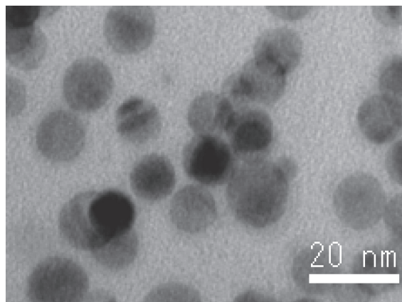
Fig. 3 TEM image of surface of glass after ion-exchange treatment at 753 K for 48 h and hydrogen reduction for 1 h.
