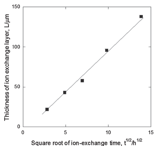
Fig. 2 Relationship between the thickness of the ion exchanged layer of the glass and the square root of the duration of the ion exchange.
