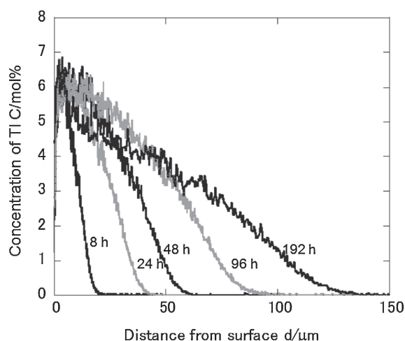
Fig. 1 Concentration profiles of Tl in the glass after ion exchange treatments from 8 to 192 h at 753 K.
