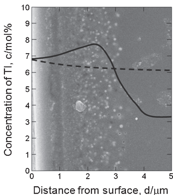
Fig. 5 Cross-sectional SEM image of the glass after hydrogen reduction and concentration profile of the Tl in the glass subjected to ion exchange for 48 h at 753 K: dotted line before and solid line after the hydrogen reduction of the glass.
