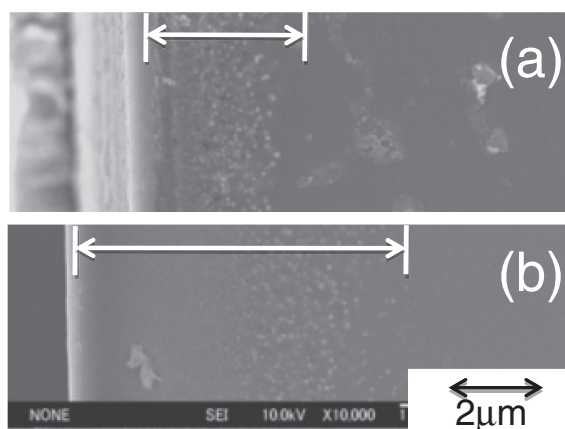
Fig. 4 Cross sectional SEM images of the surface regions of the glass after ion exchange treatment for 48 h and (a): hydrogen reduction for 1 h; (b): hydrogen reduction for 5 h.
