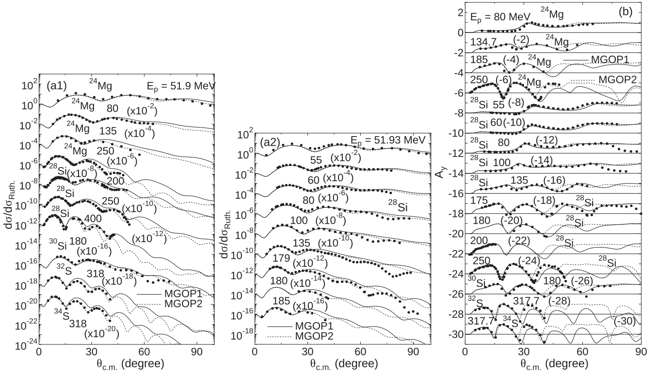
FIG. 19. (a) Elastic-scattering cross sections of p + ^{24}\text{Mg} , ^{28}\text{Si} , ^{30}\text{Si} , ^{32}\text{S} , and ^{34}\text{S} systems at E_p = 51.9 –400 MeV in the Rutherford ratio and (b) analyzing power of p + ^{24}\text{Mg} , ^{28}\text{Si} , ^{30}\text{Si} , ^{32}\text{S} , and ^{34}\text{S} systems at E_p = 55 –317.7 MeV. The experimental data are taken from Refs. [74,112,137,157–166].
