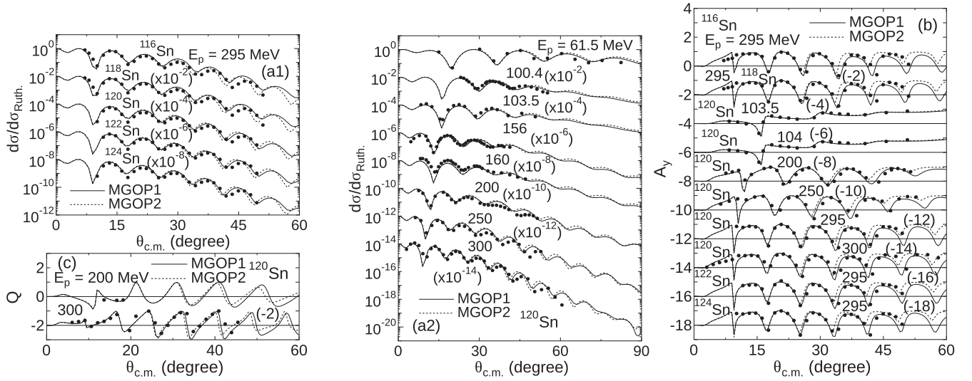
FIG. 24. (a) Elastic-scattering cross sections in the Rutherford ratio at E_p = 61.5 – 300 MeV; (b) analyzing power at E_p = 103.5 – 300 MeV of p + {}^{116}\text{Sn} , {}^{118}\text{Sn} , {}^{120}\text{Sn} , {}^{122}\text{Sn} , and {}^{124}\text{Sn} systems; and (c) Spin-rotation function Q at E_p = 200 and 300 MeV of p + {}^{120}\text{Sn} system. The experimental data are taken from Refs. [74,134,135,159,168,178,186,191,195].
