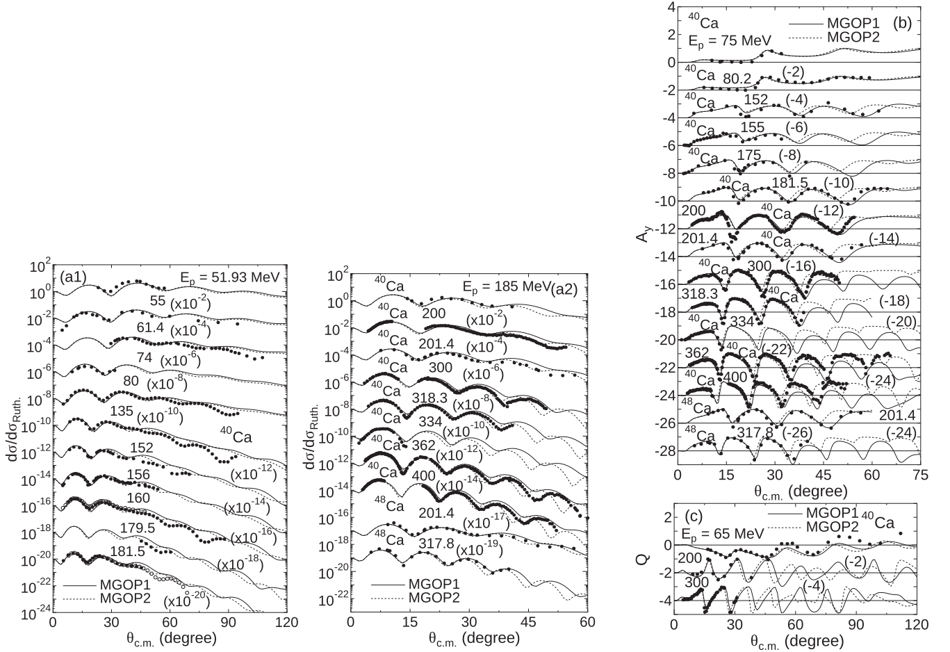
FIG. 20. (a) Elastic-scattering cross sections of p + {}^{40}\text{Ca} and {}^{48}\text{Ca} systems at E_p = 51.93 –400 MeV in the Rutherford ratio; (b) analyzing power of p + {}^{40}\text{Ca} and {}^{48}\text{Ca} systems at E_p = 75 –400 MeV; and (c) spin-rotation function Q of p + {}^{40}\text{Ca} system at E_p = 65 –300 MeV. The experimental data are taken from Refs. [4,32,33,74,124,125,127,132,133,135,137,155,159,166–173].
