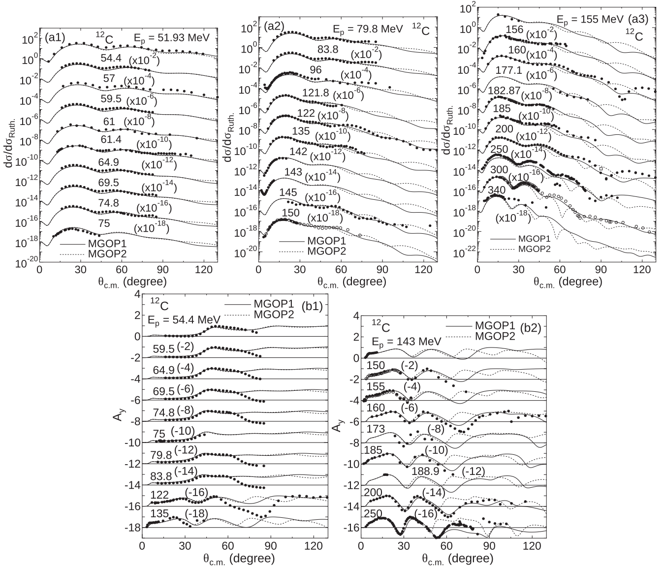
FIG. 17. (a) Elastic-scattering cross sections in the Rutherford ratio at E_p = 51.93 – 340 MeV and (b) analyzing power at E_p = 54.4 – 250 MeV of p + {}^{12}\text{C} system. The experimental data are taken from Refs. [74,121–149].
