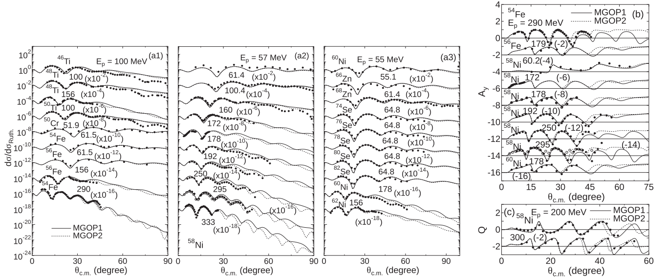
FIG. 21. (a) Elastic-scattering cross sections of p + {}^{46}\text{Ti} , {}^{48}\text{Ti} , {}^{50}\text{Ti} , {}^{50}\text{Cr} , {}^{54}\text{Fe} , {}^{56}\text{Fe} , {}^{58}\text{Ni} , {}^{60}\text{Ni} , {}^{62}\text{Ni} , {}^{66}\text{Zn} , {}^{68}\text{Zn} , {}^{74}\text{Se} , {}^{76}\text{Se} , {}^{78}\text{Se} , {}^{80}\text{Se} , and {}^{82}\text{Se} systems at E_p = 51.9 –333 MeV in the Rutherford ratio; (b) analyzing power of p + {}^{54}\text{Fe} , {}^{56}\text{Fe} , {}^{58}\text{Ni} , and {}^{60}\text{Ni} systems at E_p = 60.2 –295 MeV; and (c) spin-rotation function Q of p + {}^{58}\text{Ni} at E_p = 200 and 300 MeV. The experimental data are taken from Refs. [74,129,133–135,137,168,173–188].
