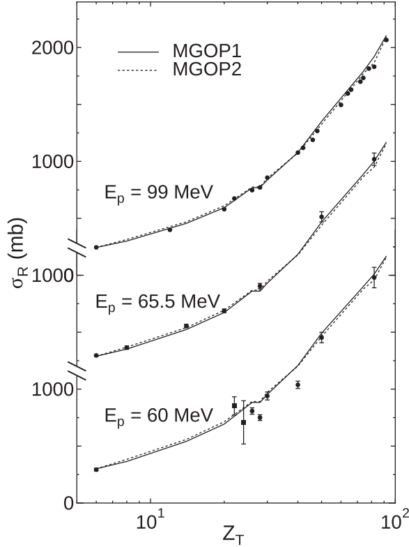
FIG. 7. Total reaction cross sections at E_p = 60 , 65.5 , and 99 MeV as a function of the proton number of a target nucleus Z_T calculated with the MGOP1 and MGOP2 models. See text for more details. The experimental data are taken from Refs. [74,81,82,84].
