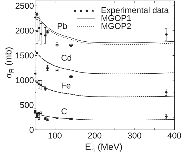
FIG. 9. Total reaction cross sections of n + {}^{12}\text{C} , {}^{56}\text{Fe} , {}^{114}\text{Cd} , and {}^{208}\text{Pb} systems as a function of incident neutron energy E_n calculated with the MGOP1 and MGOP2 models. Experimental data for {}^{\text{Nat.}}\text{C} , {}^{\text{Nat.}}\text{Fe} , {}^{\text{Nat.}}\text{Cd} (natural cadmium), and {}^{\text{Nat.}}\text{Pb} targets are taken from Refs. [74,86–90].
