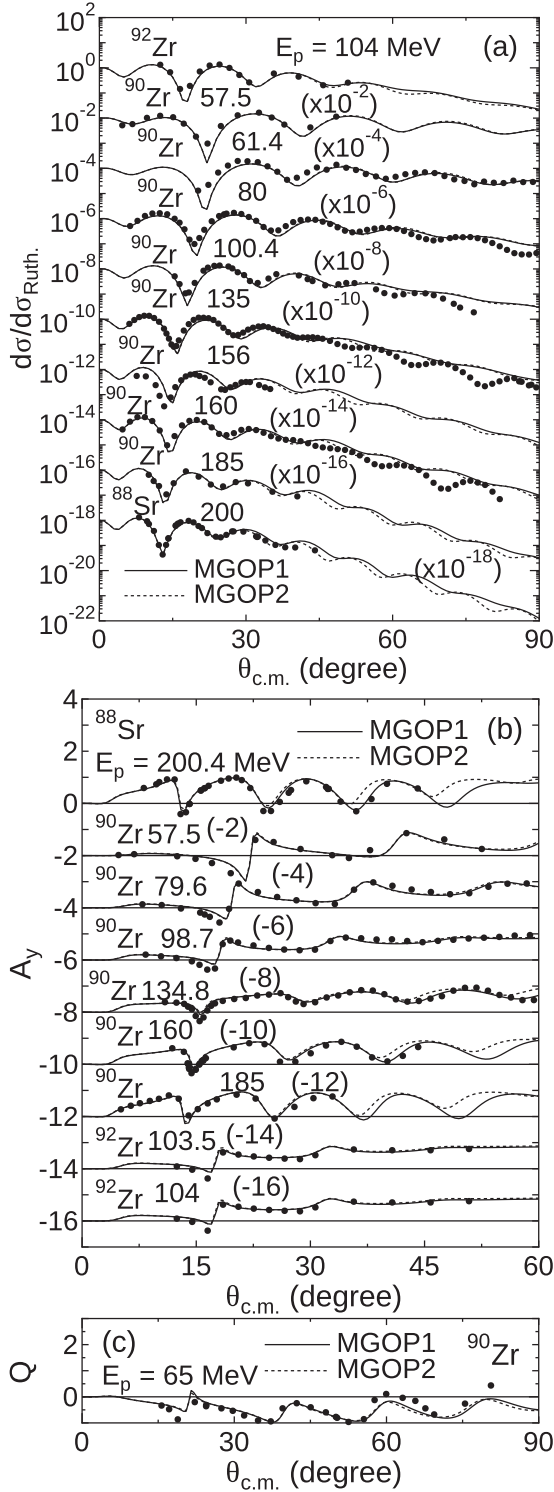
FIG. 22. (a) Elastic-scattering cross sections in the Rutherford ratio at E_p = 57.5 – 200 MeV; (b) analyzing power at E_p = 57.5 – 200.4 MeV of p + ^{88}\text{Sr} , ^{90}\text{Zr} , and ^{92}\text{Zr} systems; and (c) Spin-rotation function Q at E_p = 65 MeV of p + ^{90}\text{Zr} system. The experimental data are taken from Refs. [4,32,74,133,135,159,178,189–192].
