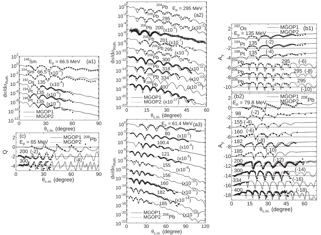
FIG. 25. (a) Elastic-scattering cross sections of p + {}^{148}\text{Sm} , {}^{154}\text{Sm} , {}^{192}\text{Os} , {}^{194}\text{Pt} , {}^{198}\text{Pt} , {}^{204}\text{Pb} , {}^{206}\text{Pb} , and {}^{208}\text{Pb} systems in the Rutherford ratio at E_p = 61.4 – 400 MeV; (b) analyzing power of p + {}^{192}\text{Os} , {}^{194}\text{Pt} , {}^{198}\text{Pt} , {}^{204}\text{Pb} , {}^{206}\text{Pb} , and {}^{208}\text{Pb} systems at E_p = 79.8 – 400 MeV; and (c) spin-rotation function Q of p + {}^{208}\text{Pb} system at E_p = 65 – 300 MeV. The experimental data are taken from Refs. [4,32,33,74,133,135,159,168,172,178,183,188,196–205].
