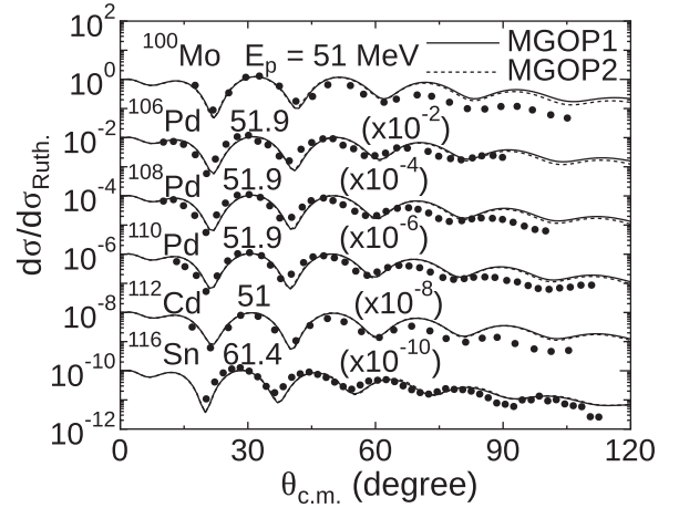
FIG. 23. Elastic-scattering cross sections of p + ^{106}\text{Pd} , ^{108}\text{Pd} , ^{110}\text{Pd} , ^{112}\text{Cd} , and ^{116}\text{Sn} systems in the Rutherford ratio at E_p = 51 – 61.4 MeV. The experimental data are taken from Refs. [74,133,193,194].
