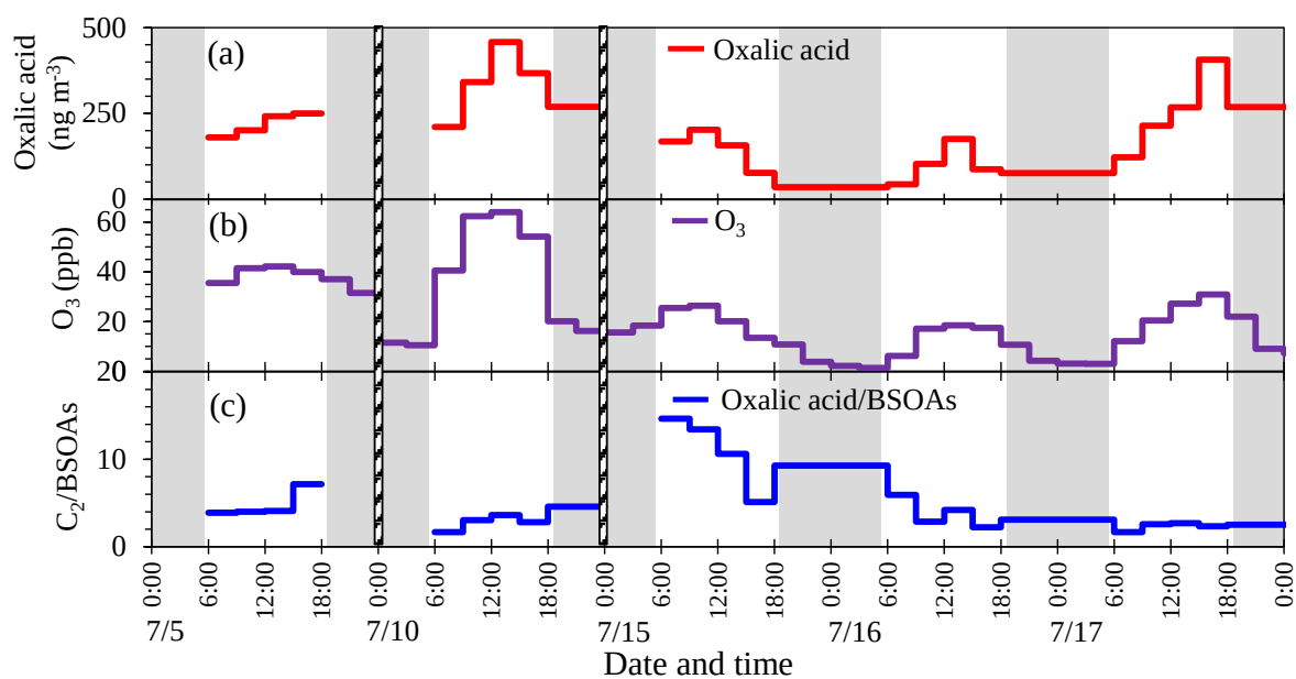
Fig. 2. Diurnal and temporal variations in the concentrations of (a) oxalic acid and (b) O_3 , and (c) mass concentration ratios of oxalic acid/BSOAs in a L. kaempferi forest. Shaded areas indicate nighttime.
