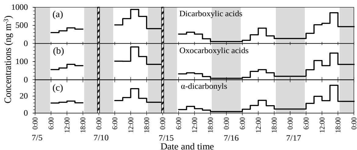
Fig. 1. Diurnal and temporal variations in the concentrations of (a) total dicarboxylic acids, (b) oxocarboxylic acids, and (c) \alpha -dicarbonyls in a L. kaempferi forest. Shaded areas indicate nighttime.
