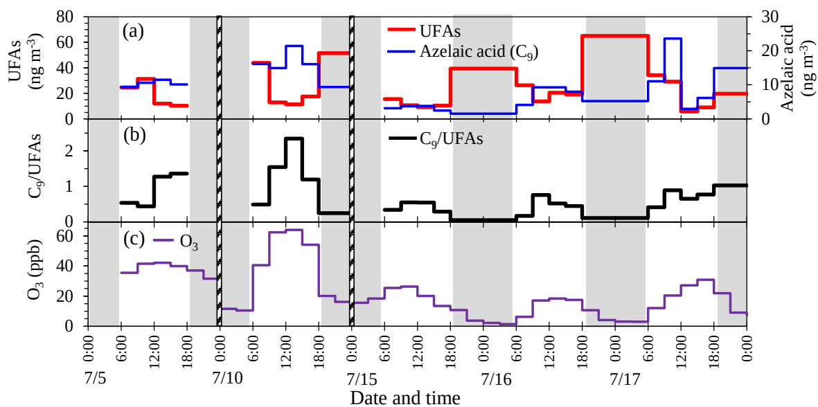
Fig. 5. Diurnal and temporal variations in (a) concentrations of unsaturated fatty acids (UFAs: oleic plus linoleic acids) and azelaic acid (C 9 ), (b) mass concentration ratios of azelaic acid/UFAs (C 9 /UFAs), and O 3 concentrations in a L. kaempferi forest. Shaded areas indicate nighttime.
