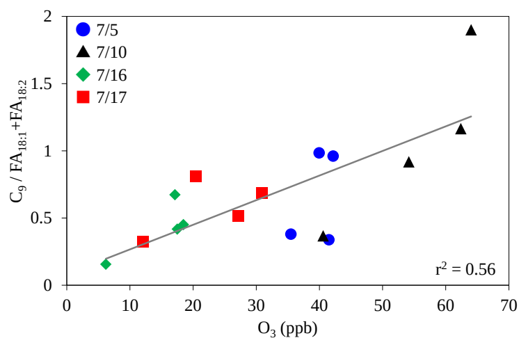
Fig. 6. Correlation plots of concentration ratios of azelaic acid (C 9 ) to oleic plus linoleic acids (C 9 /(FA 18:1 +FA 18:2 )) as a function of O 3 .
