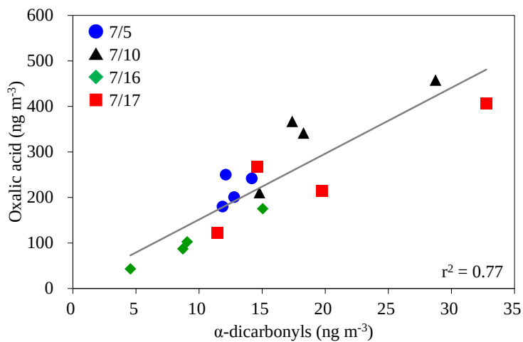
Fig. 3. Correlation plot of oxalic acid and \alpha -dicarbonyls.
