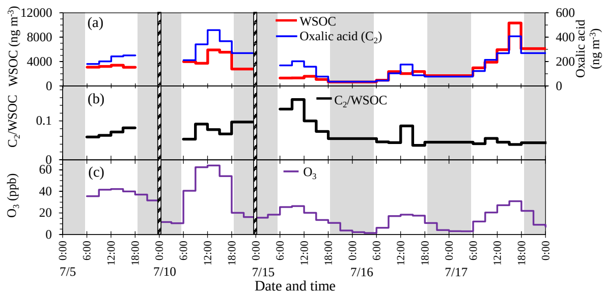
Fig. 7. Diurnal and temporal variations in (a) concentrations of water-soluble organic carbon (WSOC) and oxalic acid, (b) mass concentration ratios of oxalic acid to WSOC ( C_2/WSOC ) and (c) O_3 concentrations in a L. kaempferi forest. Shaded areas indicate nighttime.
