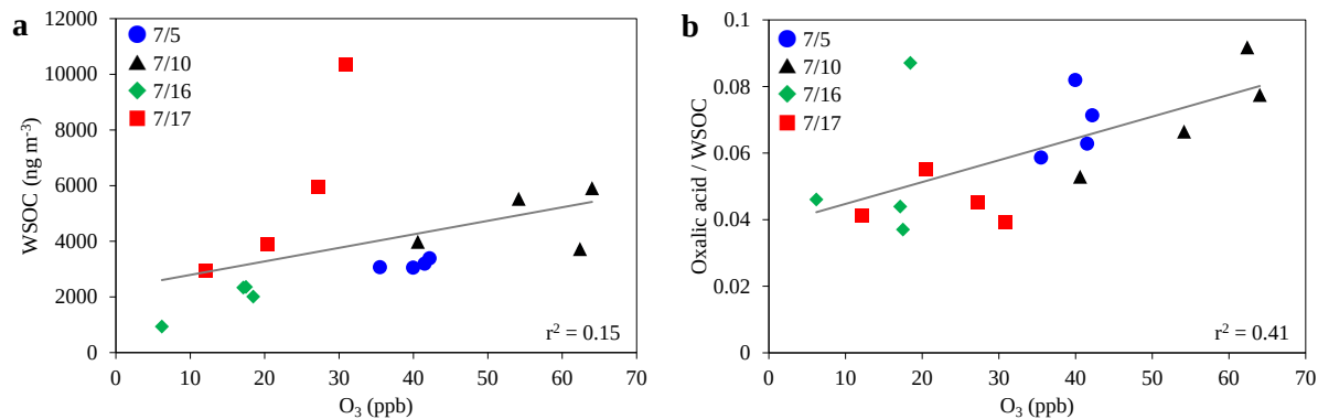
Fig. 8. Correlation plots of (a) water soluble organic carbon (WSOC) and (b) mass concentration ratios of oxalic acid to WSOC ( C_2/WSOC ) as a function of O_3 .
