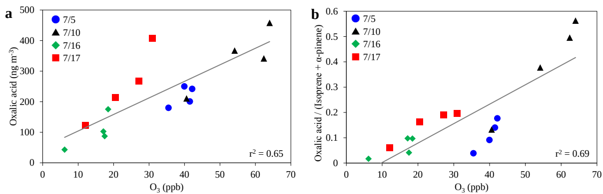
Fig. 4. Correlation plots of (a) oxalic acid with O 3 and (b) mass concentration ratio of oxalic acid to isoprene plus α-pinene (oxalic acid/(isoprene+α-pinene)) with O 3 .
