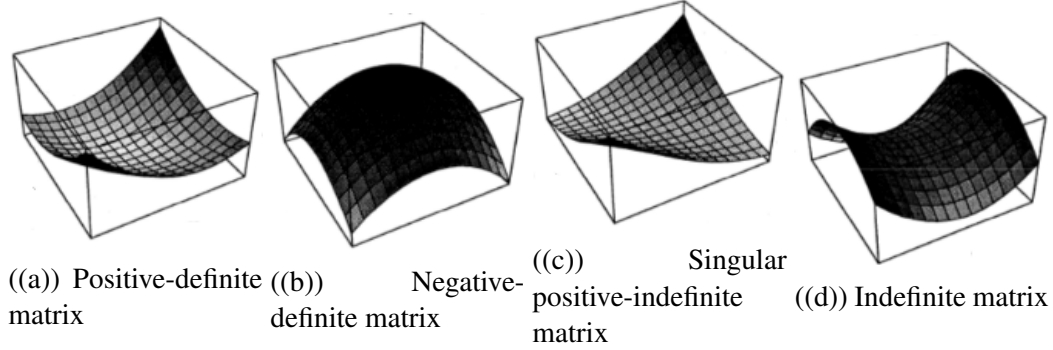
Figure 2.5: Graphic representation of matrix definitiveness
