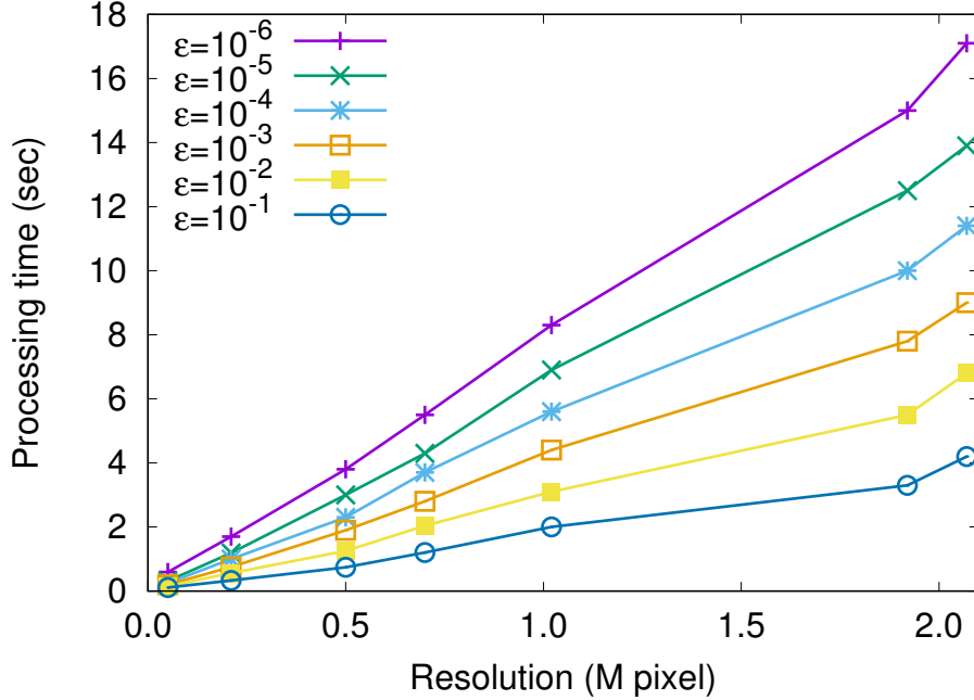
Figure 2.13: Result of conjugate gradient method (CG). Resolution vs time.
