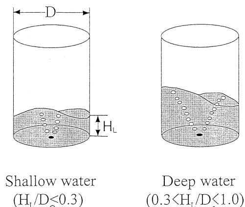
Fig. 1. Classification of swirl motions of a bath agitated by bottom gas injection.
