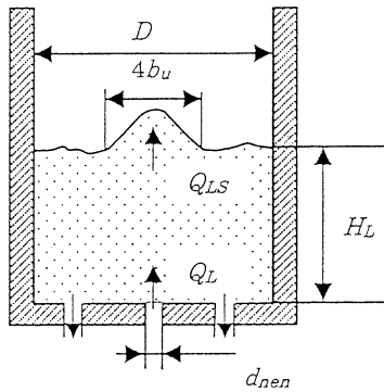
Fig. 5. Elevated surface of a bath agitated by bottom liquid injection.
