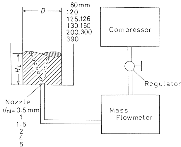
Fig. 2. Experimental apparatus.
