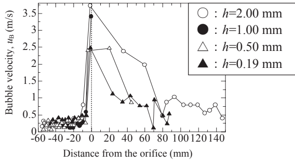
Fig. 16 Bubble velocity for four channel heights ( \beta=0.04 , L_o=5 mm, j_a=0.14 m/s, and j_w=0.14 m/s)
