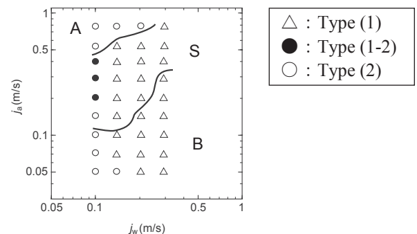
Fig. 10 Flow pattern map for h=2.00 mm, \beta=0.2 , and L_o=5 mm
