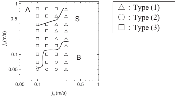
Fig. 11 Flow pattern map for h=2.00 mm, \beta=0.4 , and L_o=5 mm
