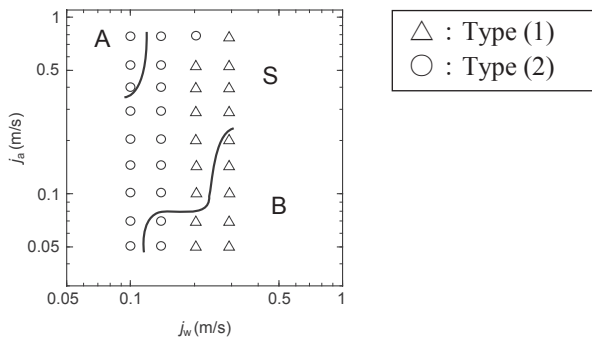
Fig. 6 Flow pattern map for h=1.00 mm, \beta=0.04 , and L_o=5 mm
