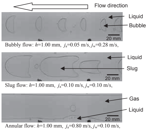
Fig. 3 Photographs of basic three flow patterns observed in the test section
