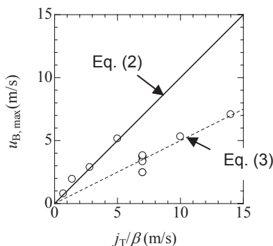
Fig. 18 Relationship between maximum bubble velocity, u_{B,max} , and j_T/\beta
