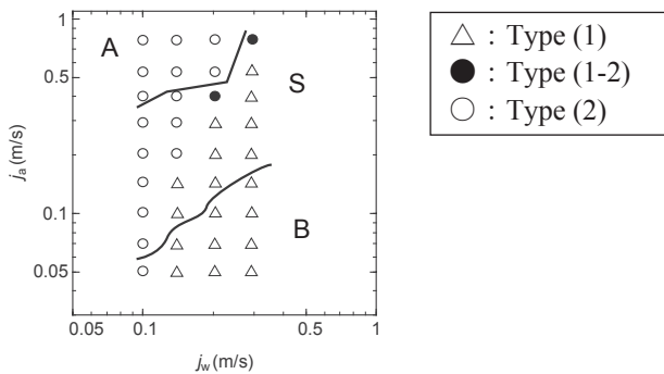
Fig. 5 Flow pattern map for h=2.00 mm, \beta=0.04 , and L_o=5 mm
