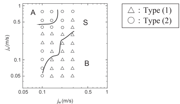
Fig. 9 Flow pattern map for h=2.00 mm, \beta=0.1 , and L_o=5 mm
