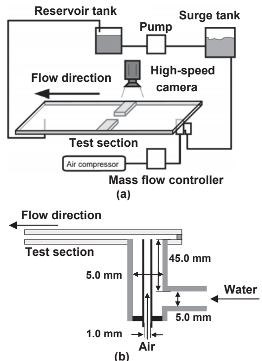
Fig. 1 Schematic diagram of experimental apparatus (a) and the details of air and water inlet (b)
