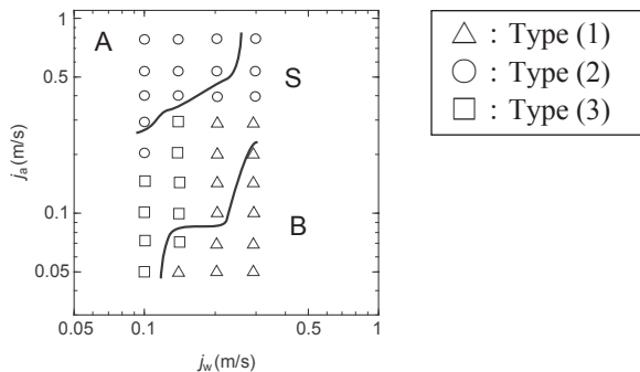
Fig. 12 Flow pattern map for h=2.00 mm, \beta=0.04 , and L_o=10 mm
