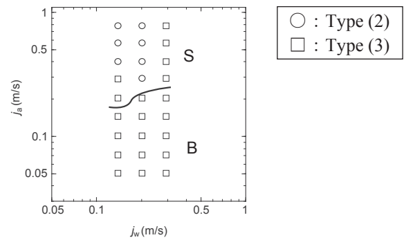
Fig. 8 Flow pattern map for h=0.19 mm, \beta=0.04 , and L_o=5 mm
