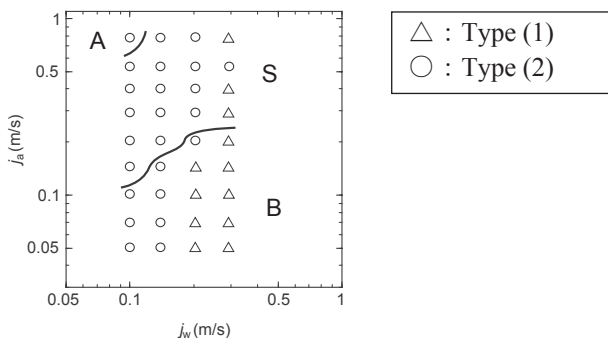
Fig. 7 Flow pattern map for h=0.50 mm, \beta=0.04 , and L_o=5 mm
