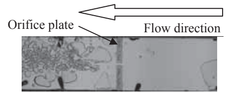
Type (1): h=2.00 mm, j_a=0.20 m/s, j_w=0.20 m/s, \beta=0.04 , L_o=5 mm
