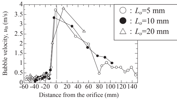
Fig. 17 Bubble velocity for three orifice thicknesses ( h=2.00 mm, \beta=0.04 , j_a=0.14 m/s, and j_w=0.14 m/s)
