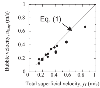
Fig. 14 Relationship between bubble velocity and the total superficial velocity
