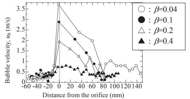
Fig. 15 Bubble velocity for four contraction ratios ( h=2.00 mm, L_o=5 mm, j_a=0.14 m/s, and j_w=0.14 m/s)
