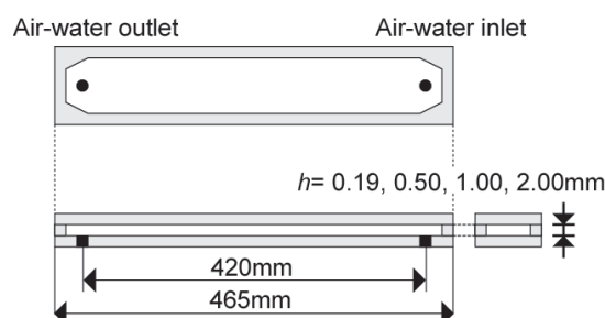
Fig. 2 Details of test section
