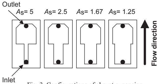
Fig. 3 Configurations of abrupt expansion
