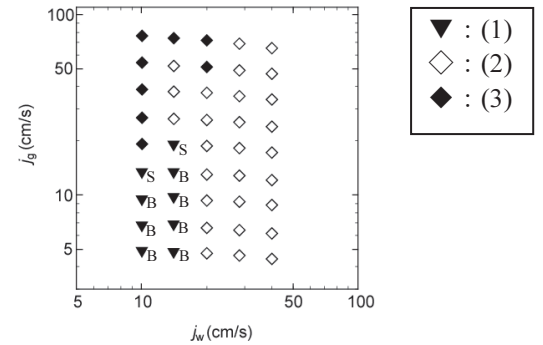
Fig. 10 Flow pattern map for h=2.00 mm and A_s=5 (B and S denote bubbly and slug flows, respectively)
