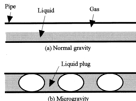
Fig.1 Liquid plug.
