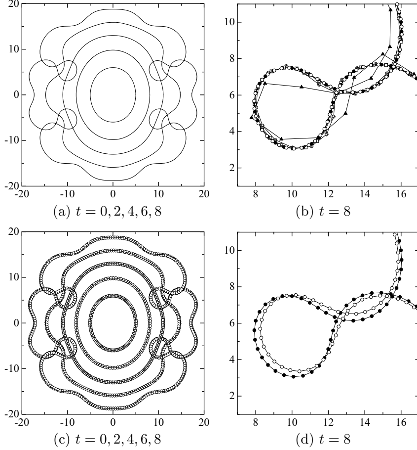
Figure 2: The time step starts from \Delta t_0 = 10^{-4} . (a) Evolution of curve computed with N = 400 . (b) An enlarged view. N = 100(\blacktriangle) , 200(\odot) , 300(\square) , 400(\bullet) , 500(\circ) . (c) Solid line: N fixed, \circ : N increased. (d) \bullet : N fixed, \circ : N increased.
