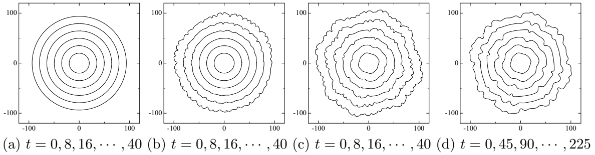
Figure 3: The time step starts from \Delta t_0 = 10^{-3} . Number of points increase from N = 256 to N = 1024 . (a),(b) Parameters: \alpha_{\text{eff}} = 3 , V^{(0)} = 1.8 , \delta = 4 . Initial curve: (a) circle ( \mathbf{X} = 20\mathbf{N} ) (b) circle ( \mathbf{X} = 20\mathbf{N} ) with 5% noise. (c),(d) Initial curve: a round square ( \mathbf{X} = R(u)\mathbf{N} , R(u) = 20(1 + 0.04\sin(4\pi u) + 0.02\sin(16\pi u)) ) with 5% noise. Parameters: \delta = 4 , (c) \alpha_{\text{eff}} = 3 , V^{(0)} = 1.8 (d) \alpha_{\text{eff}} = 1.7 , V^{(0)} = 0.3 .
