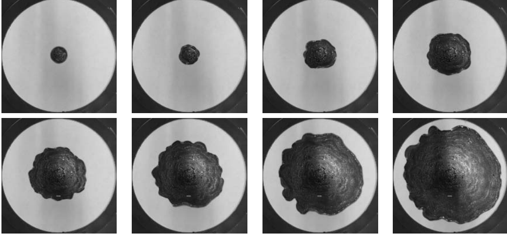
Figure 5: The photographs depict snapshots from an experimental movie of spreading flame/smoldering front along a sheet of paper placed near the floor at 200th, 400th, 1000th, 1600th, ..., 4000th frames at the rate of 30 fps. Experiments were performed by the same method as [5].
