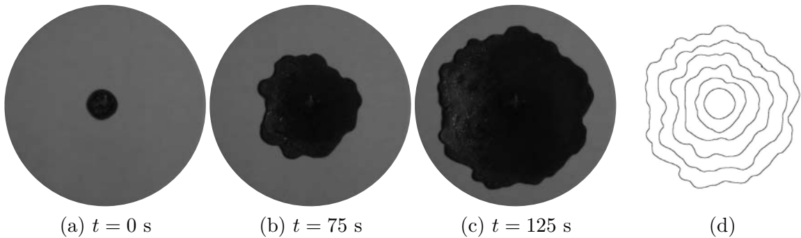
Figure 4: The formation of corrugated reaction fronts owing to inherent instability of smoldering combustion. (a),(b),(c) Experimental images of combustion of a filter paper at each time; (d) Evolution of smoldering front segmented from experimental images at t = 0, 25, 50, \dots, 125 s by the free software ImageJ.
