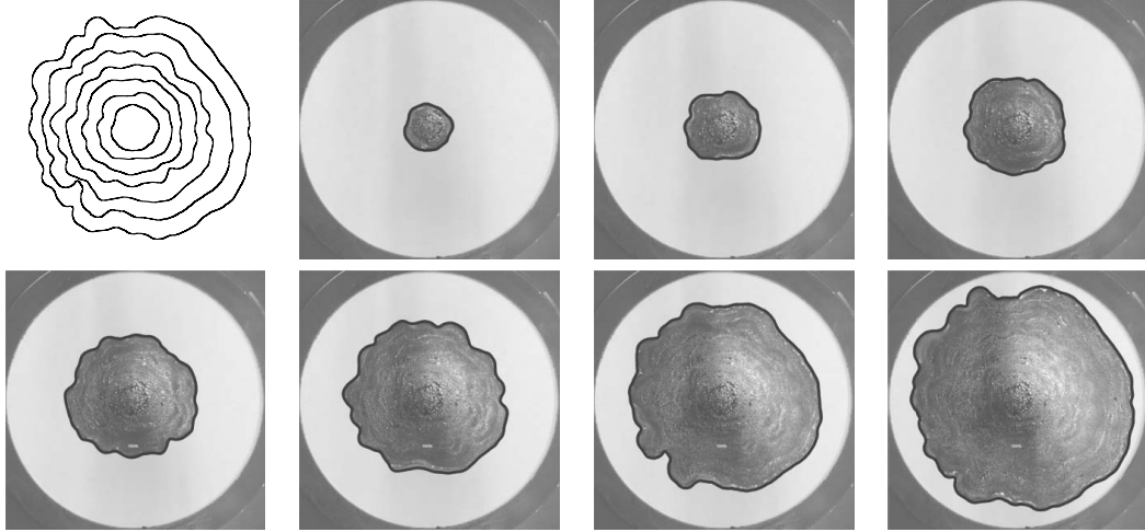
Figure 6: The upper-left figure depicts selected segmentation curves at frames: 400, 1000, 1600, 2200, 2800, 3400, 4000, summarizing the front evolution in the other photographs from left to right, upper to lower. The blue curve in each photograph is a segmentation curve, and the background vague region is the same as that in Figure 5.
