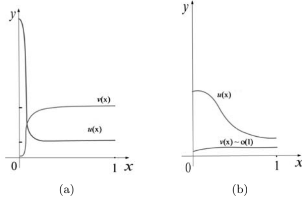
Figure 3: (a): large spiky steady state for small d_2 , large enough \rho_{12} and \rho_{12}/d_1 , (b): positive steady state with singular bifurcation structure when d_2 is near a_2/\pi^2 , \rho_{12} and \rho_{12}/d_1 are large enough.
