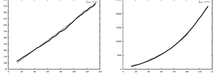
Figure 7: (Left) The total length of front \tilde{L} [mm] vs. the actual time [second]. (Right) The enclosed area \tilde{A} [mm 2 ] vs. the actual time [second]. Blue points indicate the actual values and red curves are the graphs of (23) and (24), respectively.
