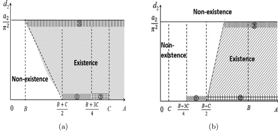
Figure 2: (a): B < C i.e. strong competition; (b): B > C i.e. weak competition.
