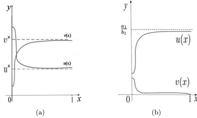
Figure 1: (a): spiky steady state near (u^*, v^*) for small d_2 , large enough \rho_{12} and \rho_{12}/d_1 , (b) spiky steady state near (a_1/b_1, 0) for A > B , when d_2 is small, d_1 and \rho_{12}/d_1 are large enough.
