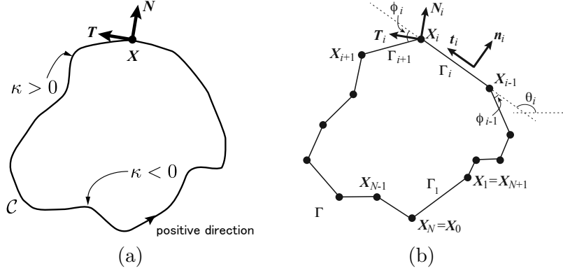
Figure 1: (a) Jordan curve \mathcal{C} (b) Jordan polygonal curve \Gamma
