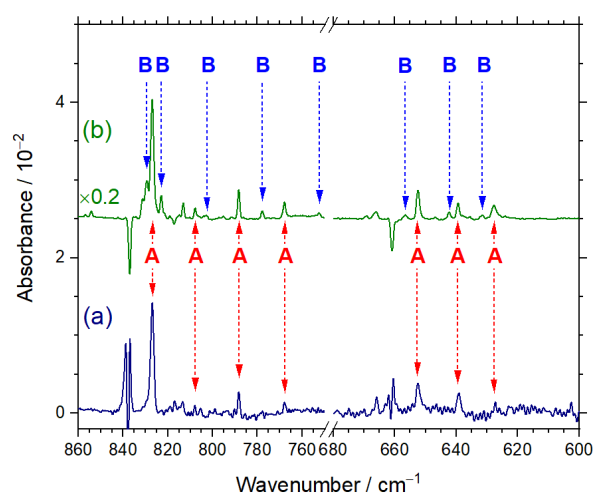
FIG. 4. Comparison of IR spectra in regions 860–750 and 680–600 \text{cm}^{-1} measured for a hydrogen-addition experiment and an electron-bombardment experiment. (a) The IR spectrum of \text{Cl}_2/\text{C}_{20}\text{H}_{10}/p\text{-H}_2 matrix after visible (405 nm) and IR irradiation. (b) The spectrum of the electron-bombarded \text{C}_{20}\text{H}_{10}/p\text{-H}_2 matrix after maintenance in darkness at 3.2 K for 30 h. From both traces, the lines of \text{C}_{20}\text{H}_{10} were stripped. The lines in groups A and B are indicated with red and blue arrows, respectively.
