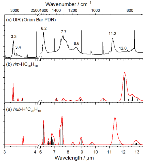
FIG. 6. Comparison of UIR bands with experimental IR spectra of hydrogenated and protonated corannulene in solid p -H 2 . Experimental spectra of (a) hub\text{-H}^+\text{C}_{20}\text{H}_{10} 28 and (b) rim\text{-HC}_{20}\text{H}_{10} ; (c) the UIR emission spectrum from Orion Bar PDR (Ref. 39). Experimental spectra are presented with sticks of which the heights represent integrated intensities. Solid red lines represent spectra convoluted with Gaussian profiles of full-width at half-maximum 30 cm -1 .
