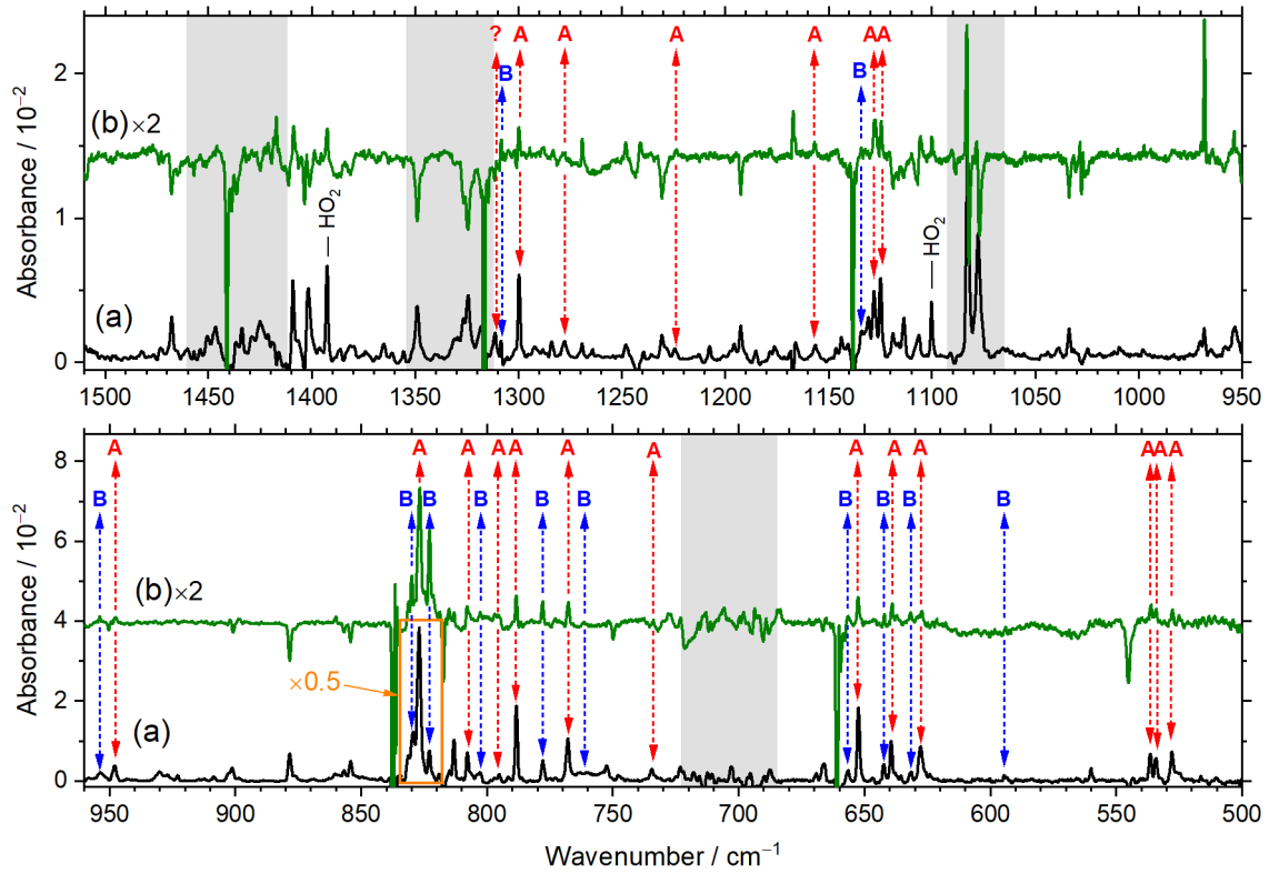
FIG. 3. Infrared spectra of electron-bombardment experiments on C_{20}H_{10}/p\text{-}H_2 in region 1510–500 \text{cm}^{-1} . (a) IR spectrum of the electron-bombarded matrix with lines of C_{20}H_{10} subtracted using an IR spectrum of C_{20}H_{10}/p\text{-}H_2 matrix deposited without electron bombardment; (b) difference spectrum of the electron-bombarded matrix after maintenance in darkness at 3.2 K for 30 h; lines pointing upward indicate production and those pointing downward indicate destruction. The lines in groups A and B are indicated with red and blue arrows, respectively. Tentative assignments are indicated with "?". The lines near 1100 and 1392 \text{cm}^{-1} due to HO_2 , which originated from the hydrogenation of O_2 impurity, are also indicated. Negative lines in trace (b) are due to C_{20}H_{10} or H^+C_{20}H_{10} for which spectral assignments were presented in our previous work. 28 The regions suffering from extensive interference are indicated with grey rectangles.
