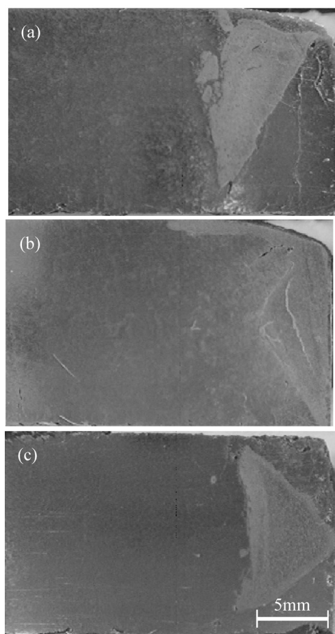
Fig. 4 OM photographs of the AZ91D magnesium alloy based specimens. Particle size of titanium and applied G number are (a) 10\mu\text{m} and 40, (b) 45\mu\text{m} and 40, and (c) 45\mu\text{m} and 120. The direction of centrifugal force is indicated by an arrow.
