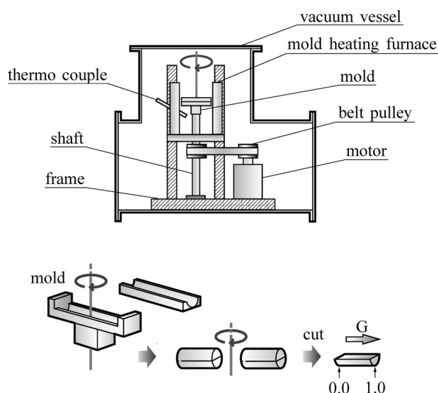
Fig. 2 Apparatuses for the centrifugal solid-particle method performed in this study. The abscissa in this figure is the normalized position, and 0.0 and 1.0 of normalized position are inside and outside surface of peripheral position, respectively.
