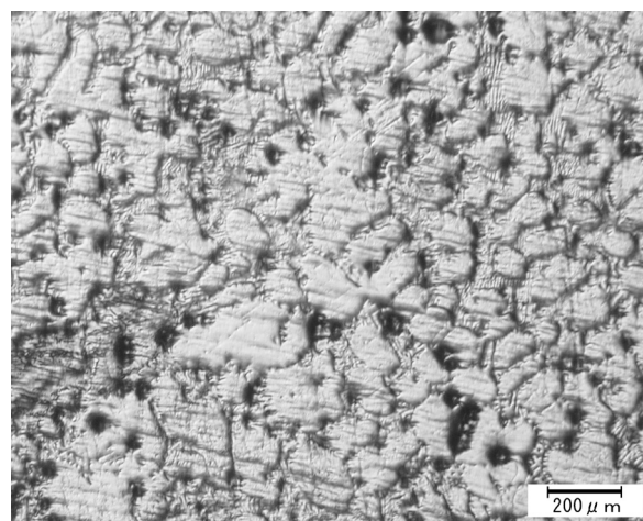
Fig. 7 OM photograph of the pure magnesium-titanium particles specimen.
