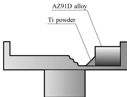
Fig. 3 Setting of the AZ91D magnesium alloy and titanium particles in the mold.
