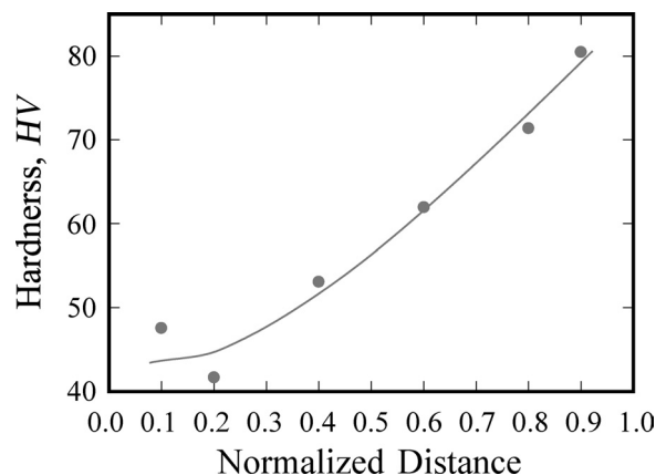
Fig. 11 Vickers hardness distribution of specimen, which were fabricated from the Mg-6 mass%Zn-2 vol%Ti master alloy.
